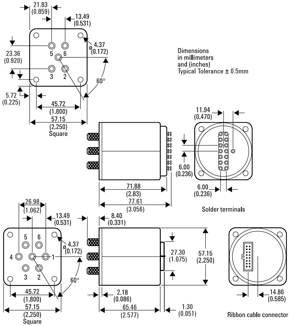
Figure 13. Mechanical dimensions
