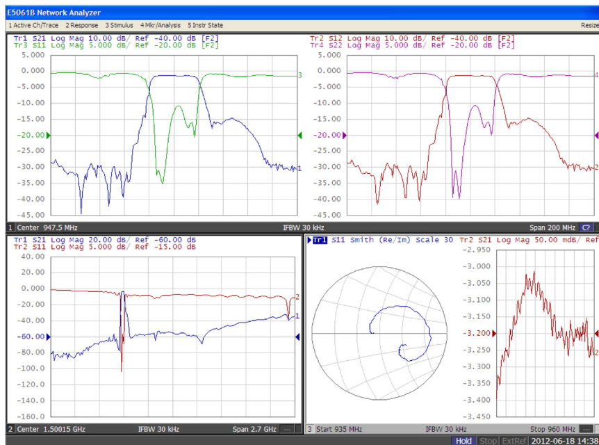
Figure 5. E5061B displaying 3 channel (setting) and 8 traces mode
