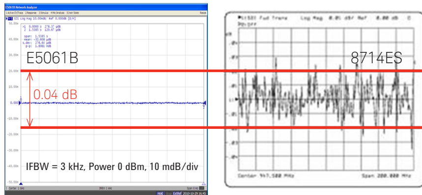
Figure 2. Trace noise comparison at 90 dB dynamic range
