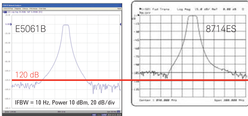
Figure 1. Dynamic range comparison
