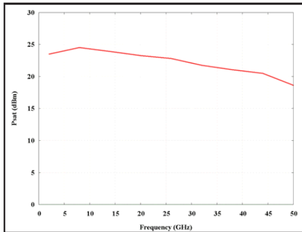
Figure 3-10 Saturated output power (for N4985A-S50)
