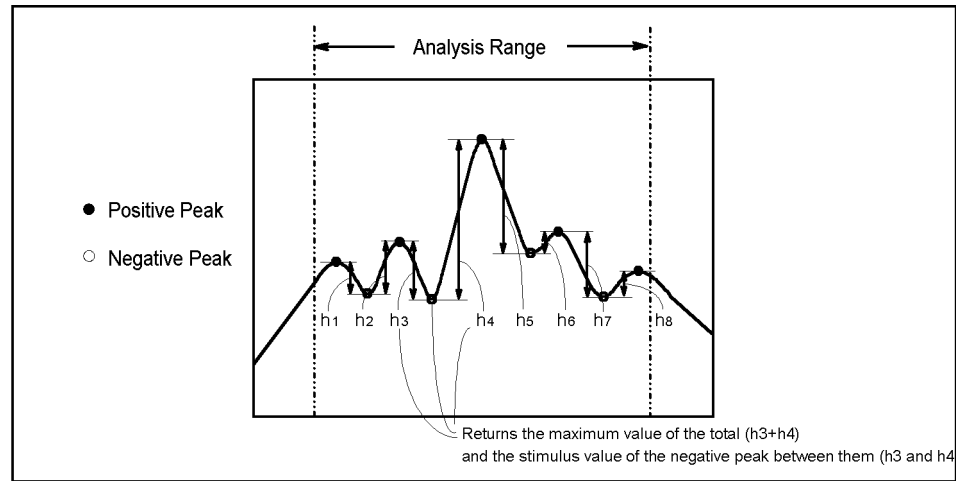
Figure 8-11 MaxRipplePoint
