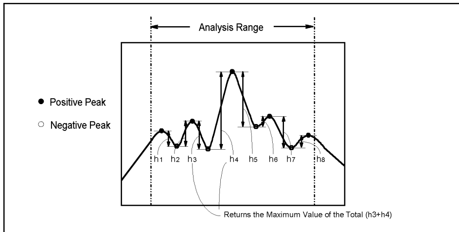
Figure 8-12 MaxRippleValue
