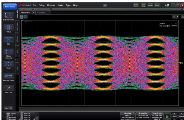
Figure 2. 80 GBaud PAM8 (= 240 Gbps)
