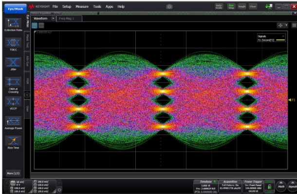
Figure 1. PAM-4, 144 GBaud (= 288 Gbps)
