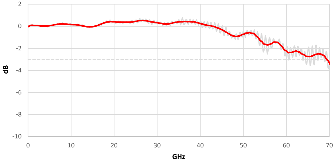
Figure 5. Frequency response at front panel output, measured at sample rate of 128 GSa/s, and 1 V_{pp,diff} amplitude. \text{Sin}(x)/x roll-off mathematically compensated. Red: Savitzky-Golay filters polynomial fit, window size: 5%, grey: measured data.
