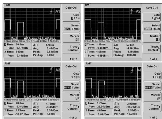
Figure 7. Measurement flexibility with 4 independent time gates
