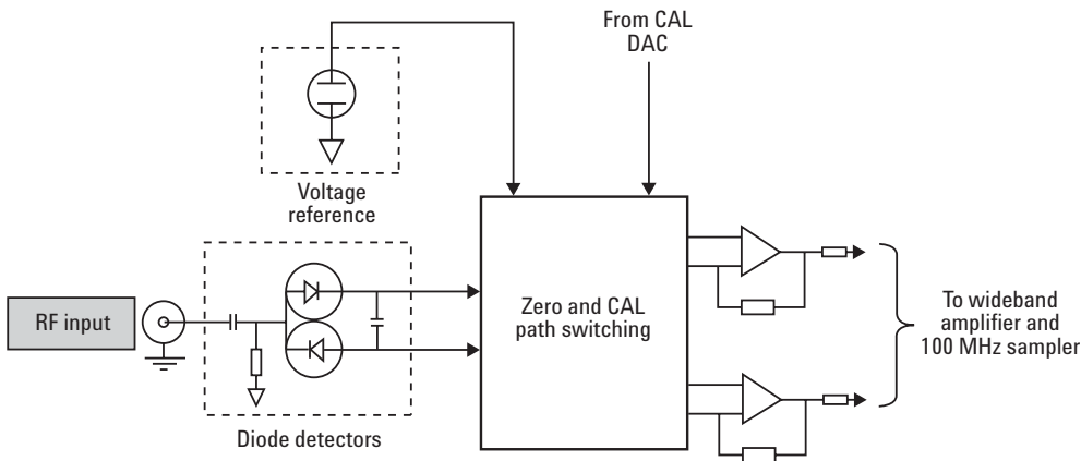
Figure 1. Internal zero and cal block diagram
