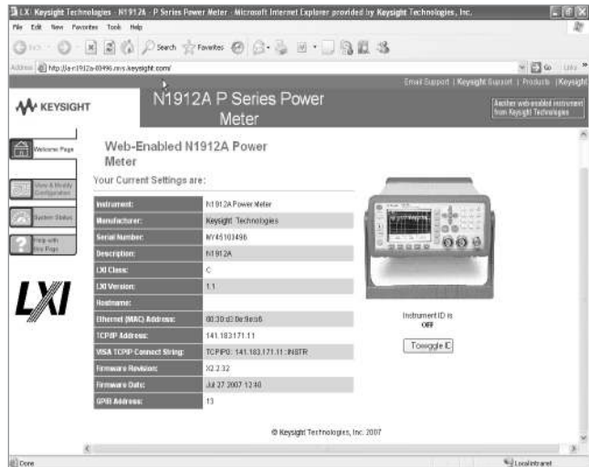
Figure 2. Instrument web page browser that provides instruments setting at a glance and enable remote access/control
