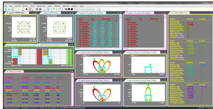
Figure 7. 8-channel TD-LTE beamforming with antenna patterns and EVM measurements per layer. The same measurement is available for LTE-FDD.
