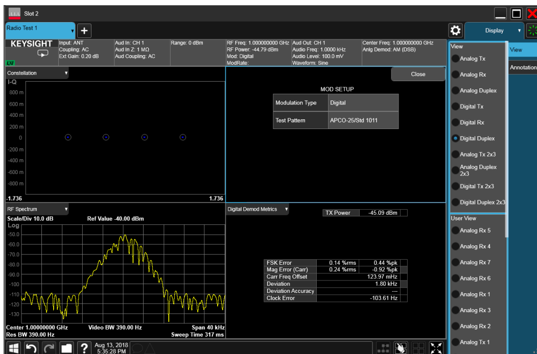
Figure 2. N9093EM1E basic digital test
