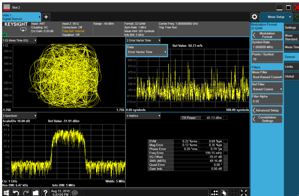
Figure 3. Y9054EM0E general purpose digital radio application
