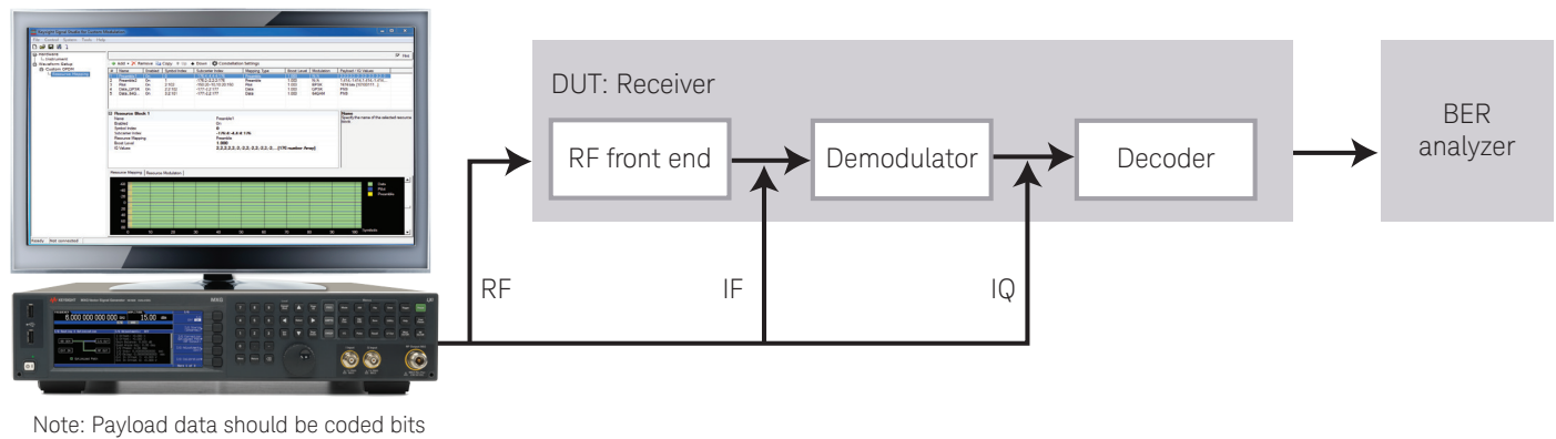
Figure 2. Generate receiver test signals for early testing of your receiver with Keysight X-Series signal generators and Signal Studio Pro.
