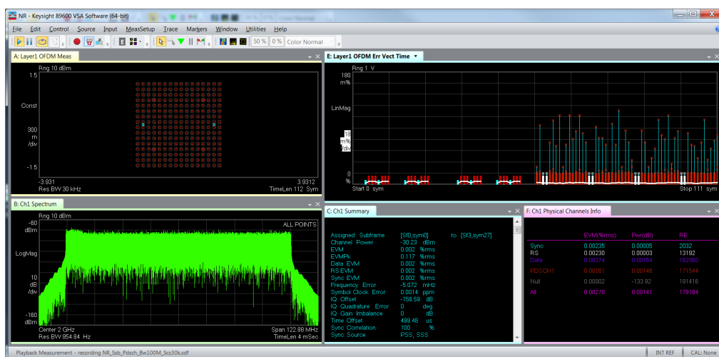
Figure 3. 5G NR single carrier measurement with 89601BHNC.
