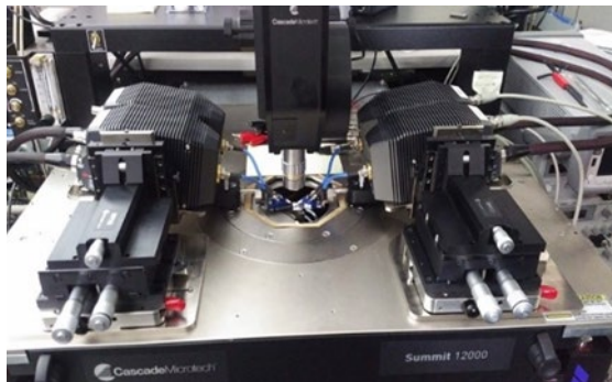
N529xAX Frequency extenders mounted on a Cascade Summit 12K probe station
