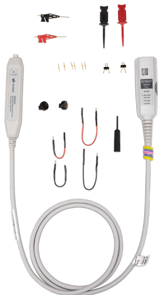
Figure 9. N2819A 800 MHz differential probe with AutoProbe interface
