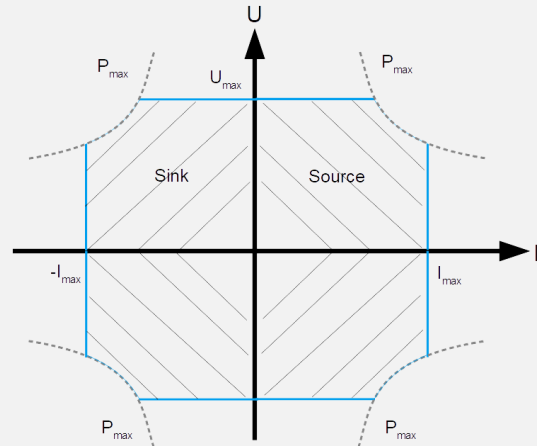
Figure 2. Maximum power of 0 V to U_{max} (4 quadrant system)
