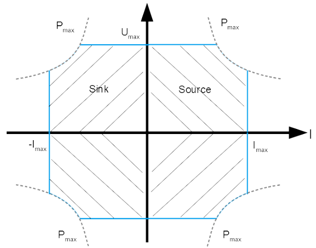
Maximum power of 0\text{ V} - U_{\max} (4 quadrant system)
