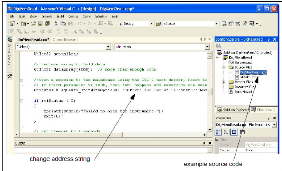
Figure 3-7 Changing the Instrument Address String (IVI-C Programs).
