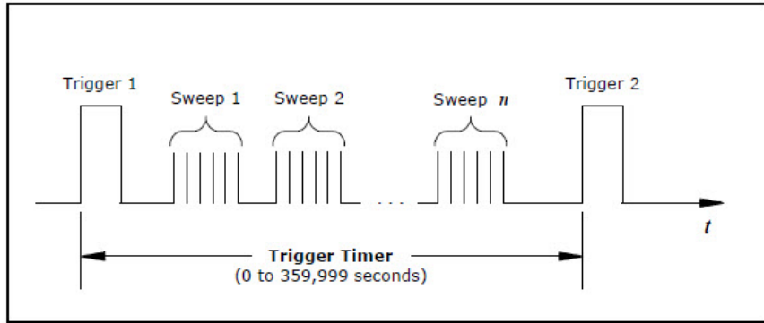
Figure 3-10 Trigger-to-Trigger Interval.
