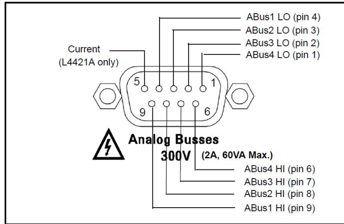
Figure 3-3 L4400 Analog Bus Port Pinouts.
