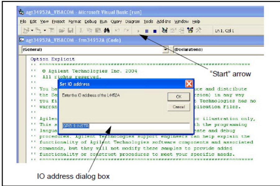
Figure 3-9 Changing the Address String (VISA COM Programs).
