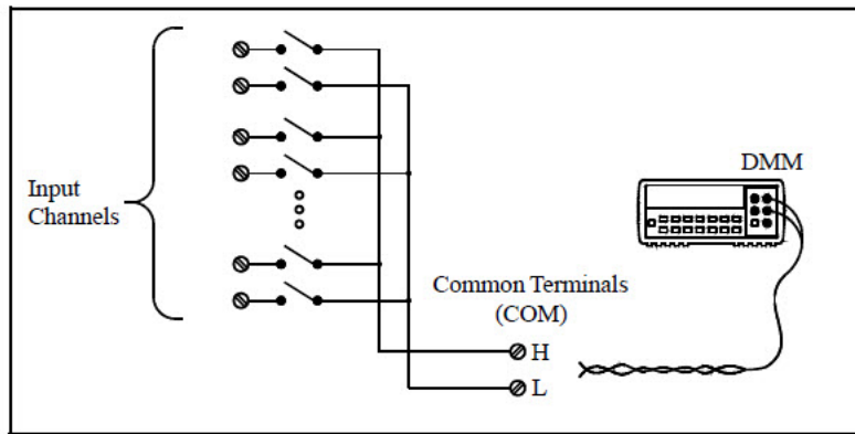
Figure 3-13 Scanning with External Instruments.
