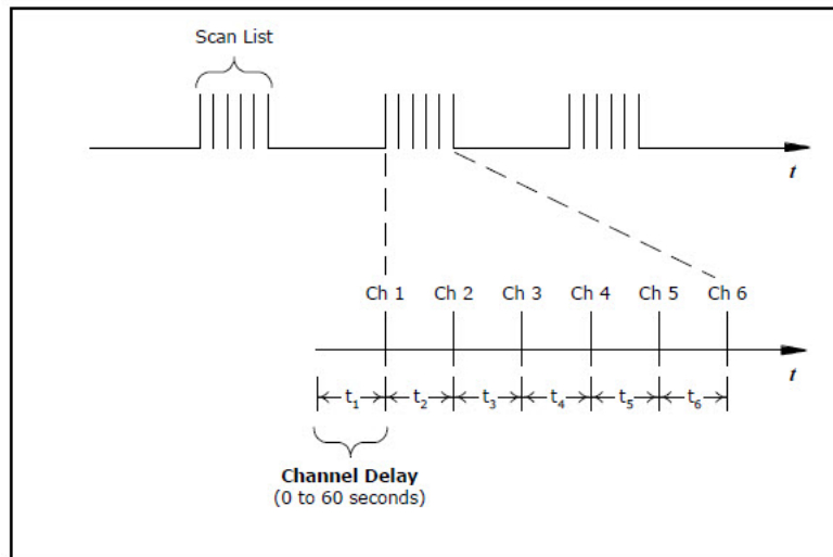
Figure 3-12 Channel Delay.
