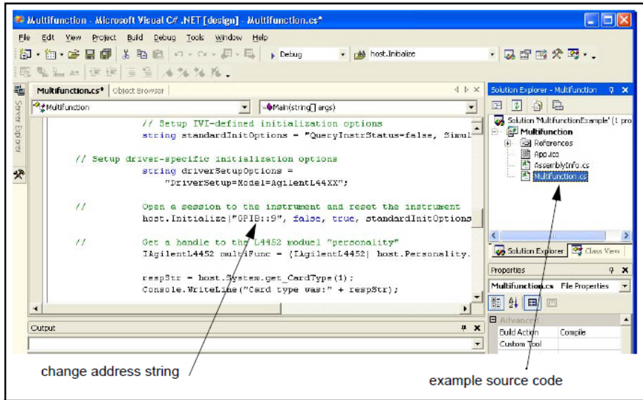
Figure 3-5 Changing the Instrument Address String (IVI-COM Programs).
