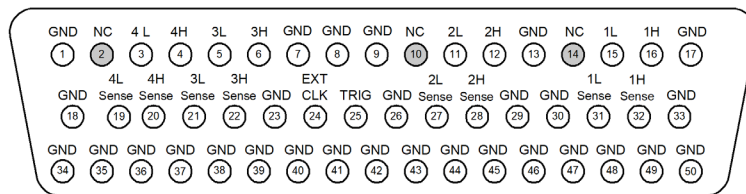
50-Pin D-Sub Female Connector
