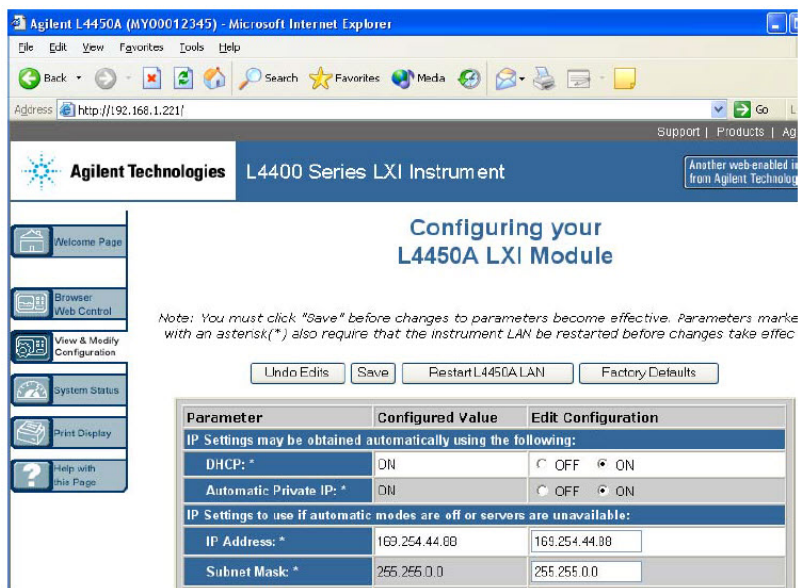
Figure 2-8 Changing the Instrument LAN Interface Configuration.
