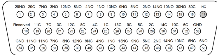
50-Pin D-Sub Male Connector
