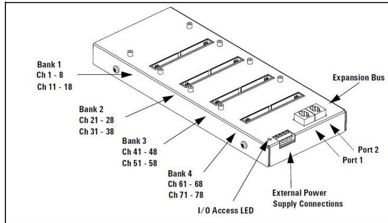
Figure 7-2 The 34945EXT Module.
