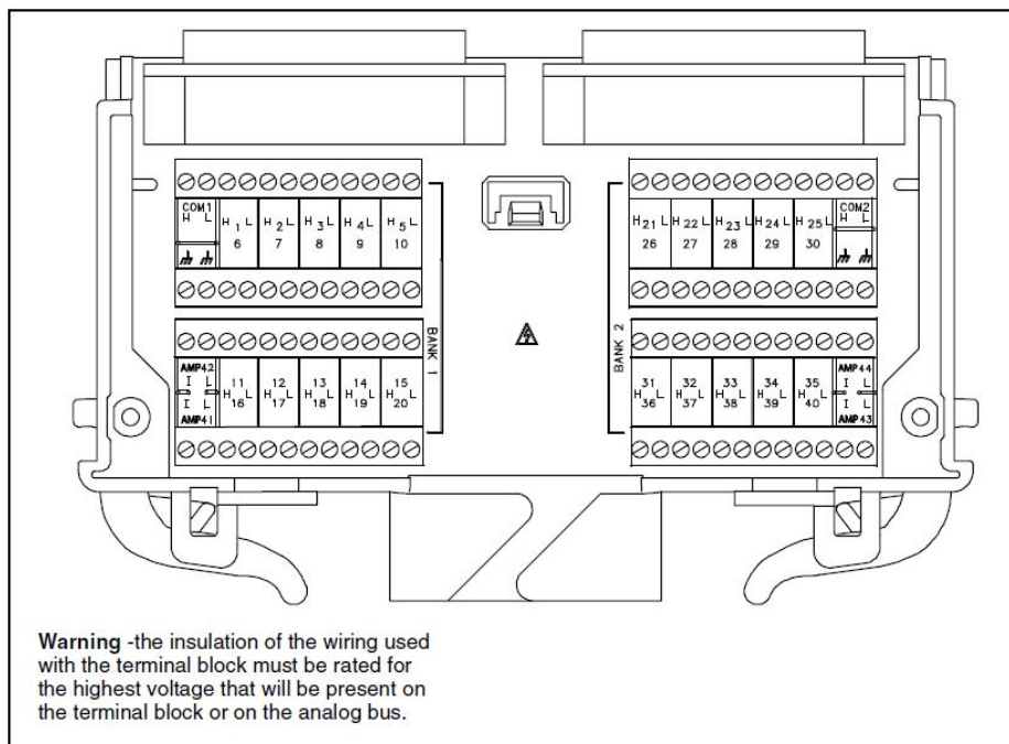
Figure 4-1 34921T Terminal Block.
