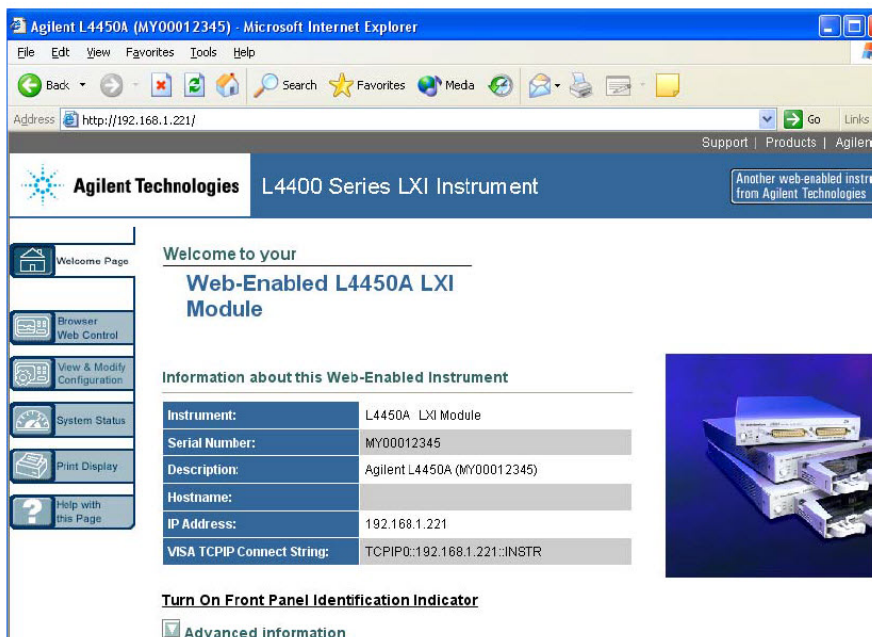
Figure 2-6 L4450A Web Interface (Welcome Page).
