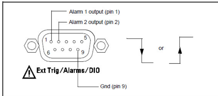
Figure 3-15 The L4400 Series Rear Panel Alarm Connector.
