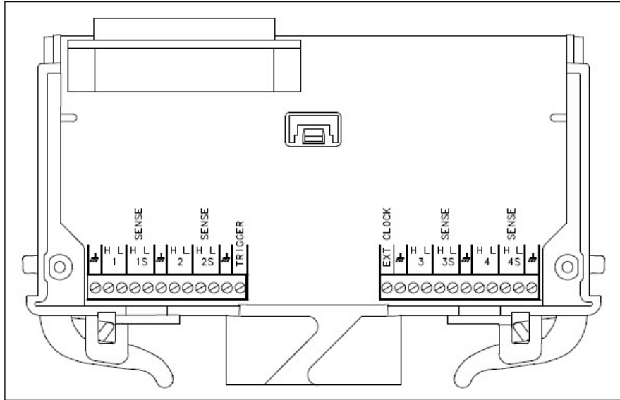
Figure 9-1 L4451A Terminal Block.
