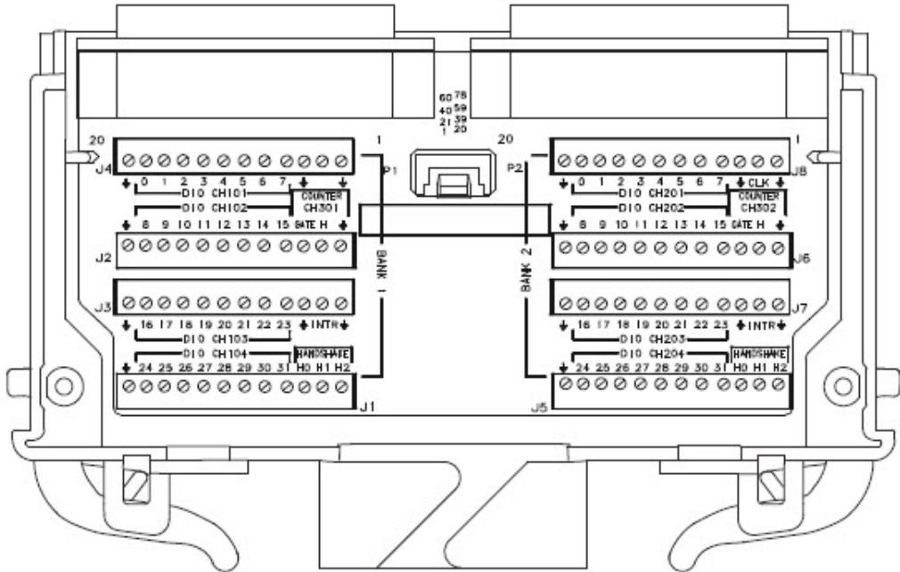
Figure 8-1 L4450A Terminal Block.
