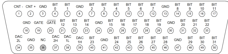
50-Pin D-Sub Female Connector
