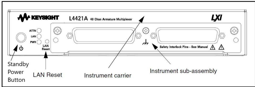
Figure 3-1 L4400 Instrument Front Panel (L4421A shown).
