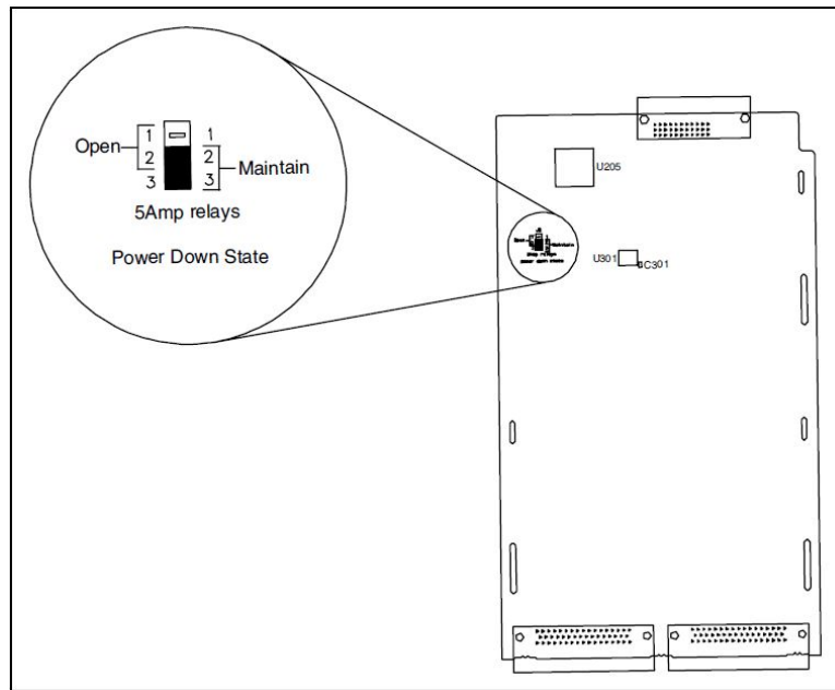
Figure 6-1 5A Relay Power-Down State Jumper.
