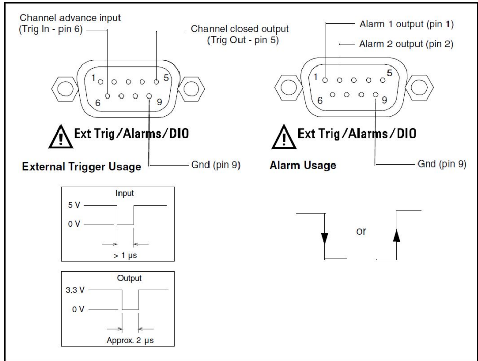
Figure 3-4 External Trigger and Alarm Port Pin Definitions.
