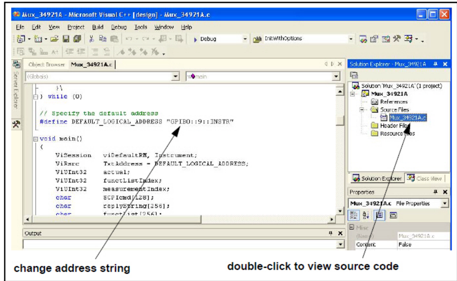
Figure 3-8 Changing the Instrument Address String (VISA Programs).
