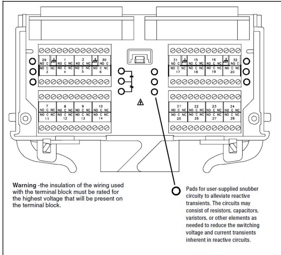
Figure 6-2 L4437A Terminal Block.
