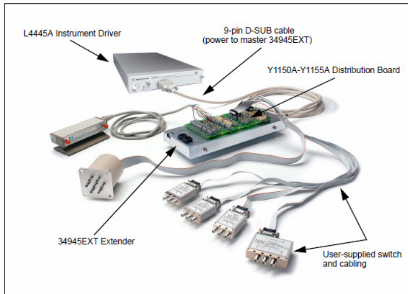
Figure 7-1 L4445A Microwave Switch / Attenuator Driver Configuration.
