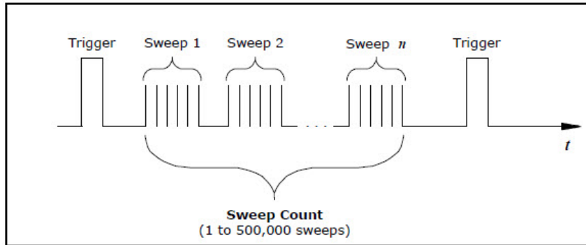
Figure 3-11 Sweep Count Diagram.
