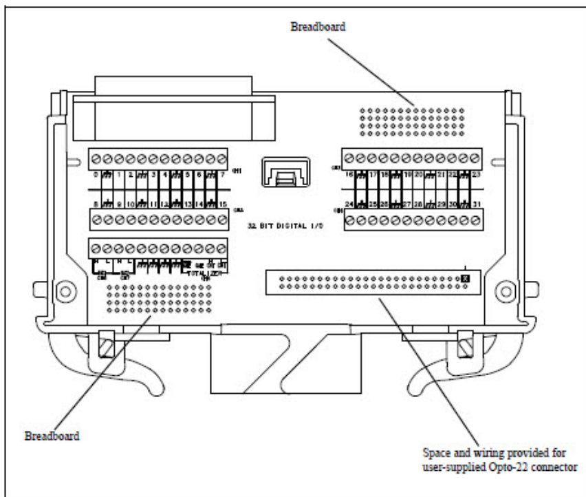
Figure 10-1 L4452A Terminal Block.
