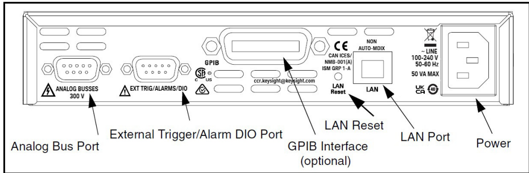
Figure 3-2 L4400 Instrument Rear Panel (L4421A shown).
