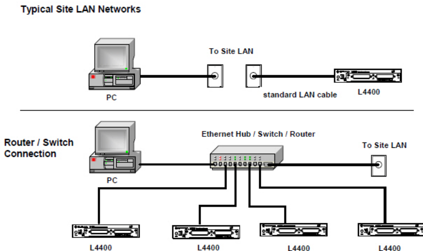
Figure 2-3 Typical Site LAN Network Connections.
