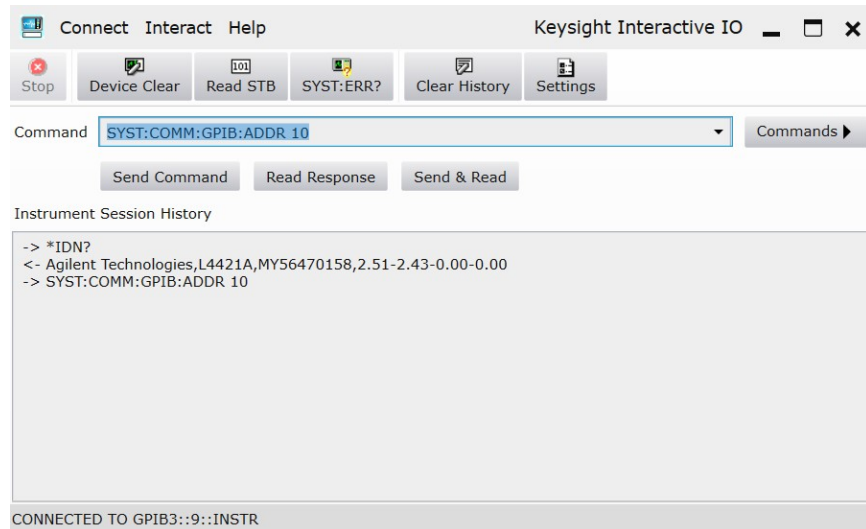
Figure 2-10 Setting the GPIB Address Using the Interactive IO Window.
