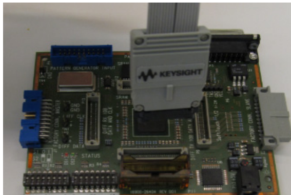
Figure 1 E5386A half channel adapter
