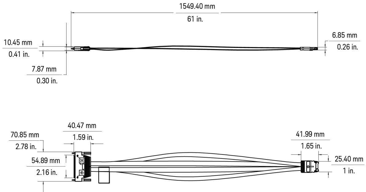
Figure 3 U4205A 38-pin single-ended probe dimensions
