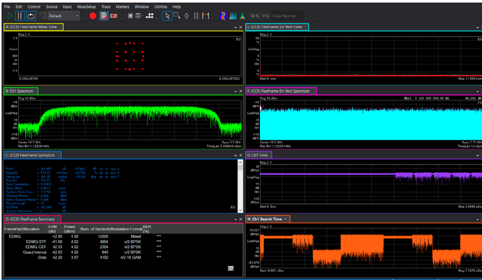
Figure 9: This picture shows the Enhanced Directional Multi-Gigabit (EDMG) measurement of 802.11ay signal with channel bonding of two 2.16 GHz channels using Flex Frame. It shows how Flex Frame can be used to measure EDMG-STF, EDMG-CEF, guard interval, and data portions of the 802.11ay signals.
