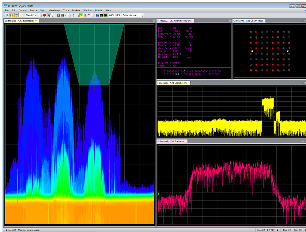
Figure 7. Create and execute a spectrally-selective frequency mask trigger from PathWave Vector Signal Analysis (VSA) software when connected to real-time enabled UXA, PXA, and MXA signal analyzers.
