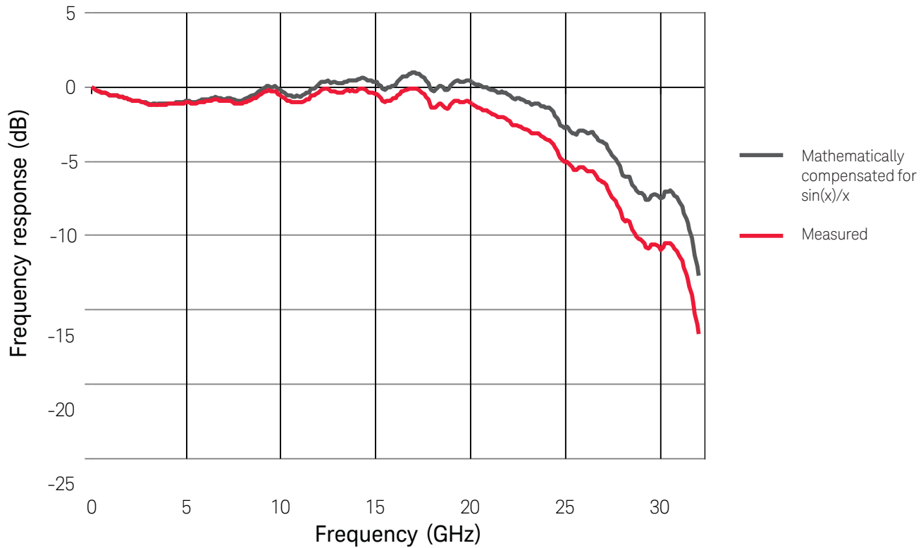
Figure 10. Nominal frequency response measured with a sample rate of 64 GSa/s and a multi-tone signal containing frequencies from DC to 32 GHz with equal amplitudes
