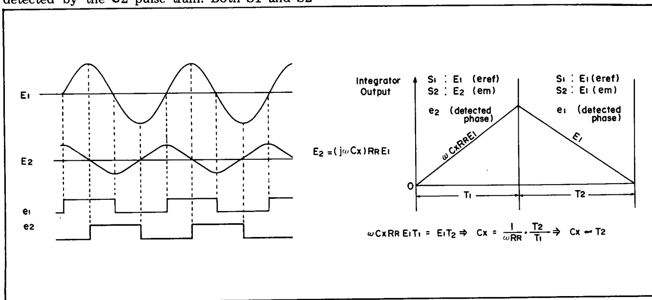
Figure 8-2. C_p Measurement.
