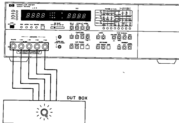
(a) (b) Figure 4-4. Dissipation Factor Accuracy Test Setups.
