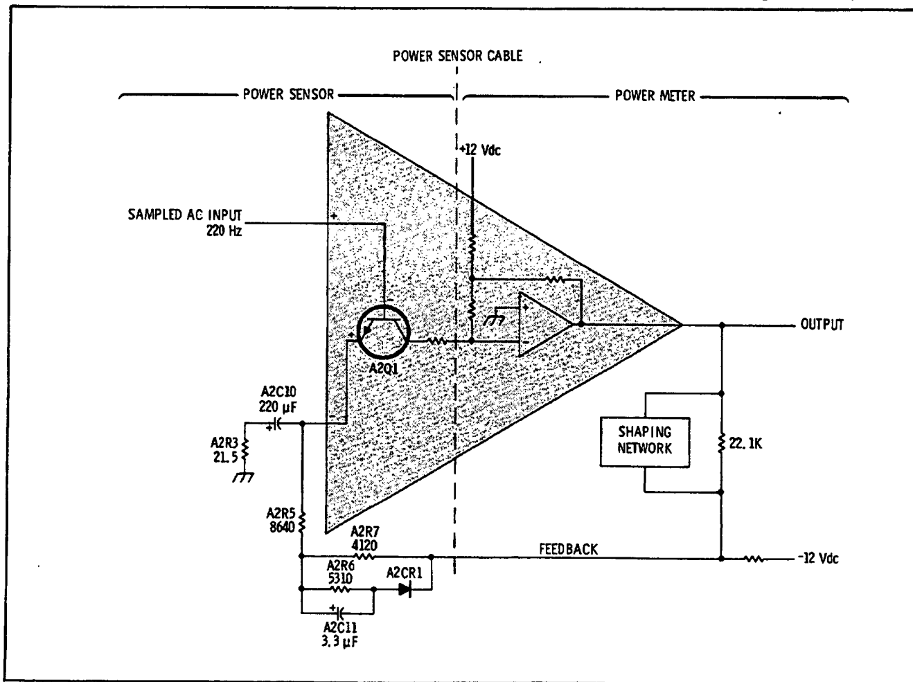
Figure 6. Operational Amplifier
