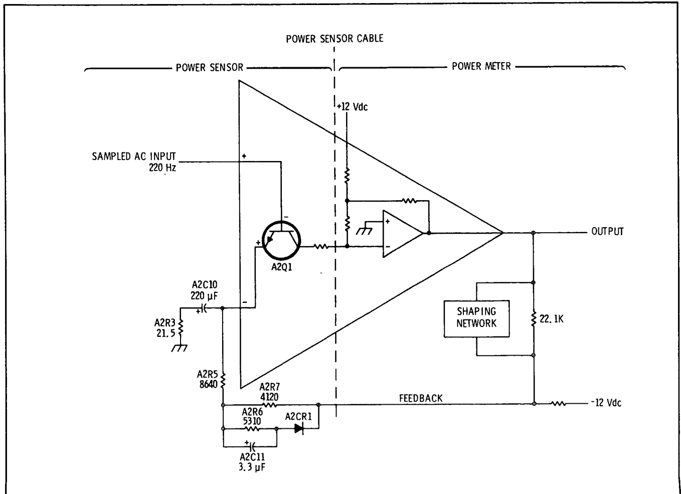
Figure 6. Operational Amplifier
