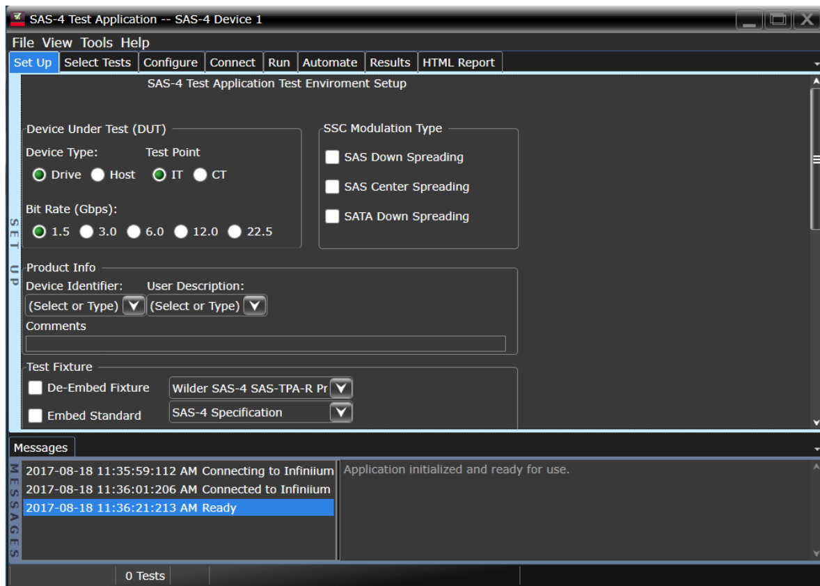
Figure 1. The Keysight automated test engine guides you quickly through selecting and configuring tests, setting up the connection, running the tests, and viewing the results. You can easily select individual tests or groups of test with a mouse-click and customize your output report based on the test results you want to see.
