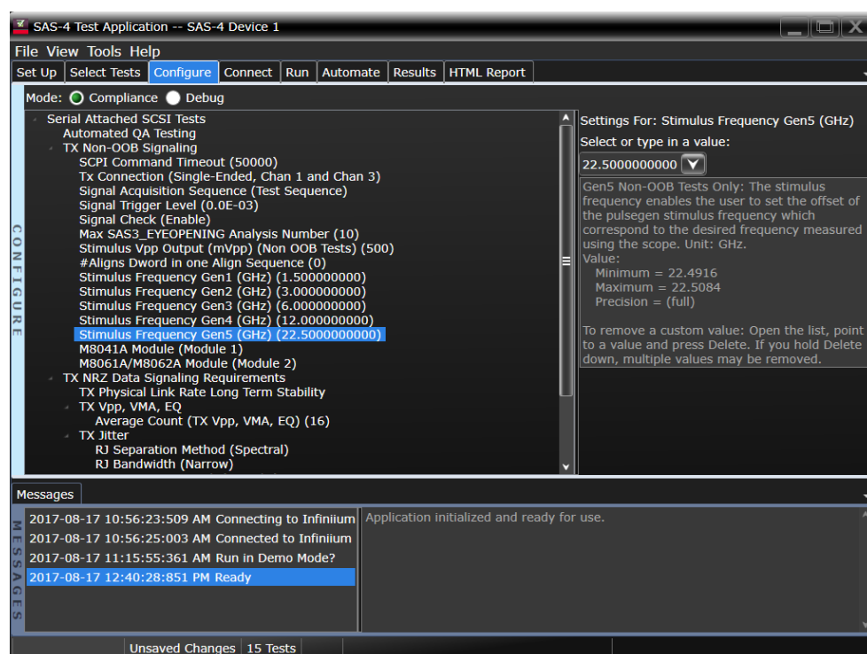
Figure 2. In configuring the tests, you define the number of UI to test, whether a TCTF load is being used and how the differential inputs and transient test probe are connected to the oscilloscope.
