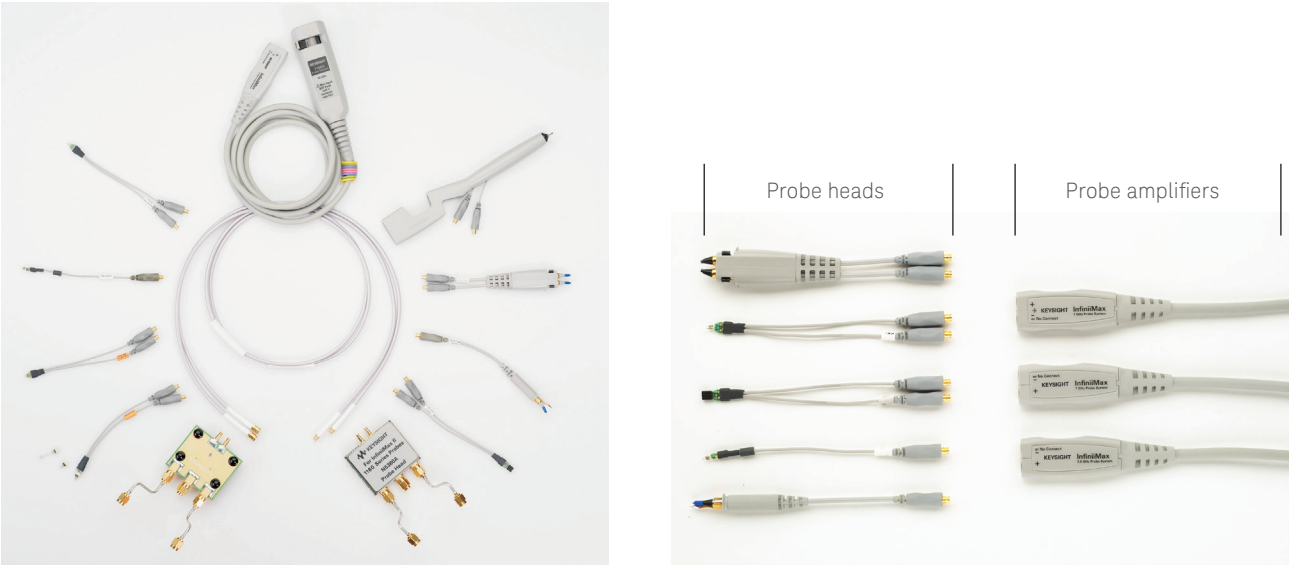
Figure 2. InfiniiMax probe heads combine with probe amplifiers for a flexible probing system.
