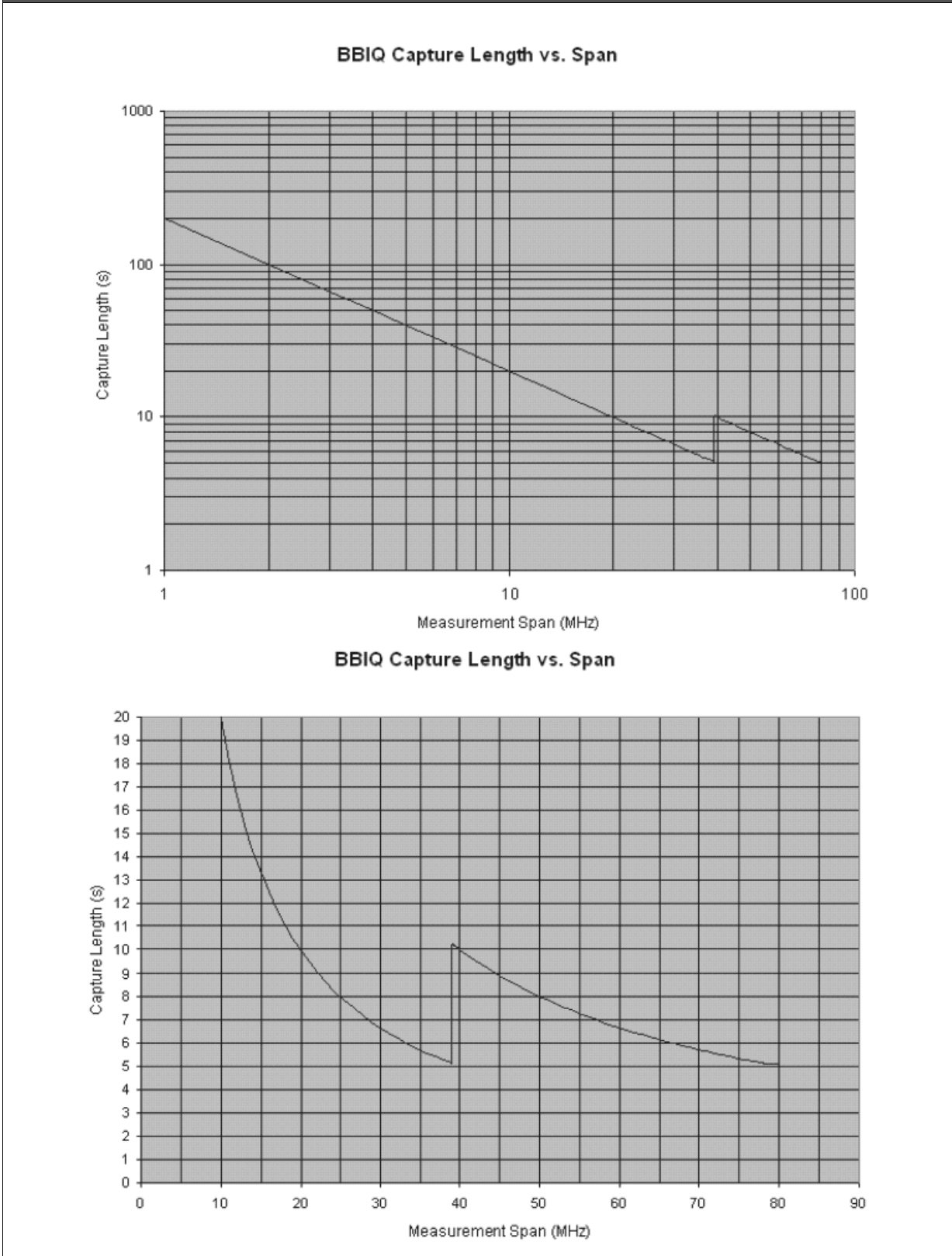
Capture Length vs. Span, 2-channel with 89600 VSA, I+jQ Mode [Plot]
