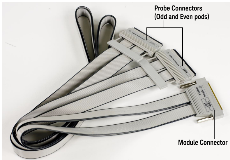
Figure 27 U4201A 90-pin two pod cable
