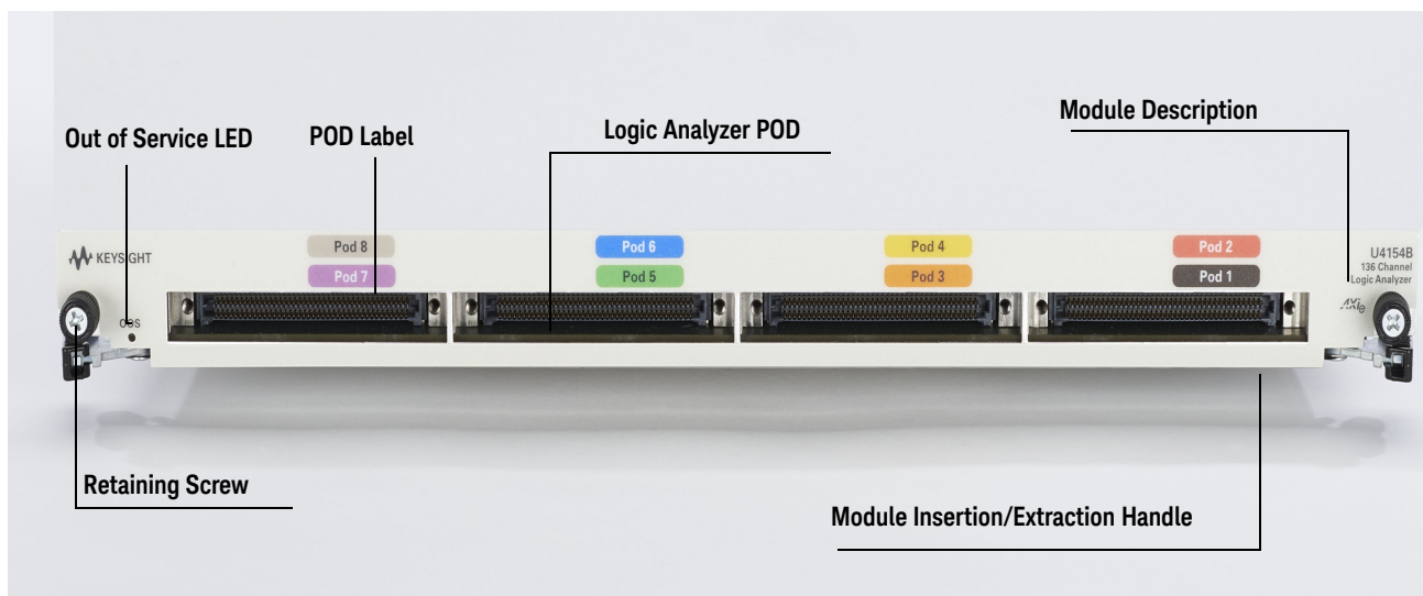
Figure 7 U4154B module
