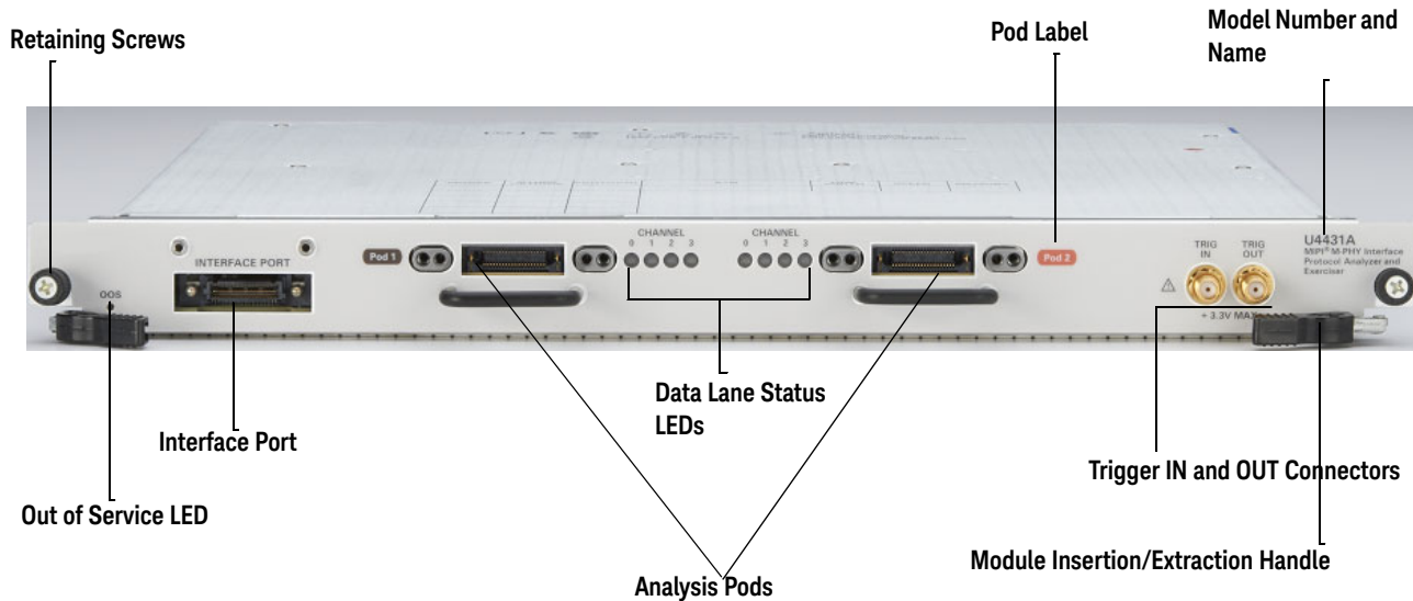
Figure 13 U4431A Module
