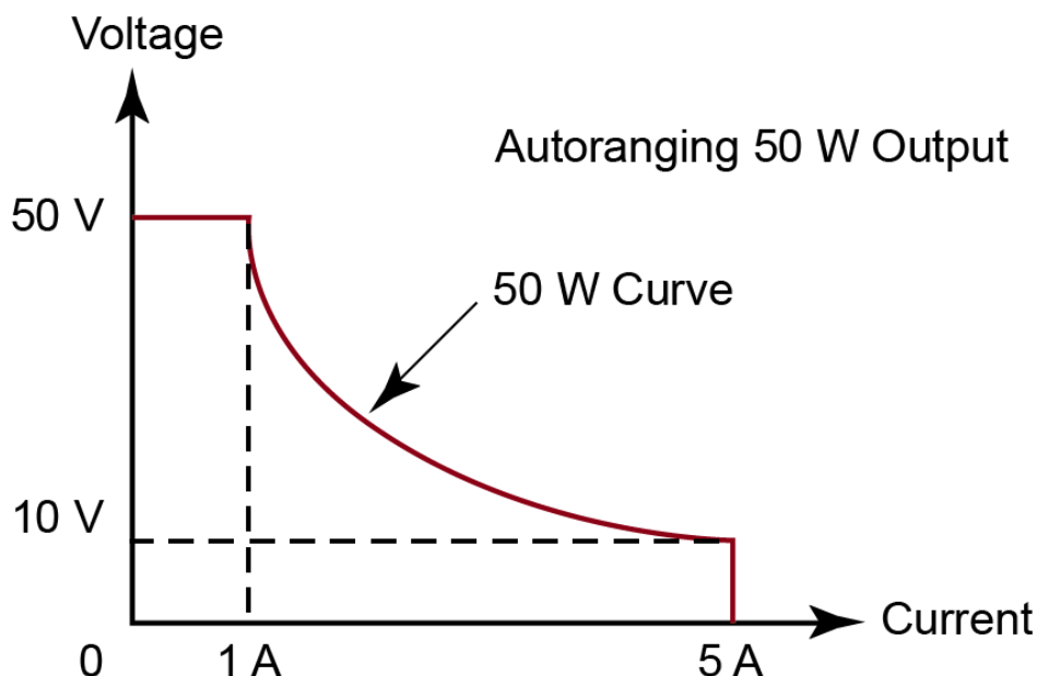
Figure 7. Autoranging characteristics
