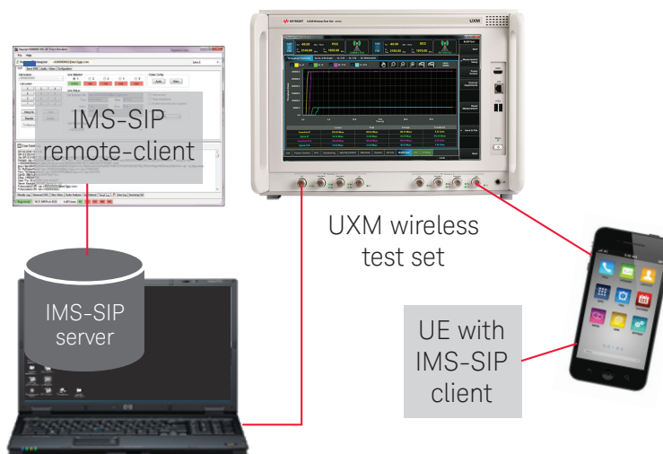
Figure 1. Typical configuration for LTE UE test
