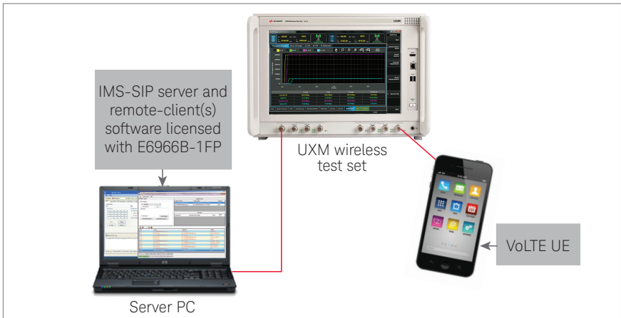
Figure 5. Example test configuration for UE with native client, connecting with an Keysight IMS-SIP server and remote-client software on server PC
