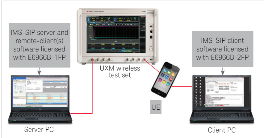
Figure 6. Example test configuration for UE without a native client (requires the addition of a client PC running Keysight IMS-SIP client software)
