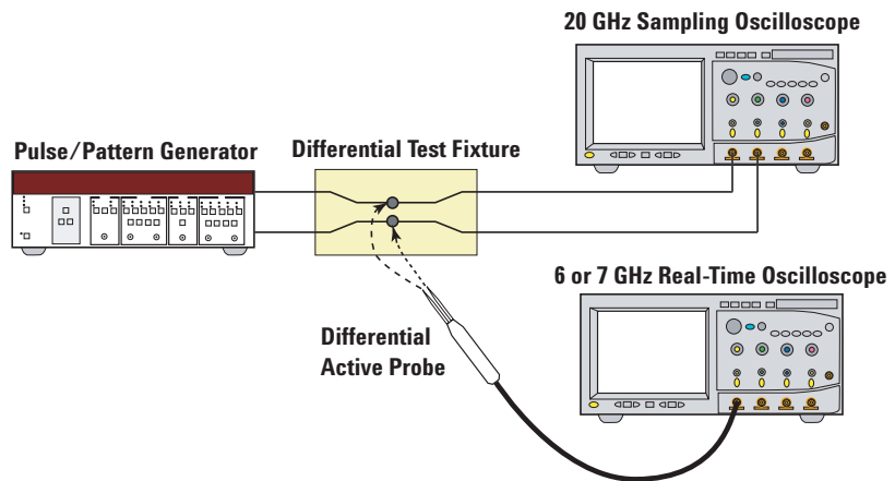
Figure 1a. Block diagram of test setup.
