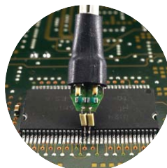
Figure 24. InfiniiMax 7 GHz differential solder-in probe head.
