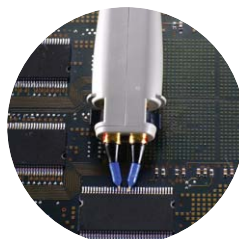
Figure 23. InfiniiMax 6 GHz differential browser probe head
