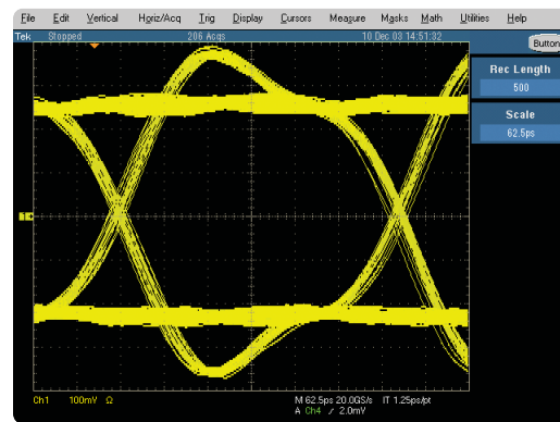
Figure 17. Measured response of 100 ps edge-speed signal using Tektronix P7250 active probe with solder-in connection.
