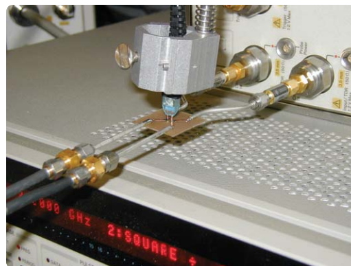
Figure 1b. Test setup with probe attached to test fixture using probe stand holder.
