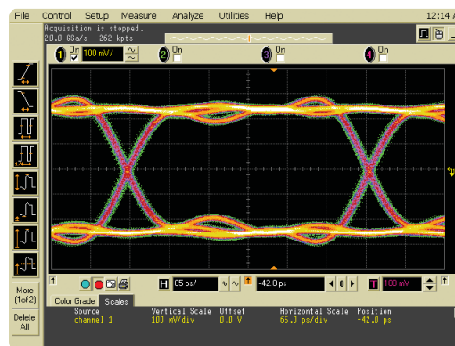
Figure 10. Measured response of 50 ps edge-speed signal using Agilent's 1134A InfiniiMax solder-in probe head.
