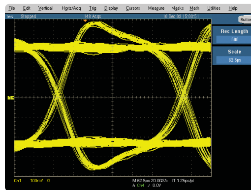
Figure 8. Measured response of 50 ps edge-speed signal using Tektronix P7250 with solder-in connection.
