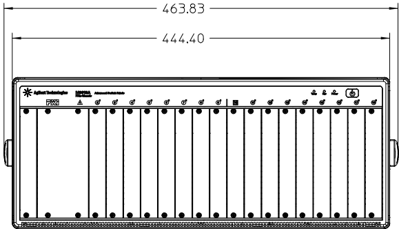
FRONT VIEW SCALE 0.33X
