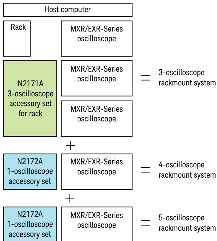
Figure 7 Expansion Accessories Required for Three- to Five-Oscilloscope (MXR/EXR-Series) Rackmount System
