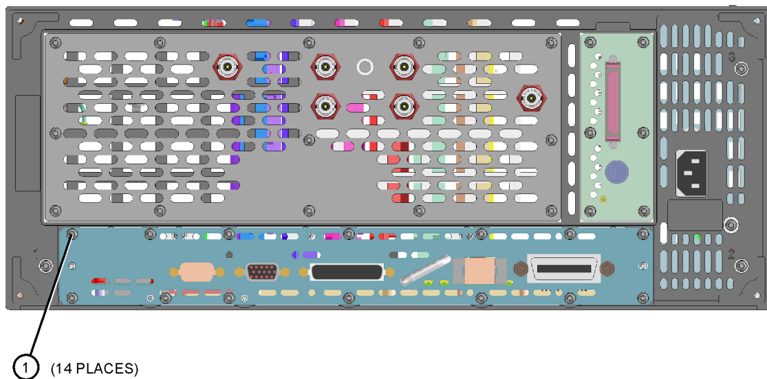
Figure 5 CPU Screw Locations
