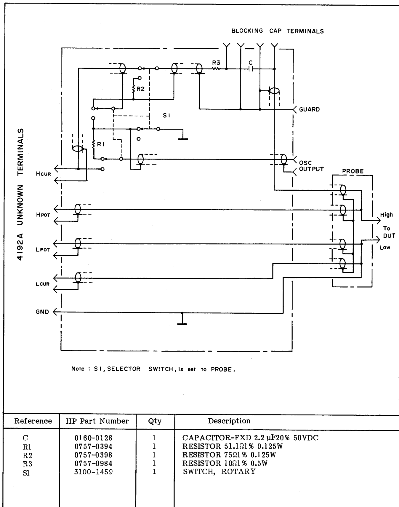
Figure 6. Model 16095A Schematic Diagram.
