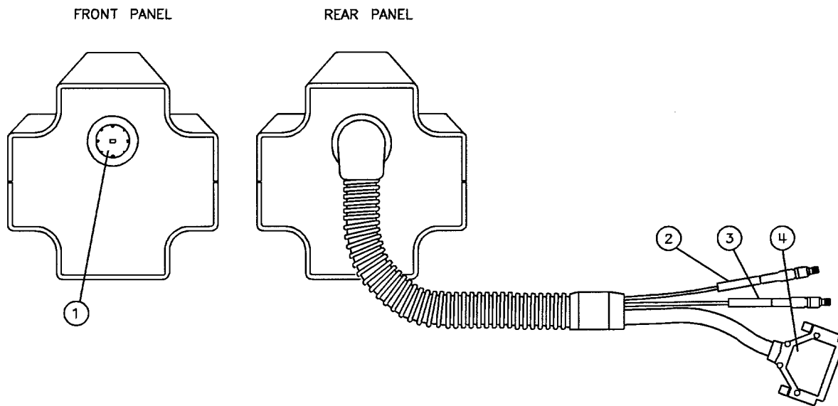
Figure 5-1 Front and Rear Panel Features of the HP 85104A (all waveguide bands)
