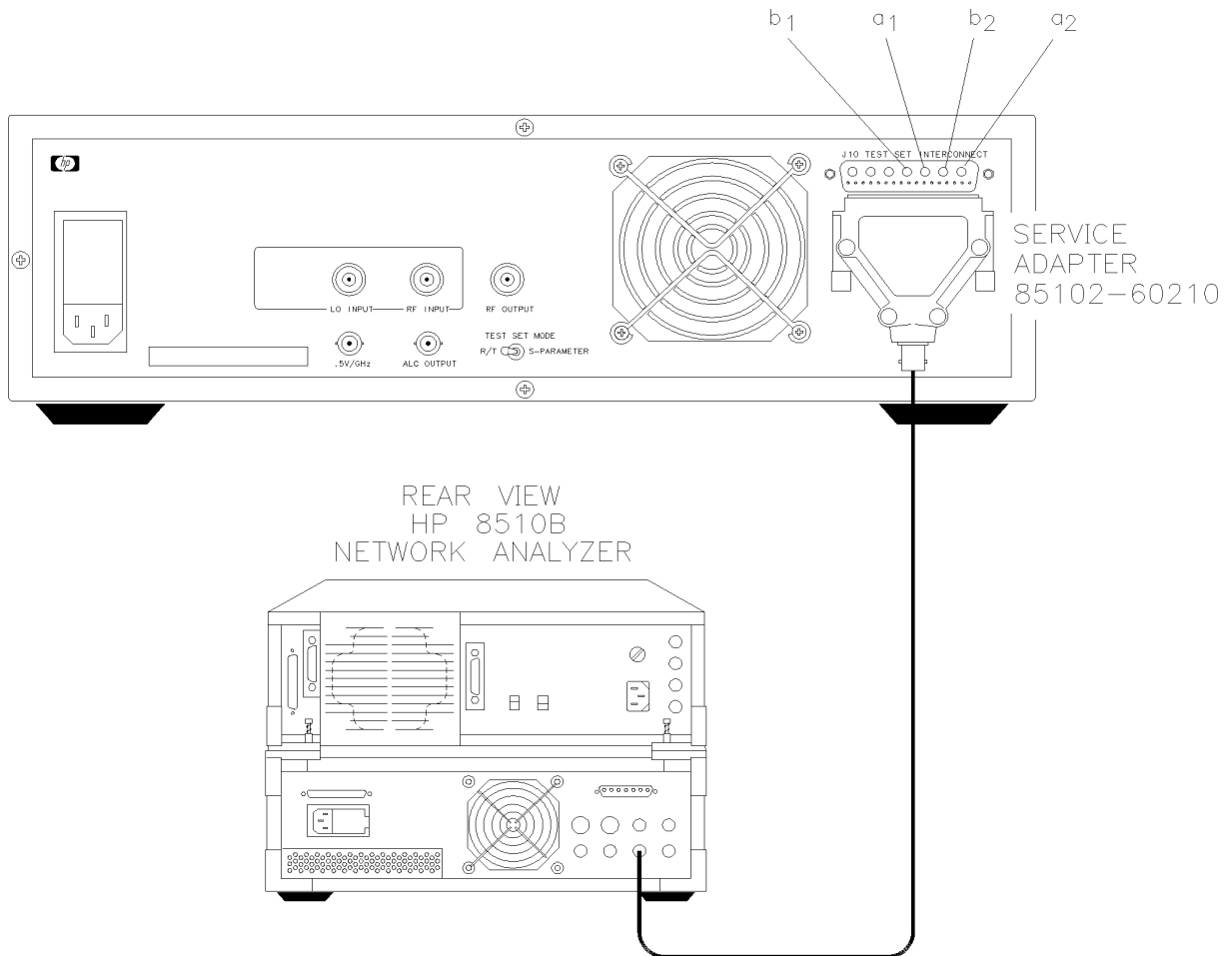
Figure 6-24 Multiplexer Inputs
