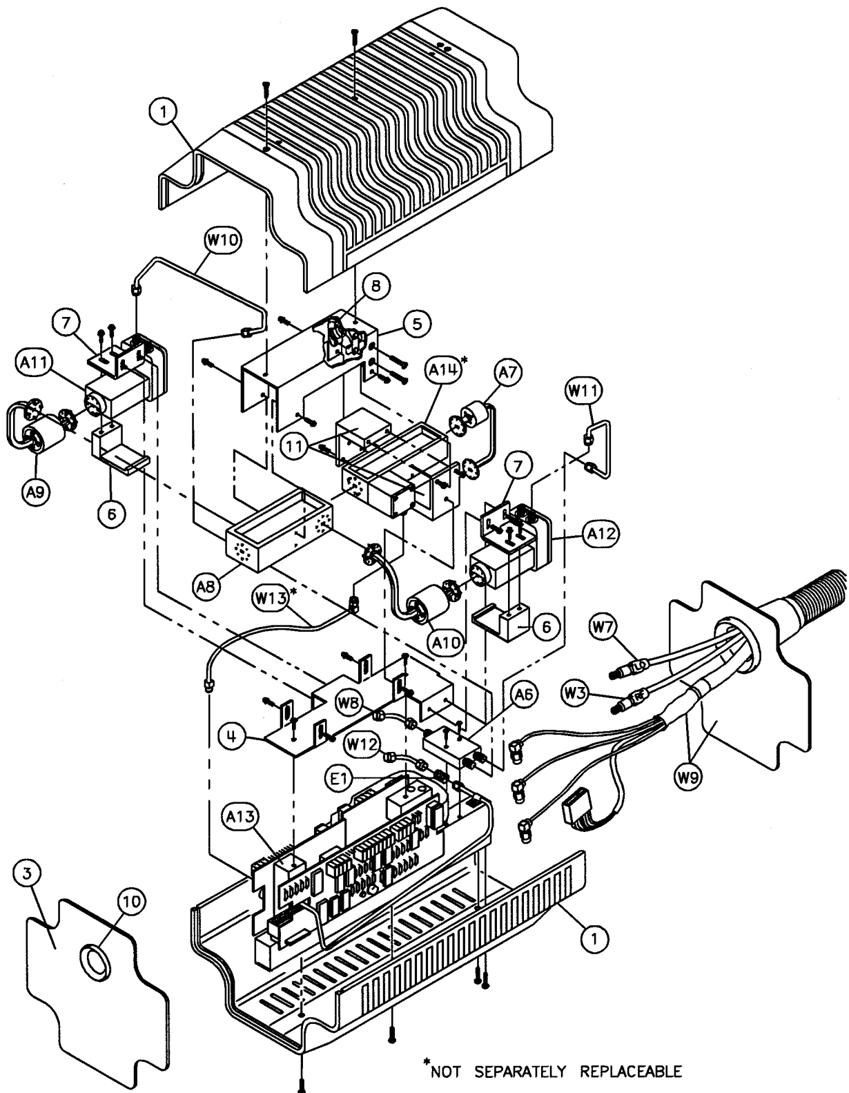
Figure 5-16 HP W85104A Replaceable Parts
