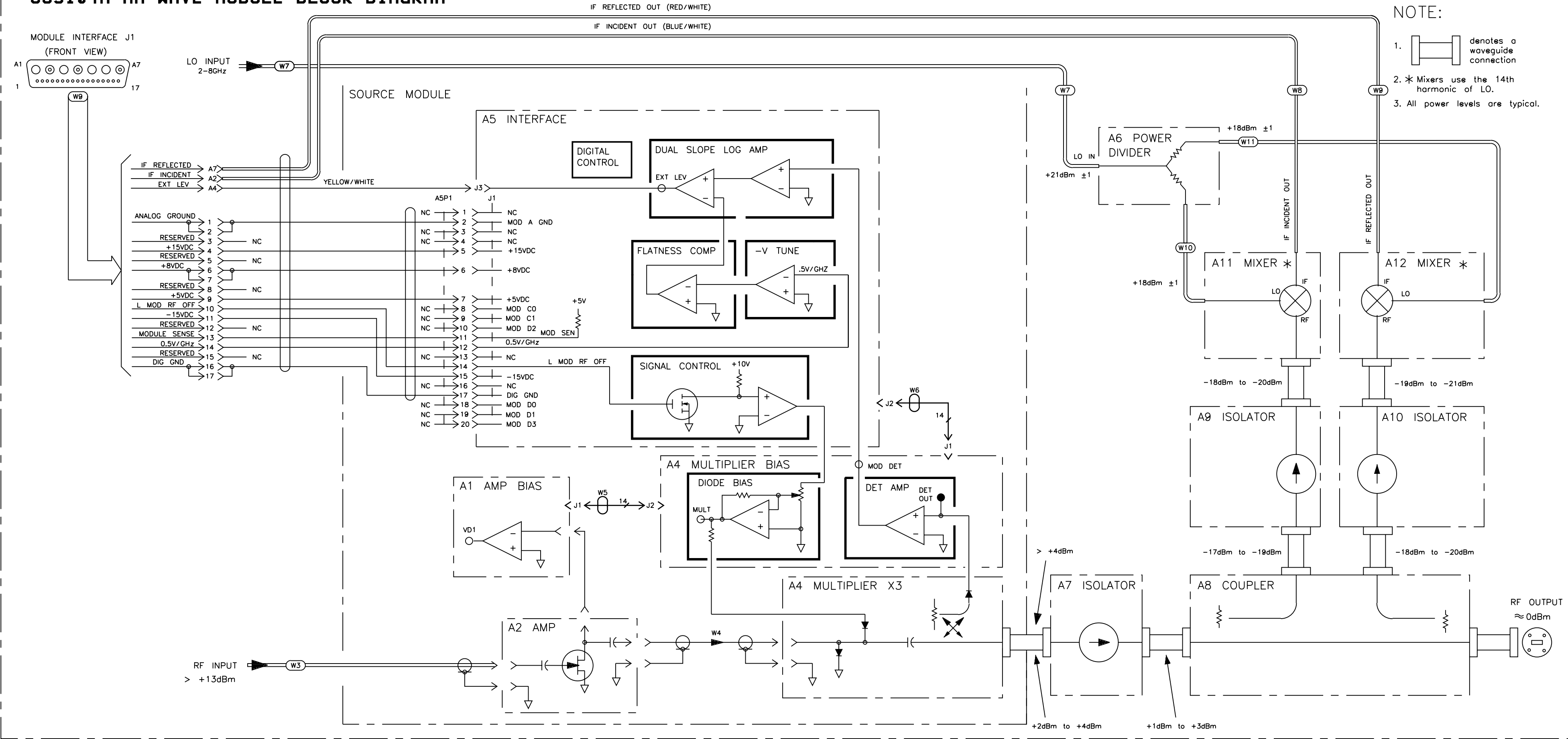
Figure 5-8. HP U85104A Block Diagram
