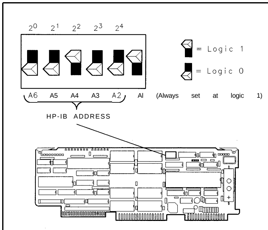
Figure 2-18. Address Switch Set to 4
