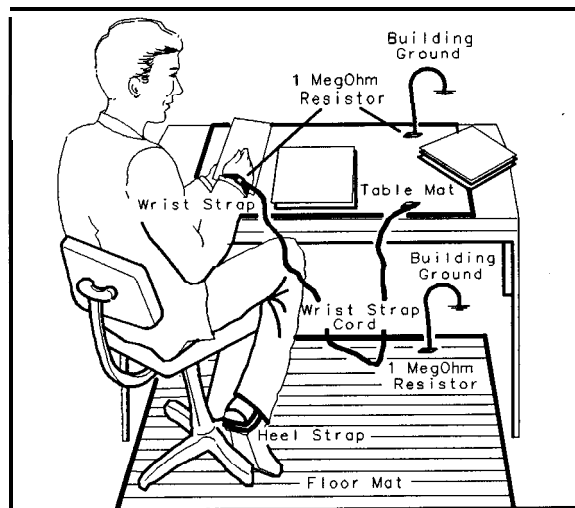
Figure 1-4. Static-Safe Workstation
