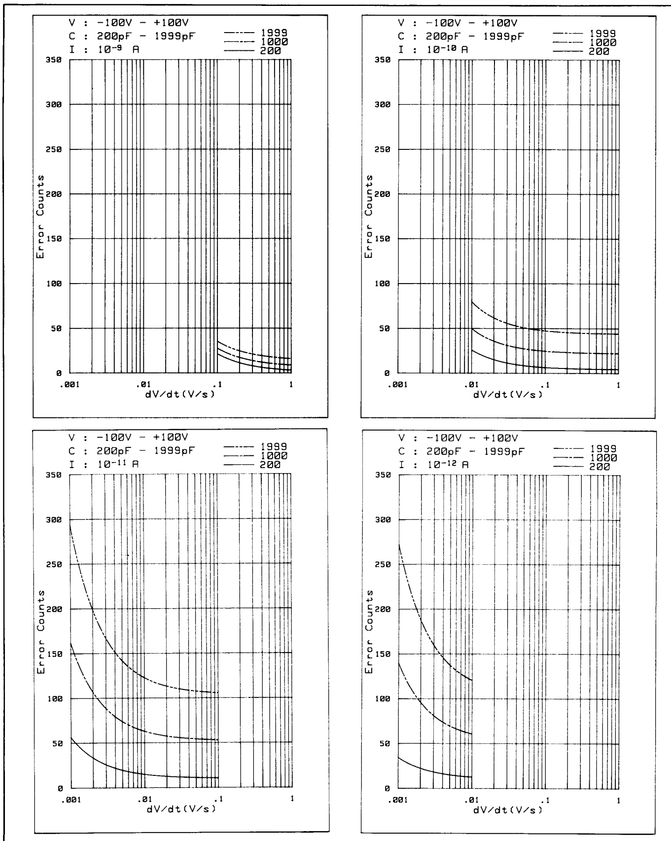
Figure 3-22. C-V Measurement Accuracy (Sheet 4 of 4).
