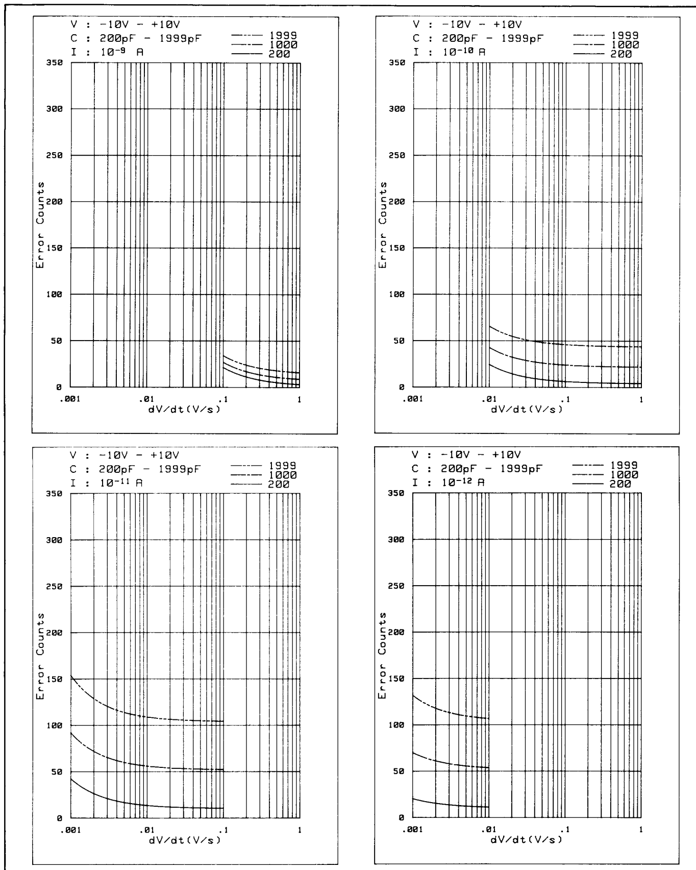
Figure 3-22. C-V Measurement Accuracy (Sheet 2 of 4).
