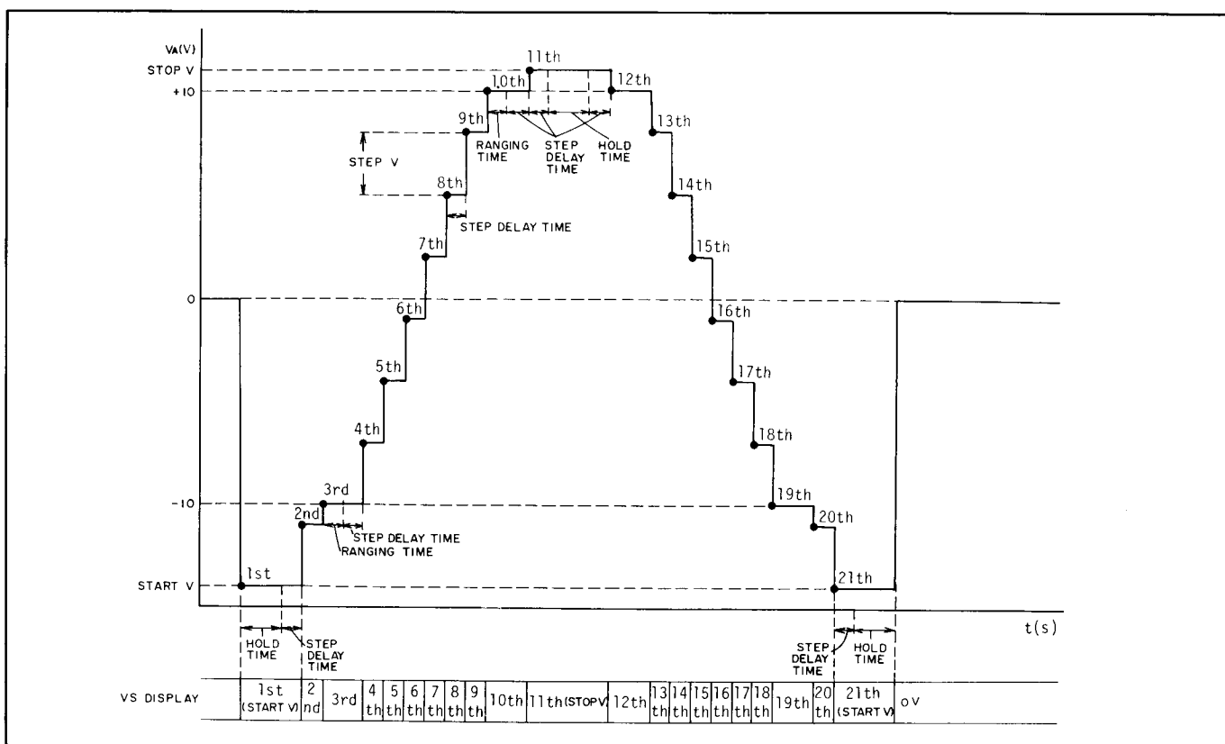
Figure 3-8. Relationship between Output Voltage and Display for \text{J}^{\text{r}} (Double Staircase Wave).
