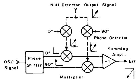
4275A Modulator Operating Principle.
