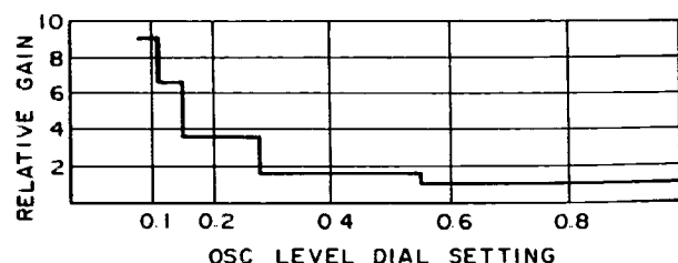
Figure 8-12. AM Amplifier Gain Control.
