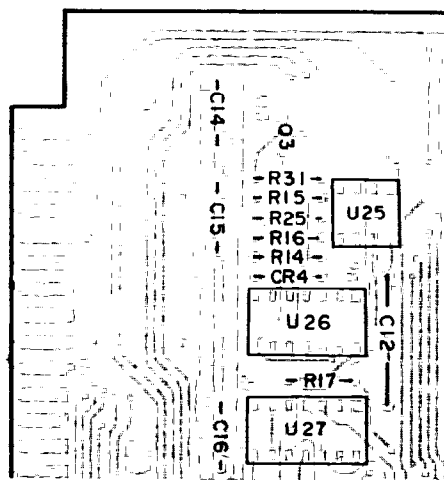
Figure 8-63. A9 Component Locations.
