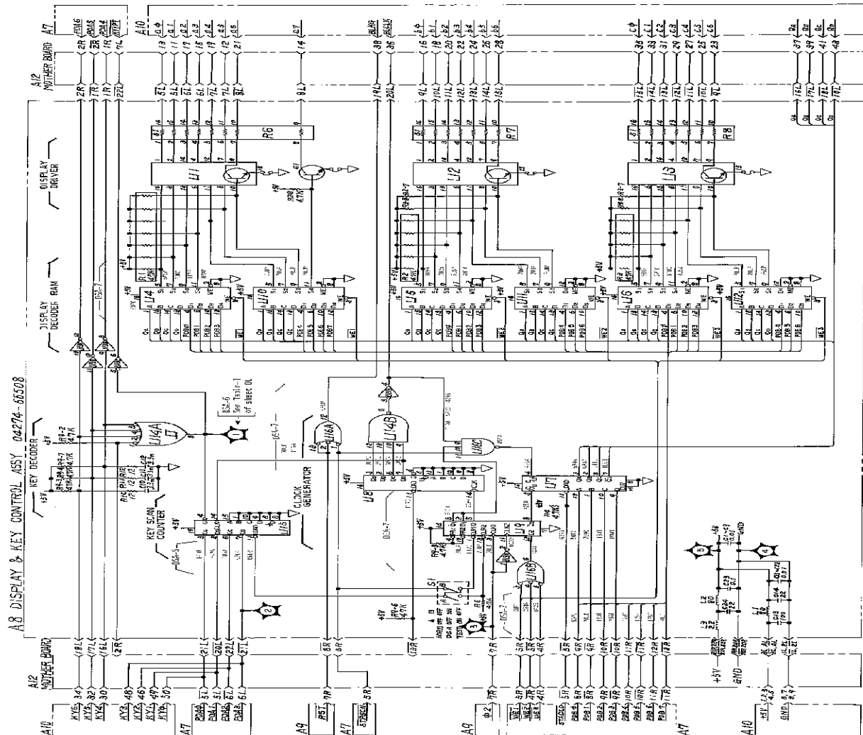
Figure 8-62. AA Display Control Board Assembly Schematic Diagram.
