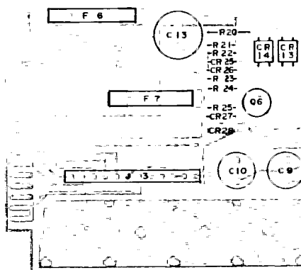
Figure 8-67. All Component Locations.
