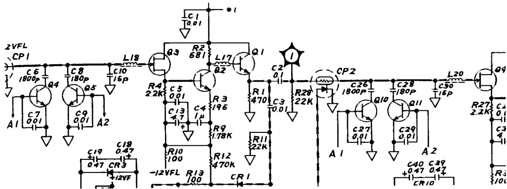
Figure 8-58 (B). A6 Schematic Diagram.
