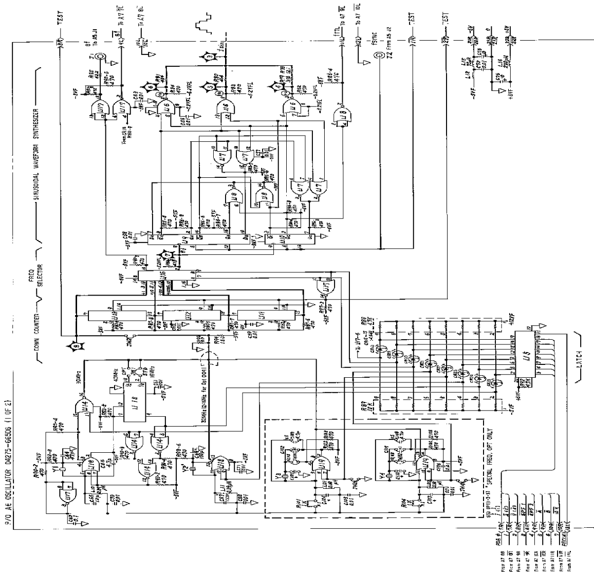
Figure 9-58(a). A6 Oscillator Board Assembly Schematic Diagram [Sheet 1 of 2].
