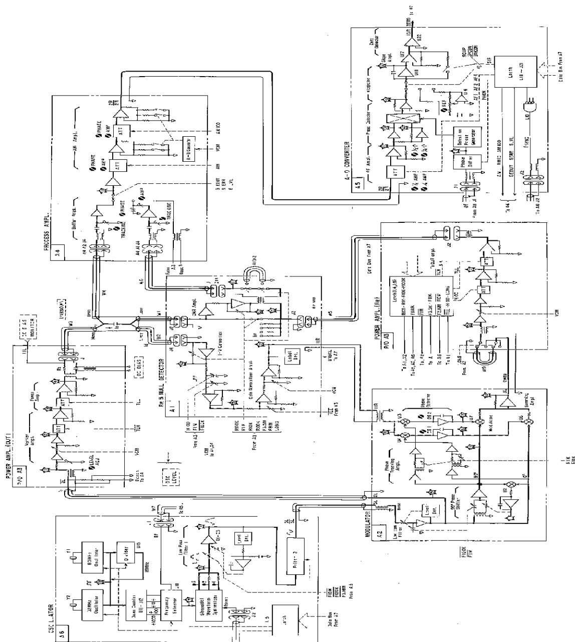
Figure 8-16. Analog Measurement Section Schematic Block Diagram.
