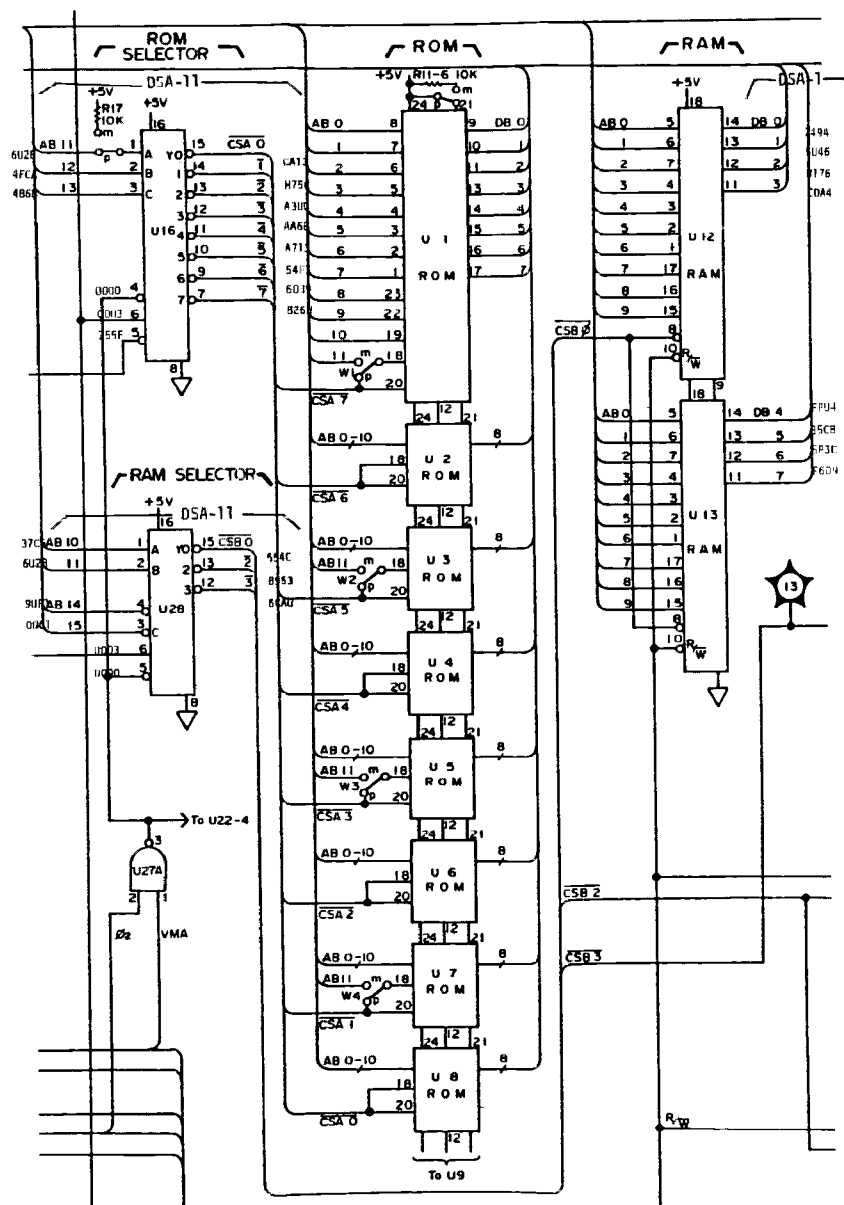
Figure 8-64. A9 MPU Assembly Schematic Diagram.
