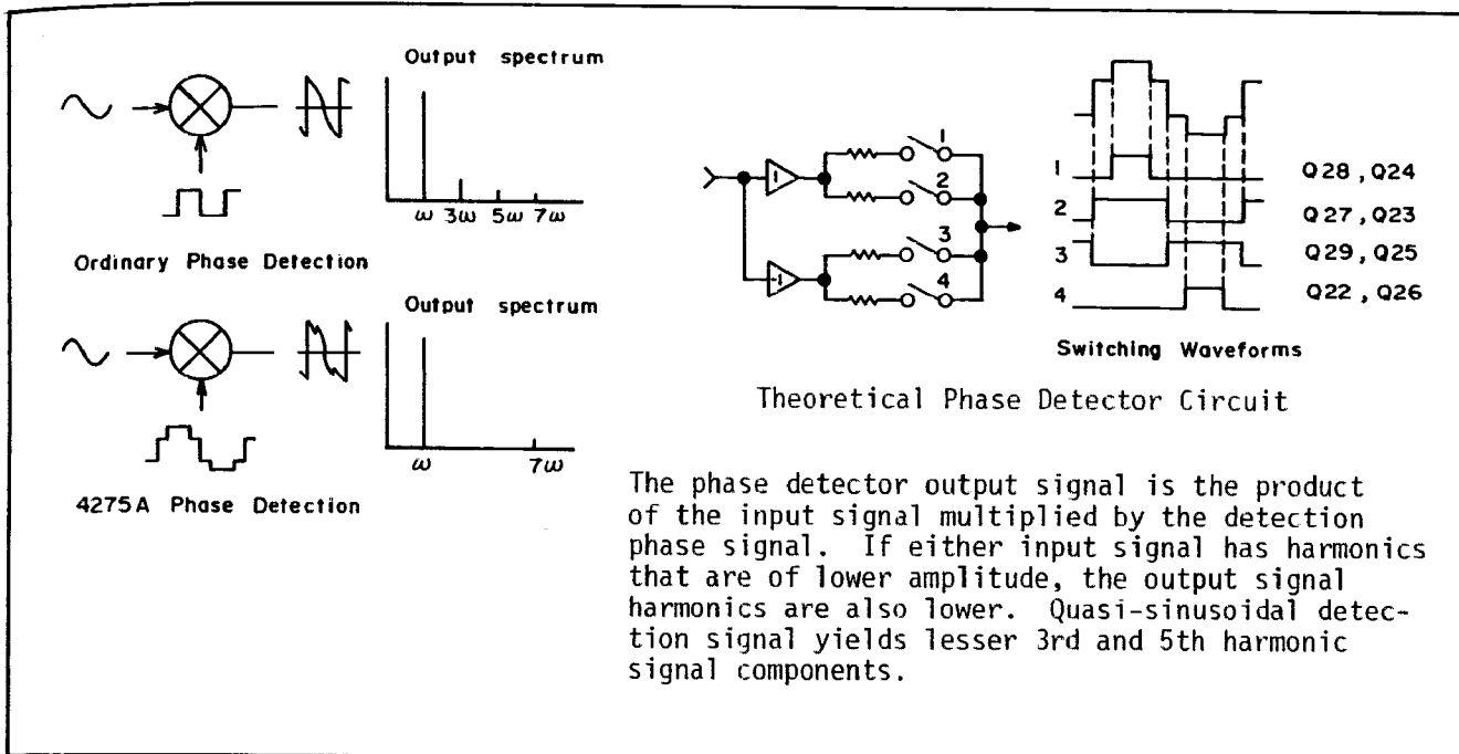
Figure 8-14. 4275A Phase Detector Operating Principle.
