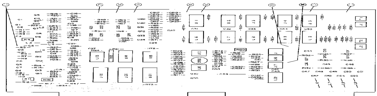
Figure 8-25. M-10 Converter Base Assembly Component Layout.
