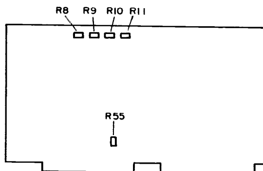
A23 Board Adjustment Locations.
