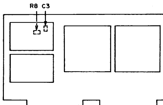
A4 Board Adjustment Locations.
