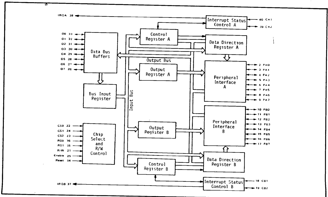
Figure 8-19. PIA Internal Circuit Configuration.
