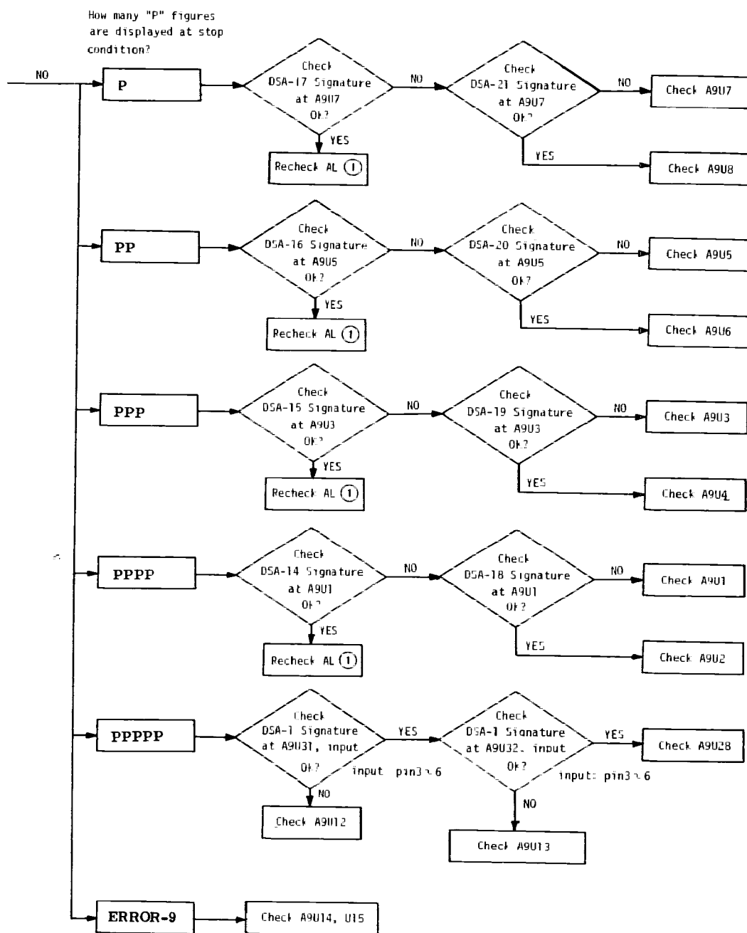
Page 8-51, Figure 8-33. Digital Section Troubleshooting Flow Diagram BL: Partially change the flow diagram as follows:
