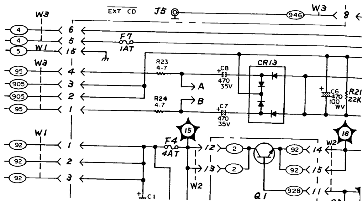
Figure 8-68. All Schematic Diagram.
