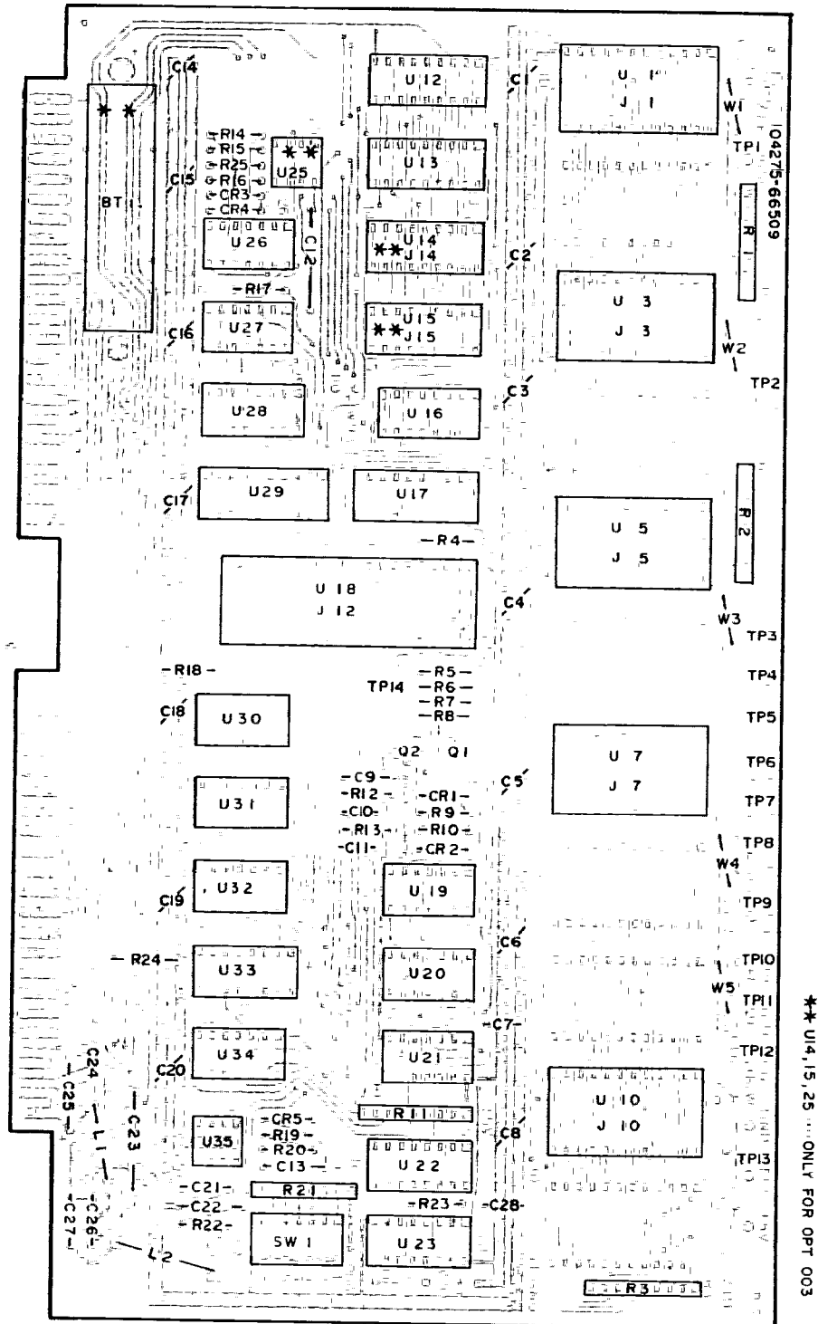
Figure 8-63. A9 MPU Component Locations.
