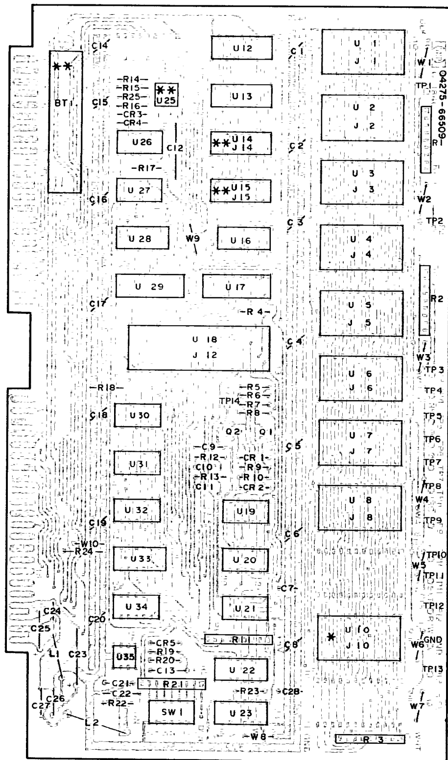
Figure 8-63. A9 Component Locations.
