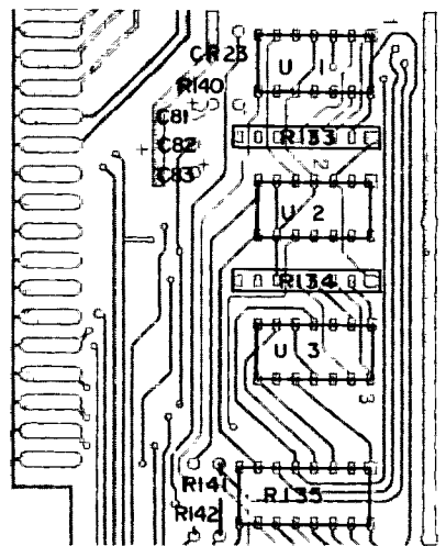
Figure 8-48. A3 Component Locations.
