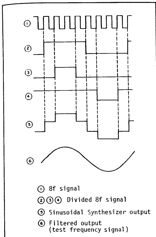
Figure 8-8. Sinusoidal Synthesizer Waveforms.
