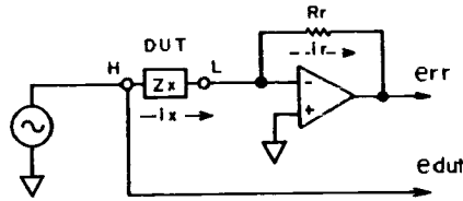
Figure A Low Frequency Vector Voltage-Current Method with Feedback Amplifier.
