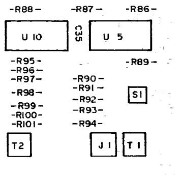
Figure 8-54. A5 Component Locations.
