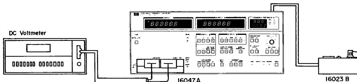
Figure 4-7. Option 001 Int DC Bias Supply Test Setup.
