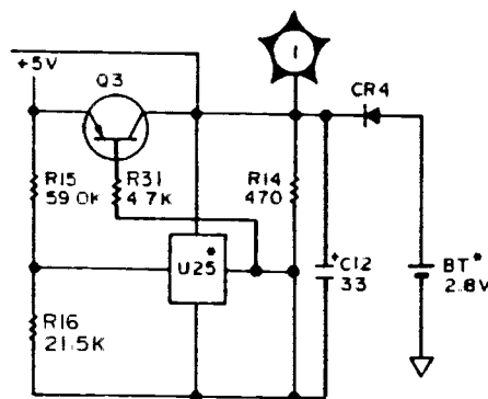
Figure 8-64. A9 MPU Assembly Schematic Diagram.
