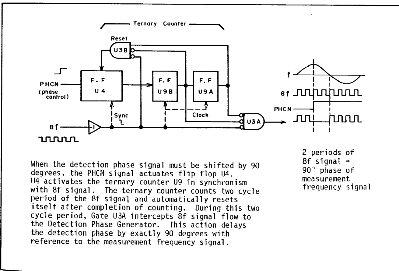
Figure 8-15. Detection Phase Shifter Operating Principle.
