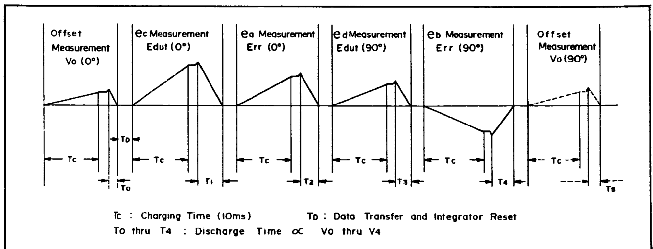
Figure 8-5. Integrator Vector Voltage Ratio Detection Timing.
