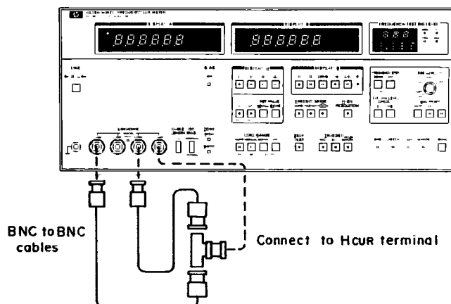
Figure 5-7. Process Amplifier Gain Adjustment Setup.
