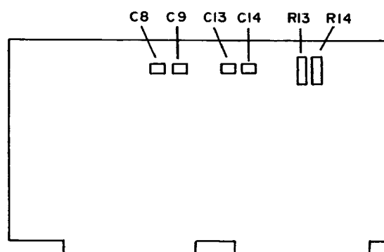
A2 Board Adjustment Locations.
