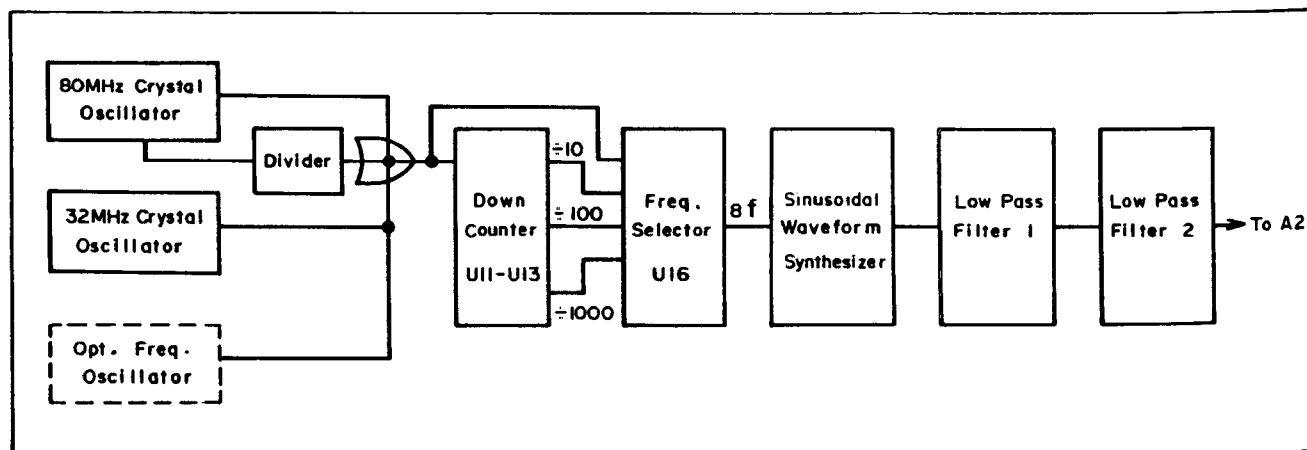
Figure 8-7. A6 Oscillator Block Diagram.
