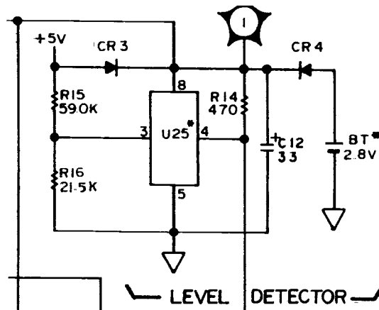
Figure 8-64. A9 MPU Assembly Schematic Diagram.
