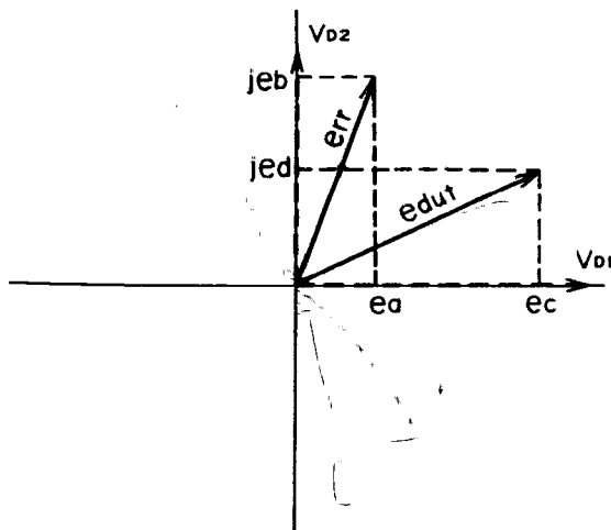
V_{01}, V_{02} : Orthogonal phase detection signals
