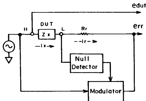
Figure 8-2. 4275A Vector Voltage-current Method.
