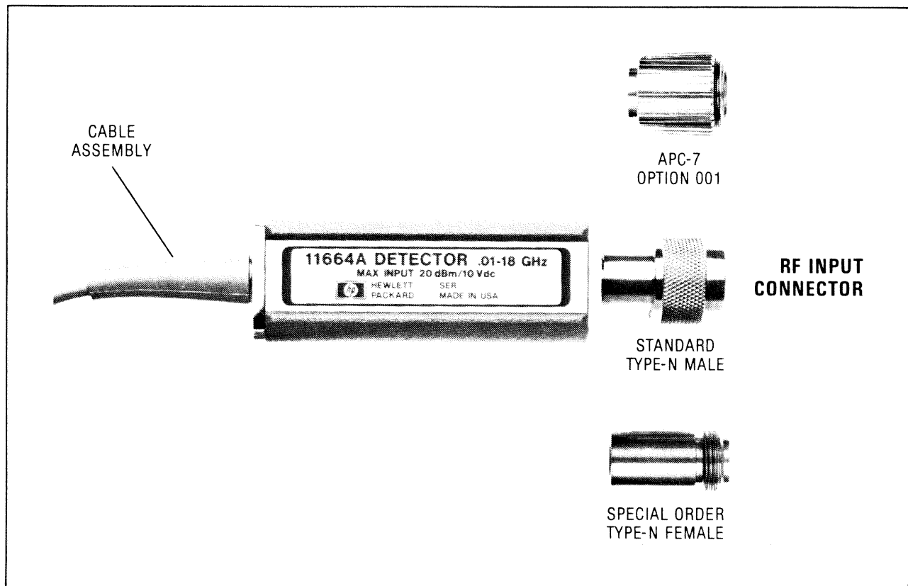
Figure 8-1. Major Assemblies
