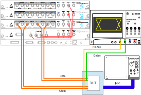
Figure 45 M8195A single module connection setup
