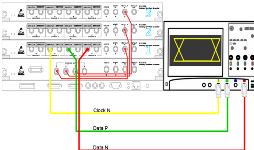
Figure 43 Connections for specific Calibration Small LP Amplitude procedures
