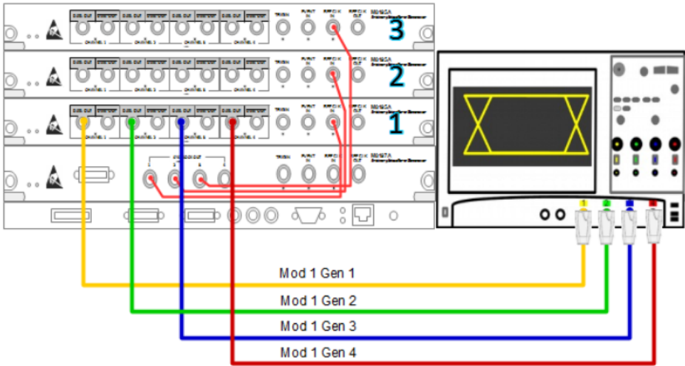
Figure 44 Connection Settings for most Calibration Small LP Amplitude procedures
