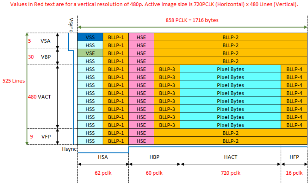
Figure 37 Block Diagram for Video transmission in Non-Burst mode with Sync Pulses
