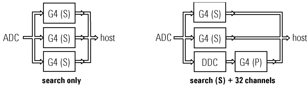
Figure 23. E9821 configuration examples for search and signal processing
