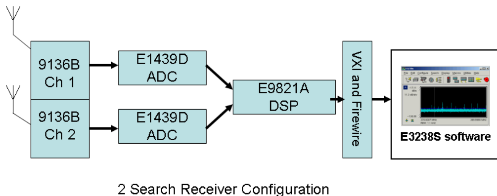
Figure 39. Dual Tuners in a 2 Search Receiver Configuration
