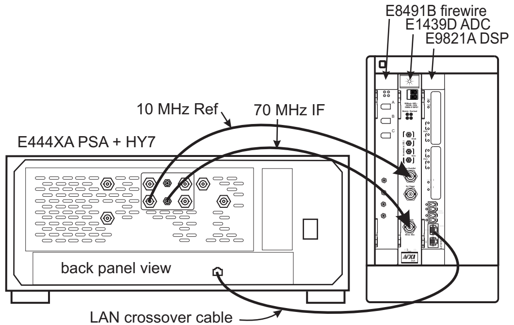
Figure 10. PSA tuner cabling
