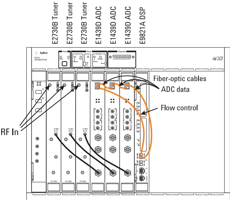
Figure 65. VHF/UHF 3-channel E1439D system
