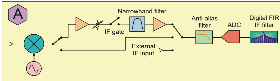
Receiver Block Diagram
