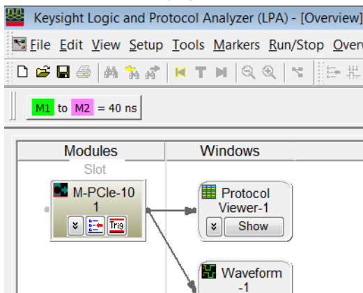
Figure 6 Software Installation
