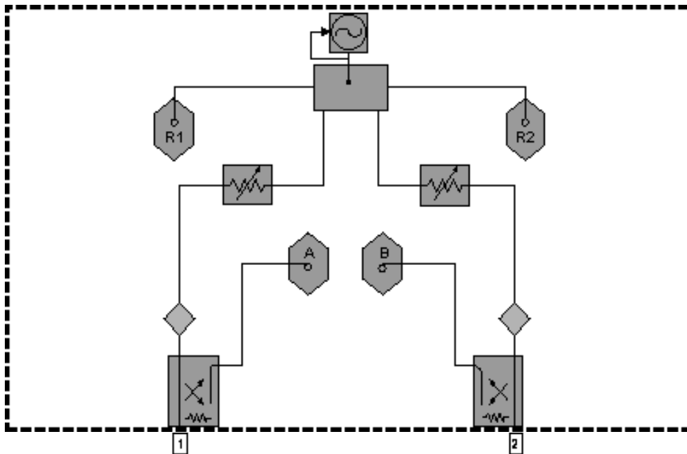
E8361A/C - Option UNL Standard Configuration with Extended Power Range and Bias - Tees
