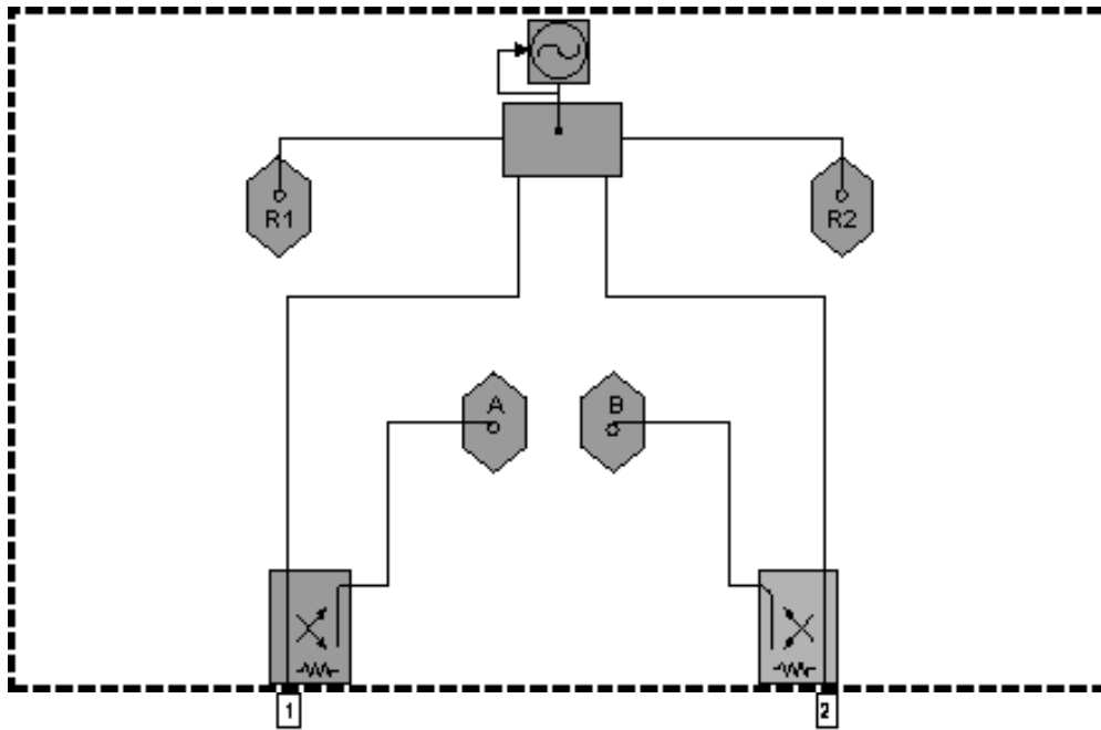
E8361A/C - Standard Configuration and Standard Power Range
