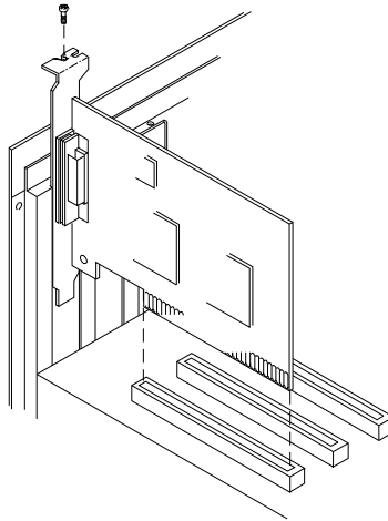
Figure 1-8 Replace the cover plate sscrew
