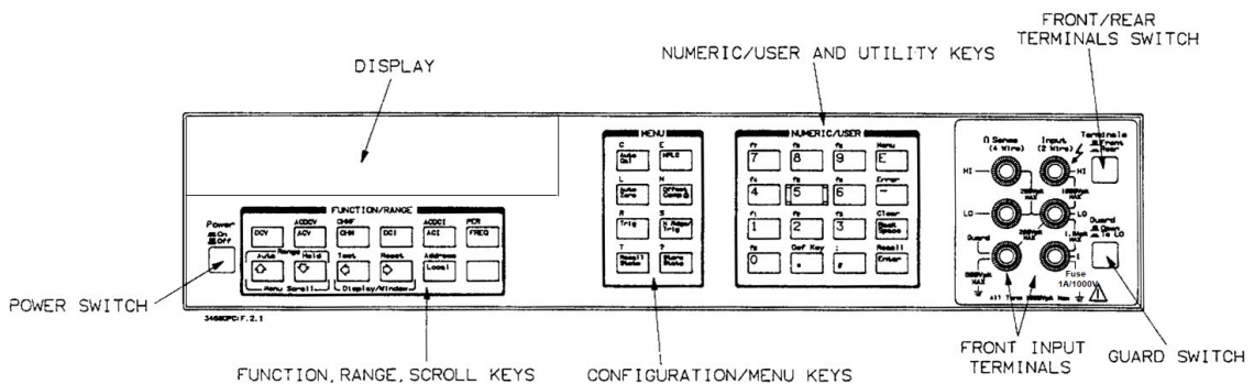
Figure 2-1 Front panel
