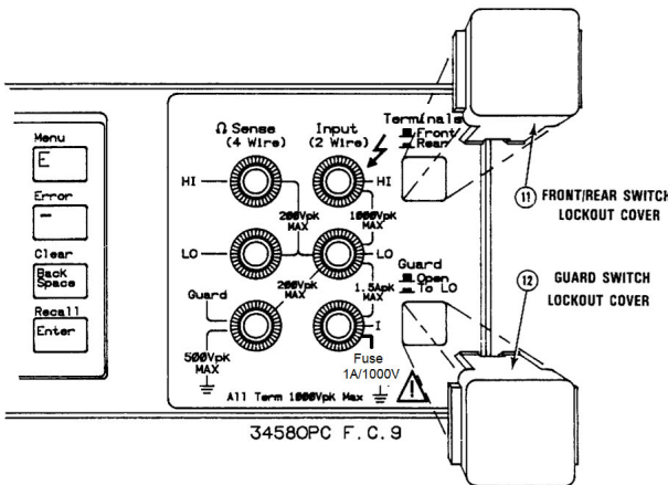
Figure C-9 Switch covers installation
