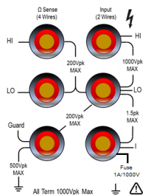
3458A Front Panel Terminal Area
