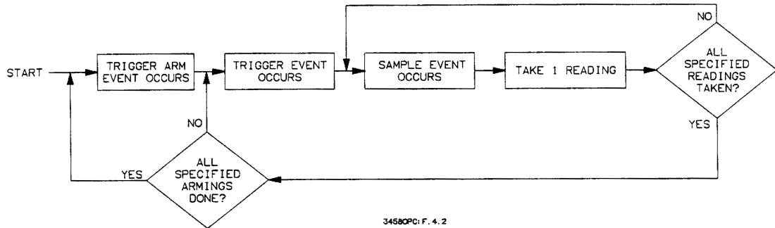
Figure 4-2 Multiple trigger arming
