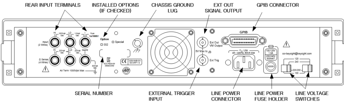
Figure 1-1 Rear panel
