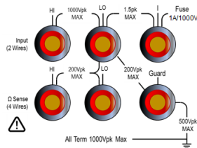
3458A Rear Panel Terminal Area
