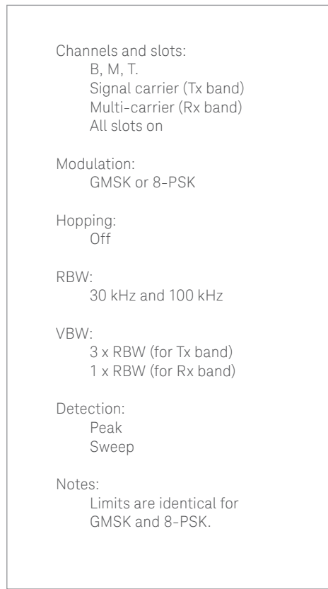
Figure 25. Tx and Rx band spurious, BTS, limits
