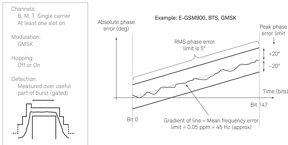
Figure 5. Phase error and mean frequency error, BTS, limits
