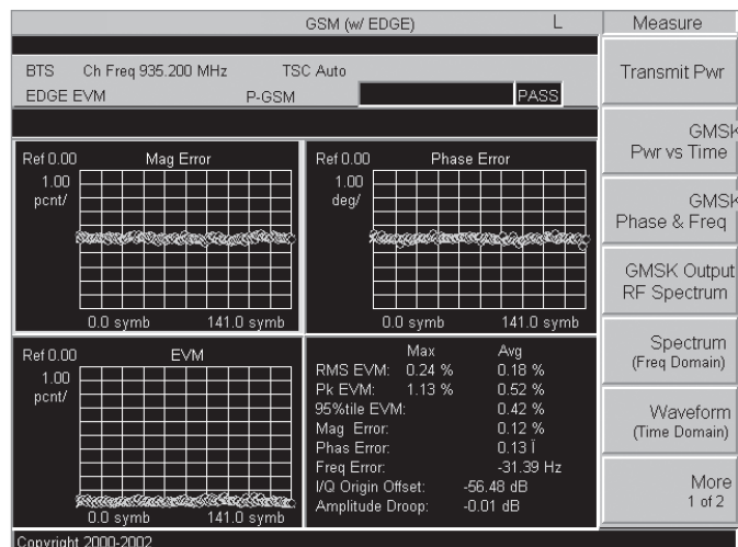
Figure 9. Quad display of the Keysight E4440A PSA series spectrum analyzer showing EDGE modulation metrics and separate magnitude and phase error
