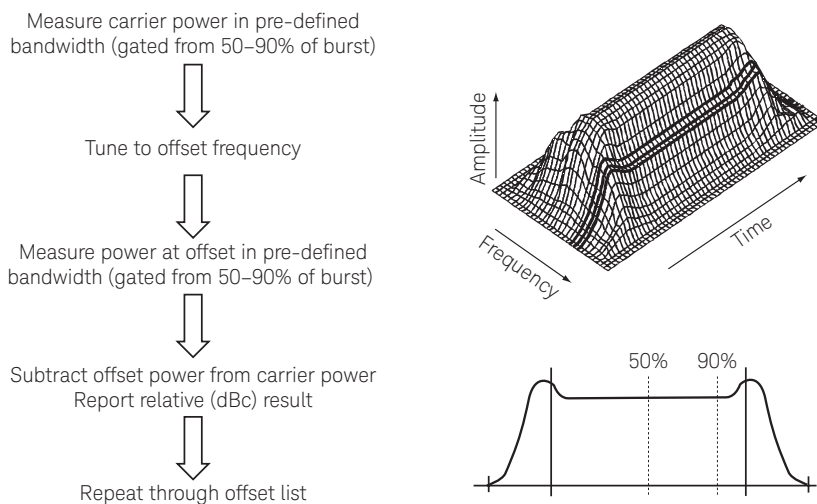
Figure 18. Theory of spectrum due to modulation and wideband noise
