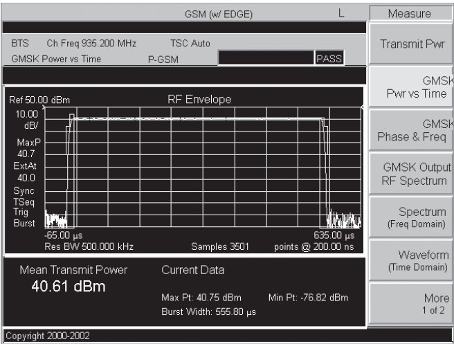
Figure 16. Power versus time on the Keysight E4440A PSA series spectrum analyzer. GSMK
