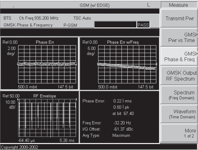
Figure 7. Quad display of the Keysight E4440A PSA series spectrum analyzer showing GMSK modulation metrics graphics of phase error with and without frequency error
