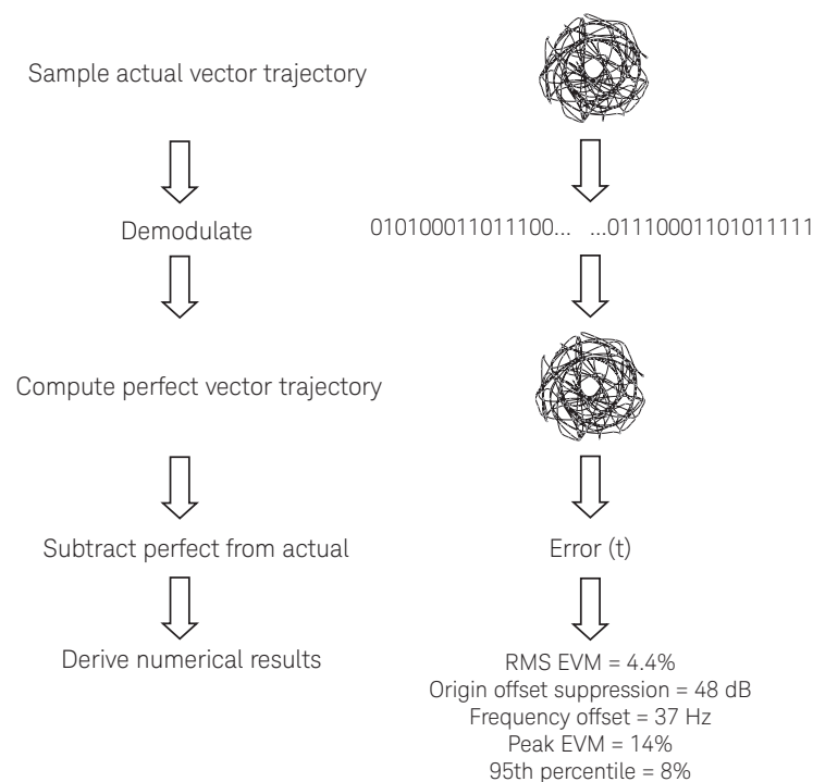
Figure 4. Theory of EVM, origin offset and frequency offset (8-PSK)
