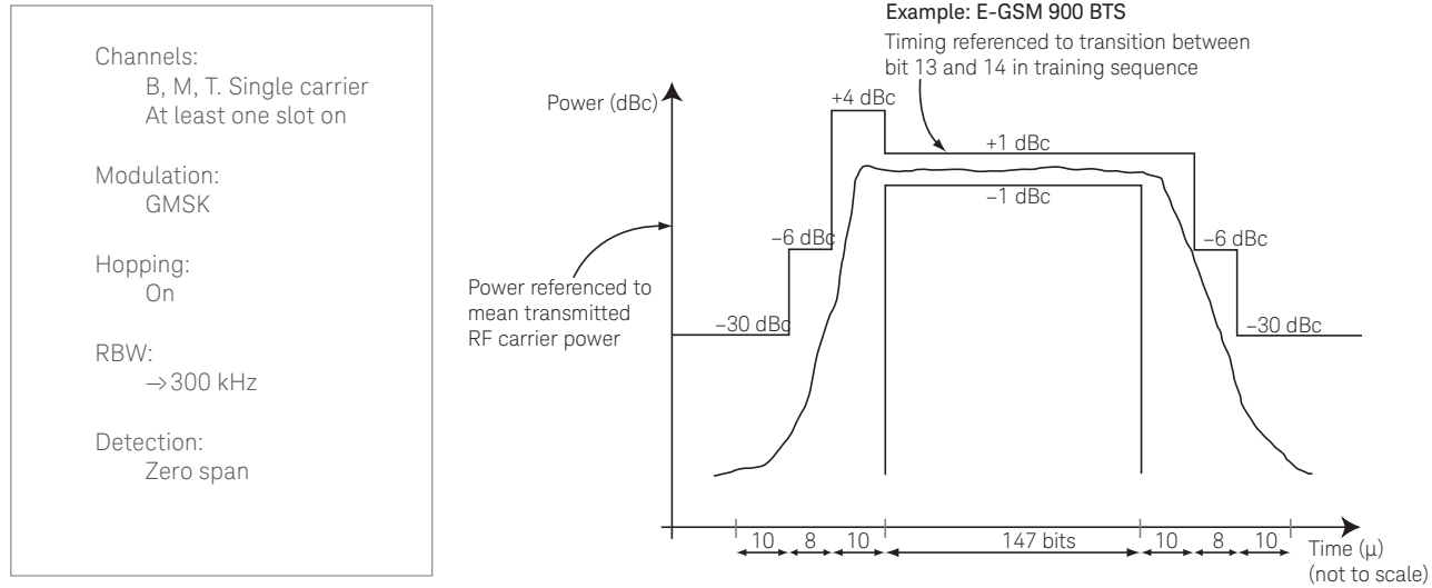
Figure 14. GMSK transmitted RF carrier power versus time, BTS, limits, GMSK
