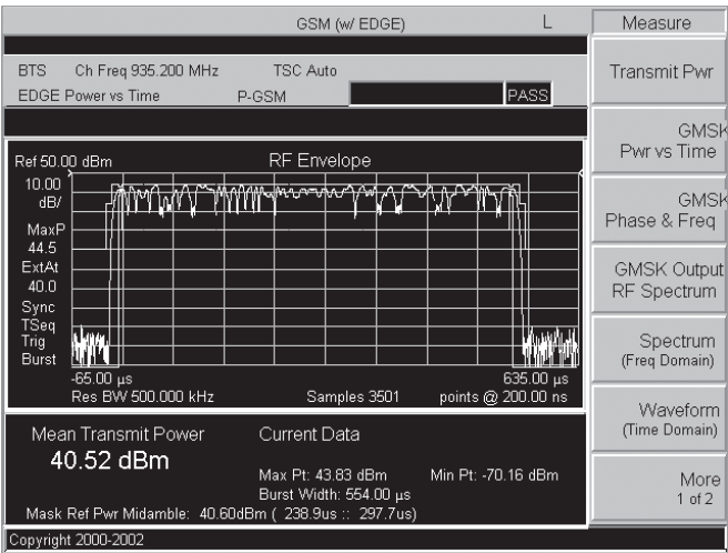
Figure 17. Power versus time on the Keysight E4440A PSA series spectrum analyzer. 8-PSK
