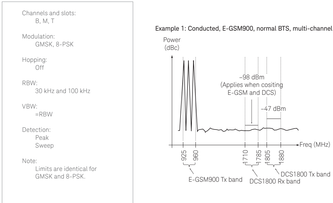
Figure 26. Cross-band spurious, GSM900 into DCS bands, BTS, limits
