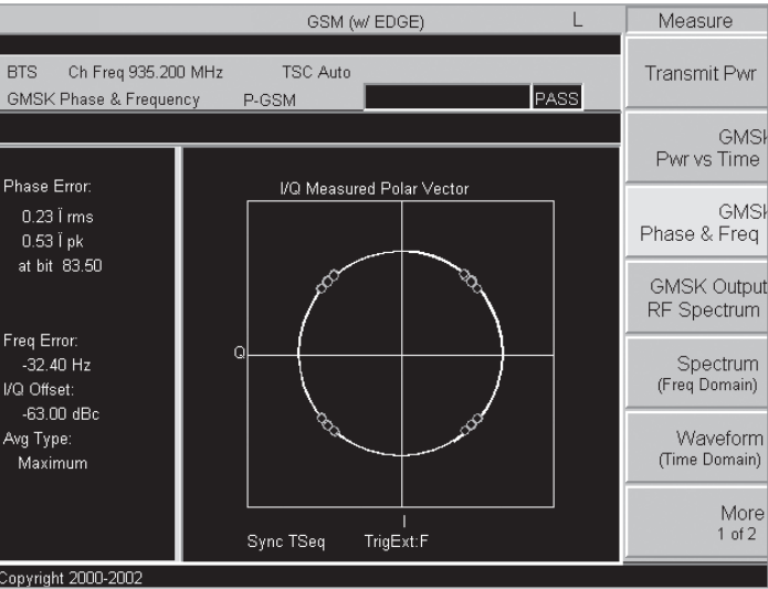
Figure 8. Constellation diagram on the Keysight E4440A PSA series spectrum analyzer showing GMSK modulation
