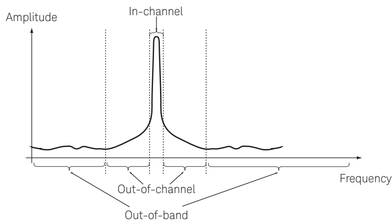
Figure 1. In-channel, out-of-channel, out-of-band measurements
