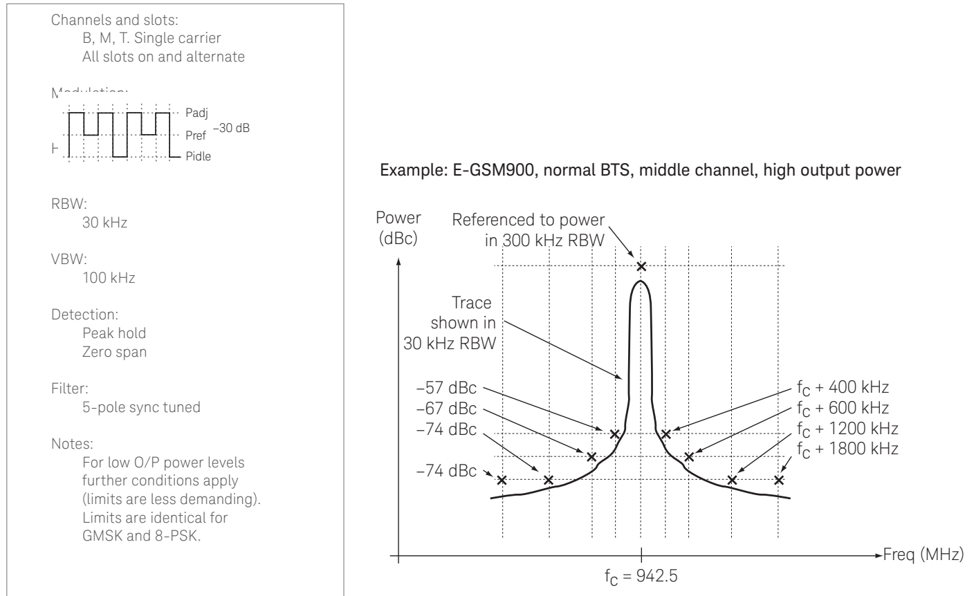
Figure 22. Spectrum due to switching, BTS, limits
