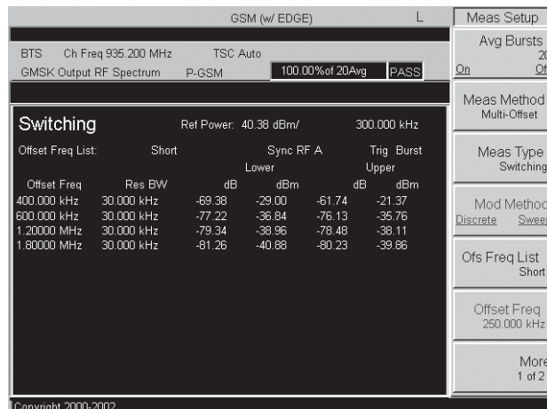
Figure 23. Spectrum due to switching shown on the Keysight E4440A PSA Series Spectrum Analyzer
