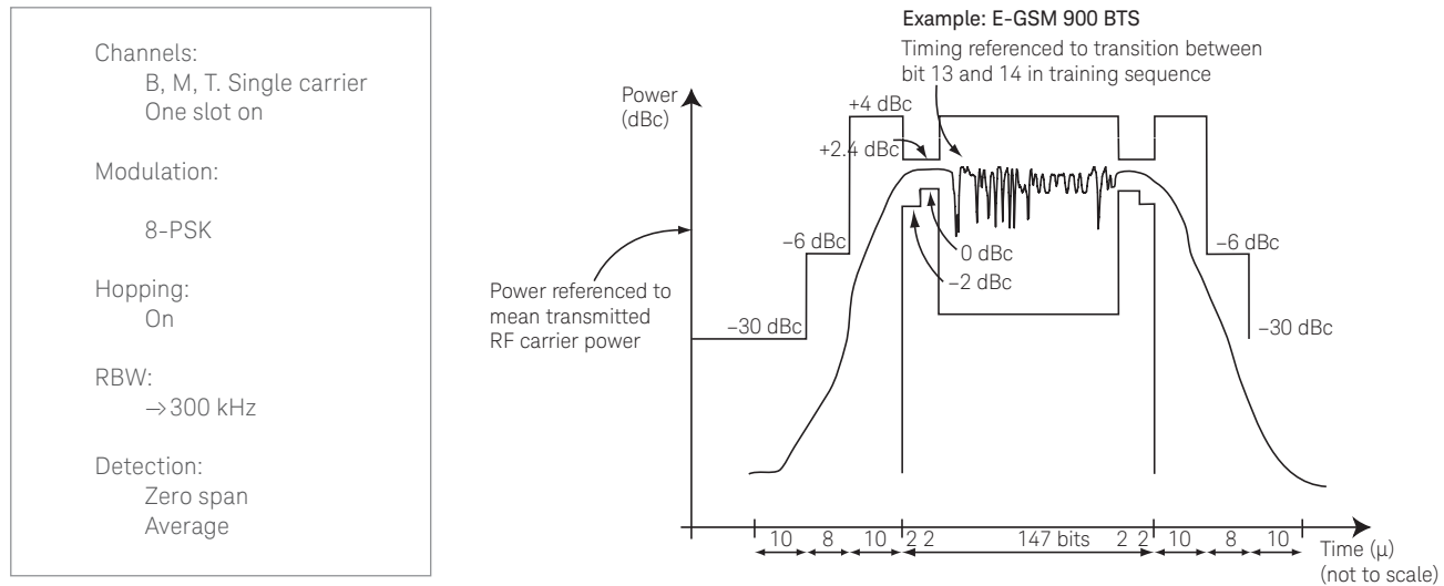
Figure 15. Transmitted RF carrier power versus time, BTS, limits: 8-PSK
