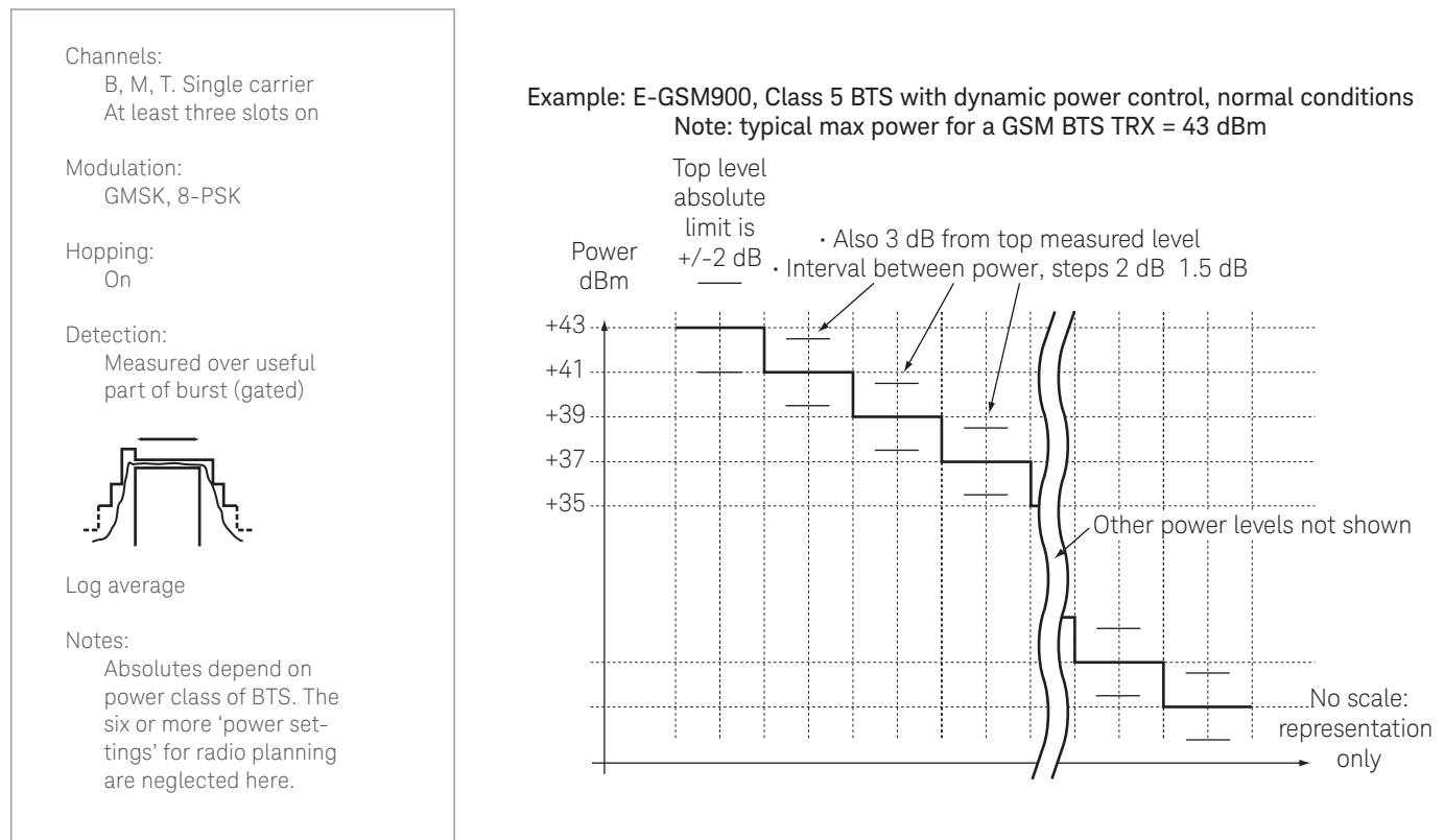
Figure 12. Mean transmitted RF carrier power, BTS, limits
