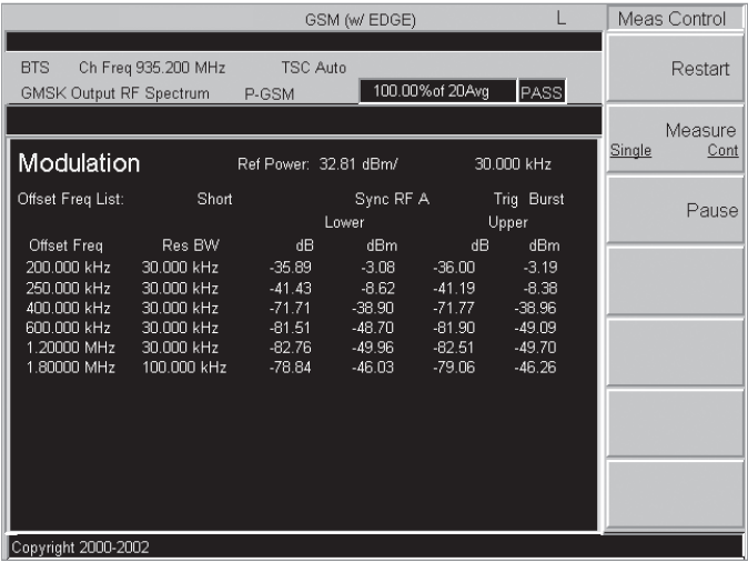
Figure 20. Spectrum due to modulation shown on the Keysight E4440A PSA series spectrum analyzer
