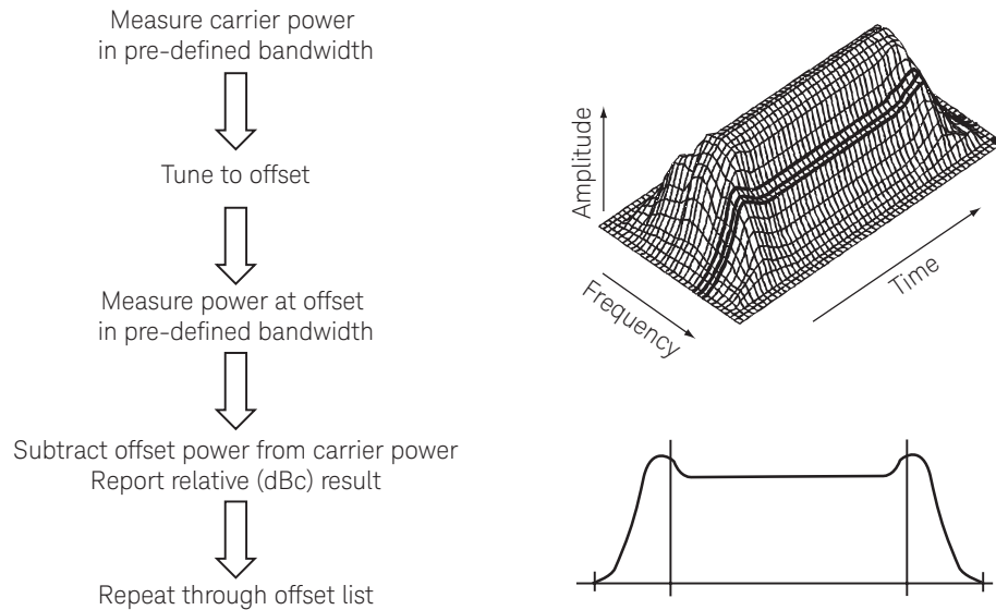
Figure 21. Theory of spectrum due to switching
