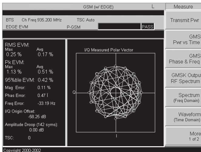
Figure 10. Constellation diagram on the Keysight E4440A PSA series spectrum analyzer showing EDGE/8-PSK modulation
