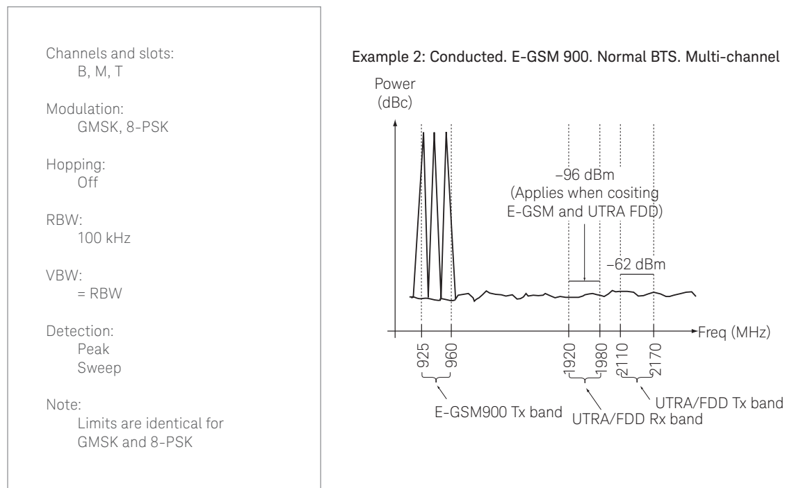
Figure 27. Cross band spurious. GSM900 into 3G bands, BTS, limits
