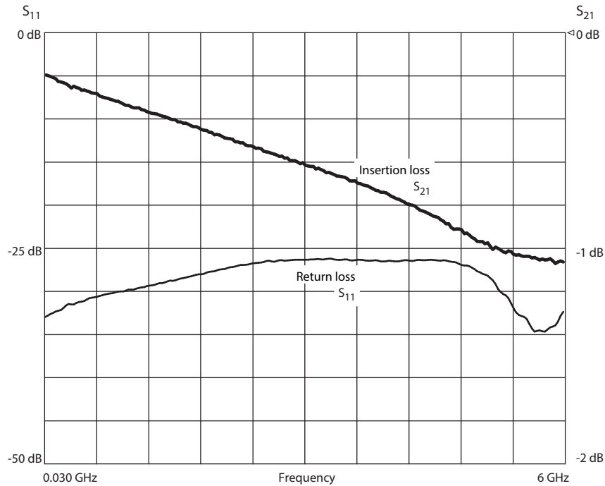
Figure 2. 11930A typical insertion and return loss versus frequency
