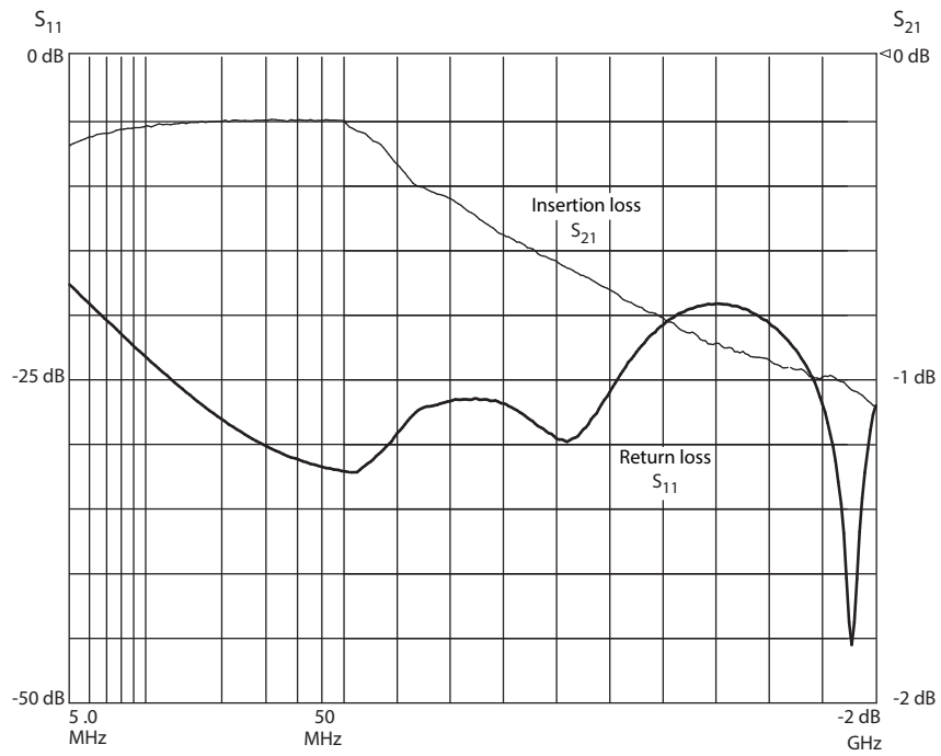
Figure 3. 11930B typical insertion and return loss versus frequency
