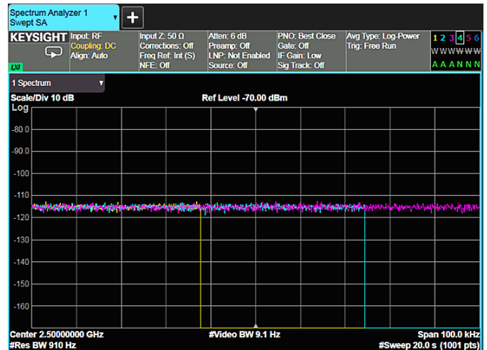
Figure 2-30b. Average detection mode: noise level remains constant, regardless of VBW-to-RBW ratios (3:1, 1:10 and 1:100).
