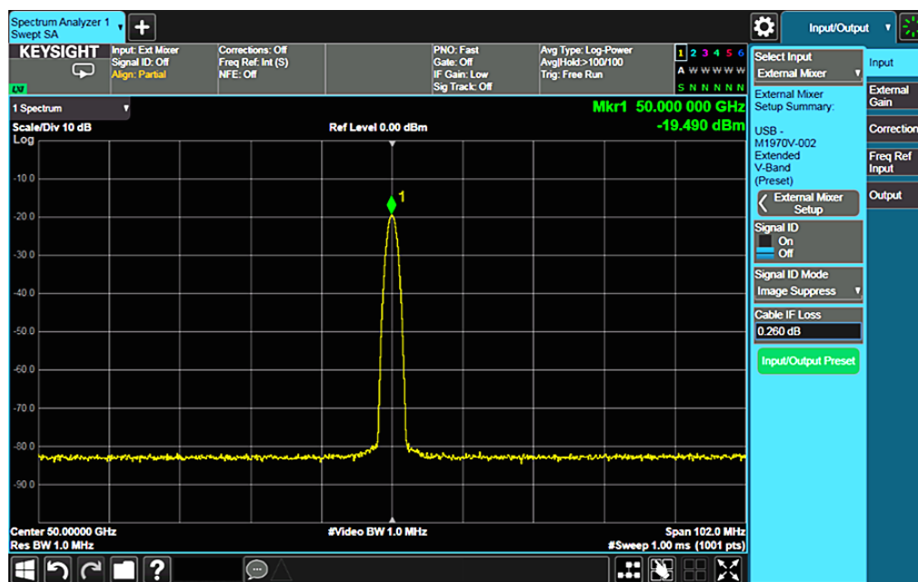
Figure 7-19. Measurement of a positively identified signal
