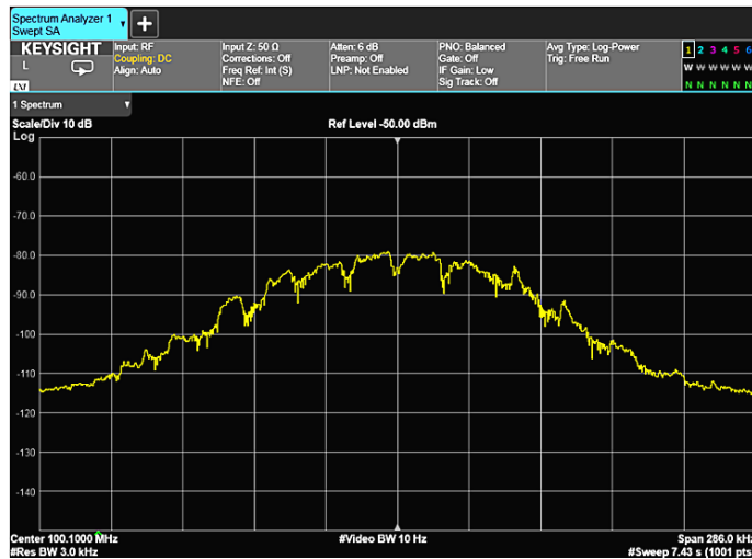
Figure 2-32a. Video filtering
