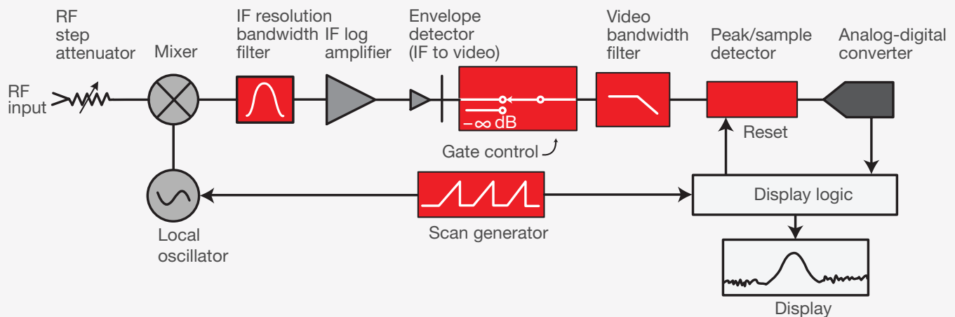
Figure 2-42. Block diagram of a spectrum analyzer with gated video
