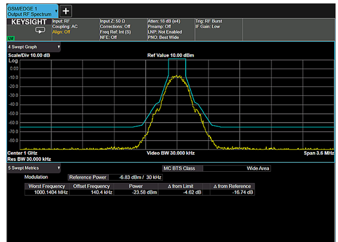
Figure 1-4. GSM radio signal and spectral mask showing limits of unwanted emissions
