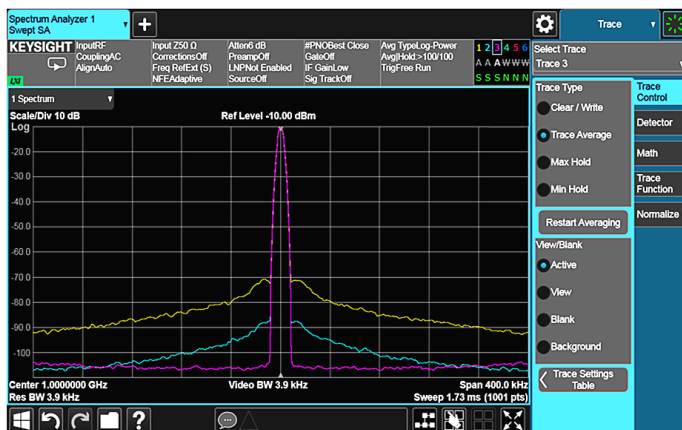
Figure 2-12a. Phase noise performance can be optimized for different measurement conditions
