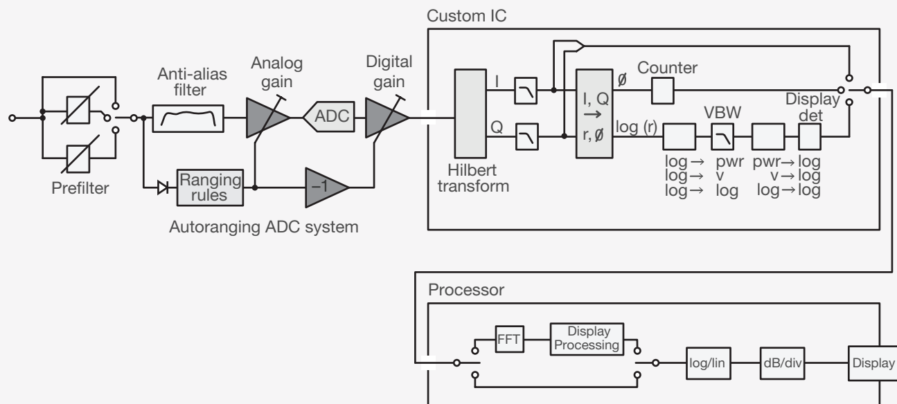
Figure 3-2. Block diagram of the all-digital IF in the Keysight X-Series signal analyzers
