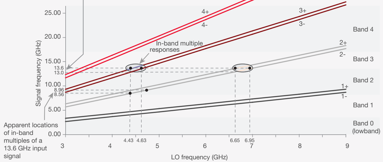
Figure 7-5. Tuning curves up to 4th harmonic of LO showing in-band multiple responses to a 13.6-GHz input signal
