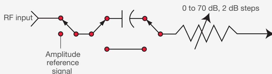
Figure 2-3. RF input attenuator circuitry
