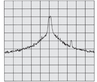
Figure 2-33b. Frequency spectrum of combined signals. Which radio produces the spurious emissions?
