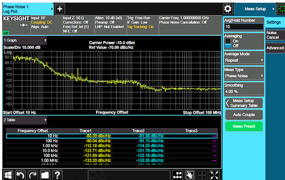
Figure 8-3. Phase noise measurement
