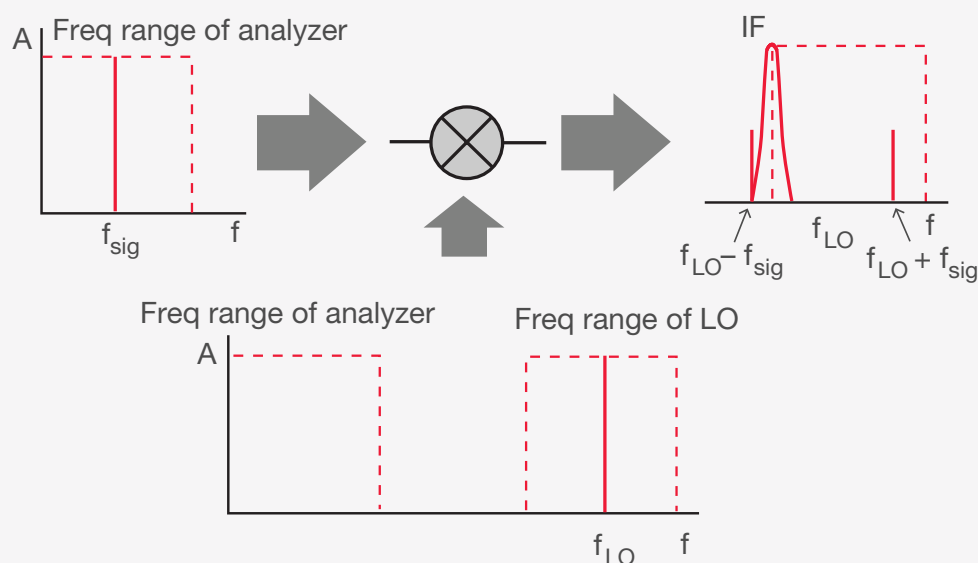
Figure 2-4. The LO must be tuned to f_{IF} + f_{sig} to produce a response on the display
