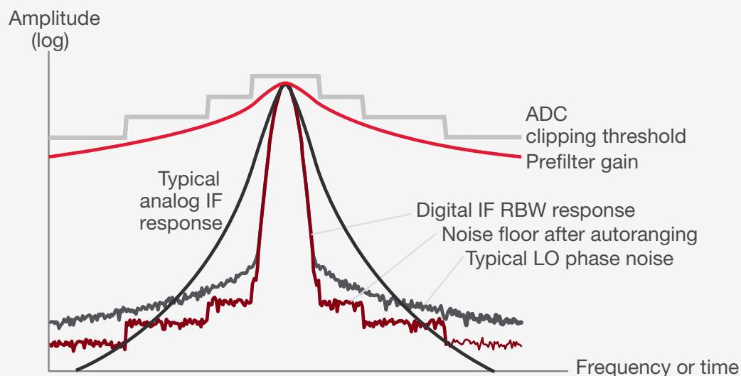
Figure 3-3. Autoranging keeps ADC noise close to the carrier and lower than LO noise or RBW filter response
