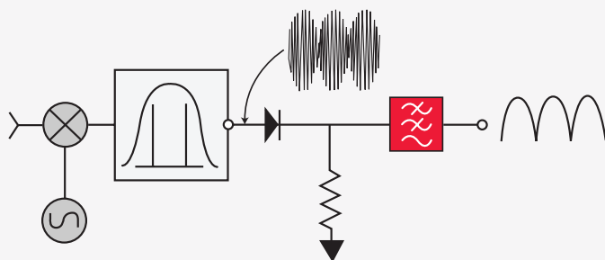
Figure 2-16b. Output of the envelope detector follows the peaks of the IF signal
