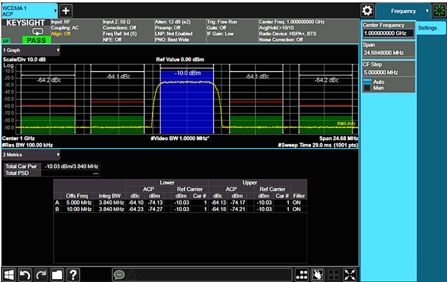
Figure 6-9. Adjacent channel power measurement using a high-performance X-Series signal analyzer
