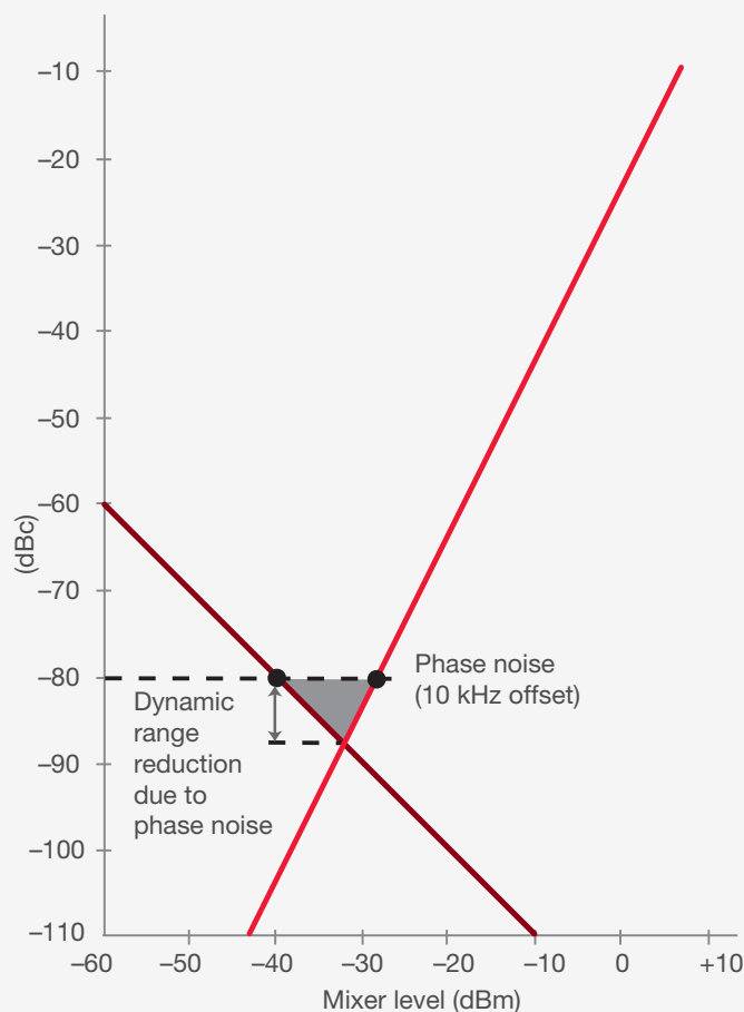
Figure 6-4. Phase noise can limit third-order intermodulation tests
