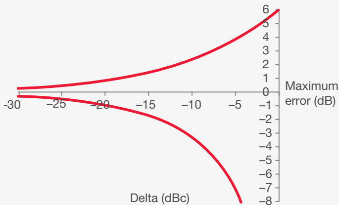
Figure 6-5. Uncertainty versus difference in amplitude between two sinusoids at the same frequency
