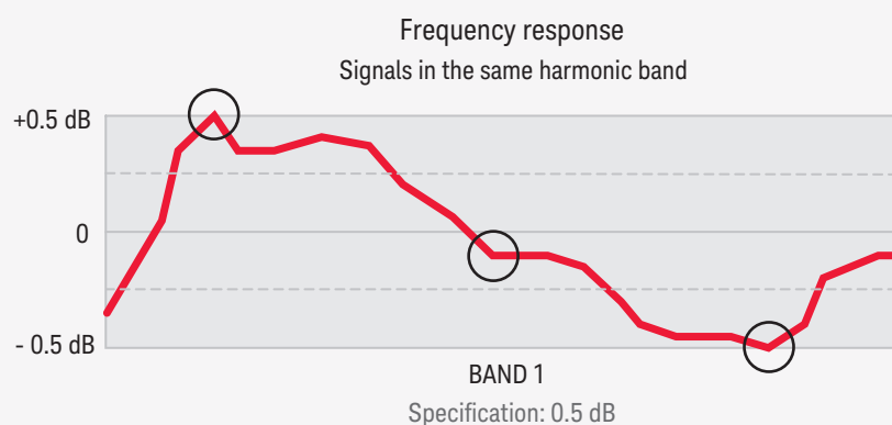
Figure 4-2. Relative frequency response in a single band
