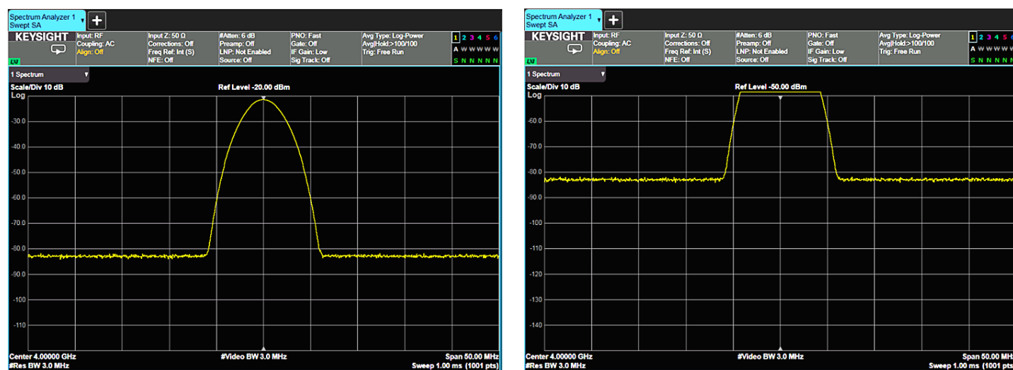
Figure 6-8. Display range and measurement range on a high-performance X-Series signal analyzer
