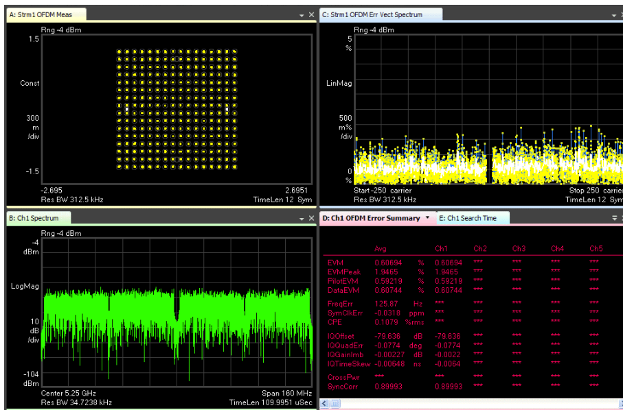
Figure 8-5. Modulation analysis of WLAN 802.11ac signal using Keysight 89600 VSA software
