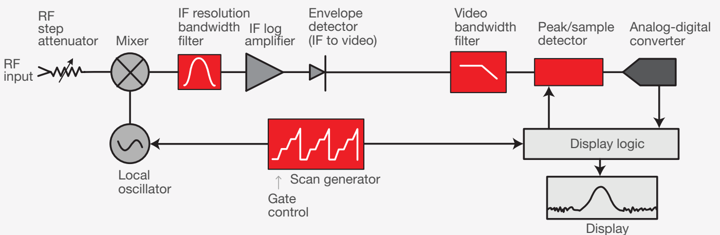
Figure 2-40. In gated LO mode, the LO sweeps only during gate interval
