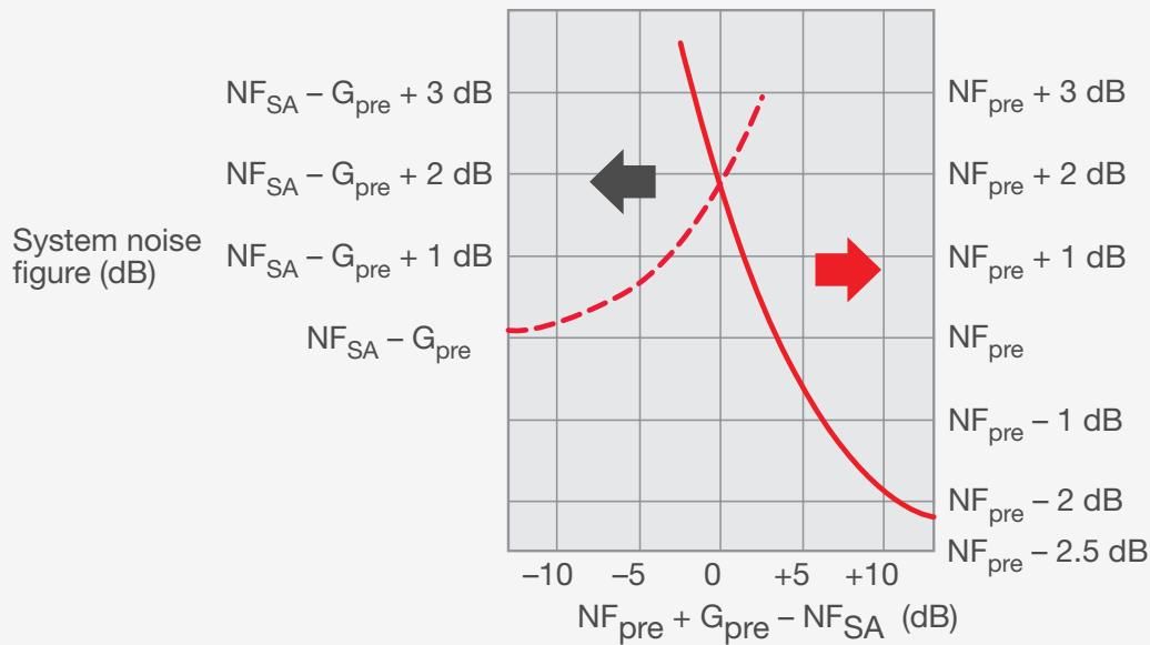
Figure 5-6. System noise figure for sinusoidal signals
