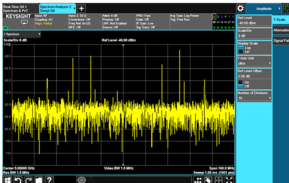
Figure 8-7 . Even when you use fast sweeps and max hold over a period of many seconds, the swept spectrum analyzer view of the radar signal is not very informative
