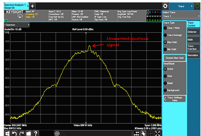
Figure 2-37. Frequency domain view of the GSM signal with 2 time slots “on” showing an unwanted spurious signal present in the spectrum.
