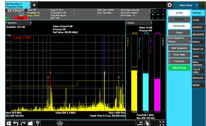
Figure 1-6. Radiated emissions plotted against CISPR11 limits as part of an EMI test
