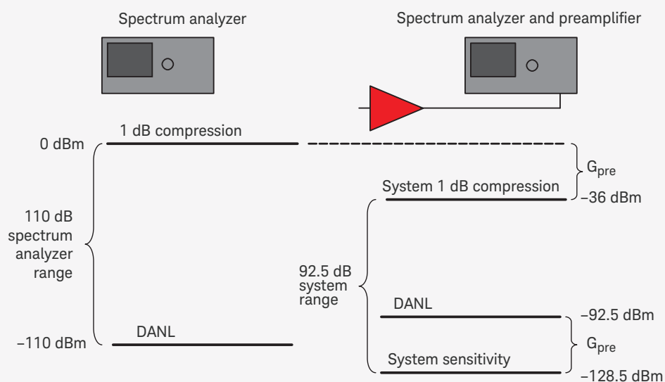
Figure 5-5. If displayed noise goes up when a preamplifier is connected, measurement range is diminished by the amount the noise changes
