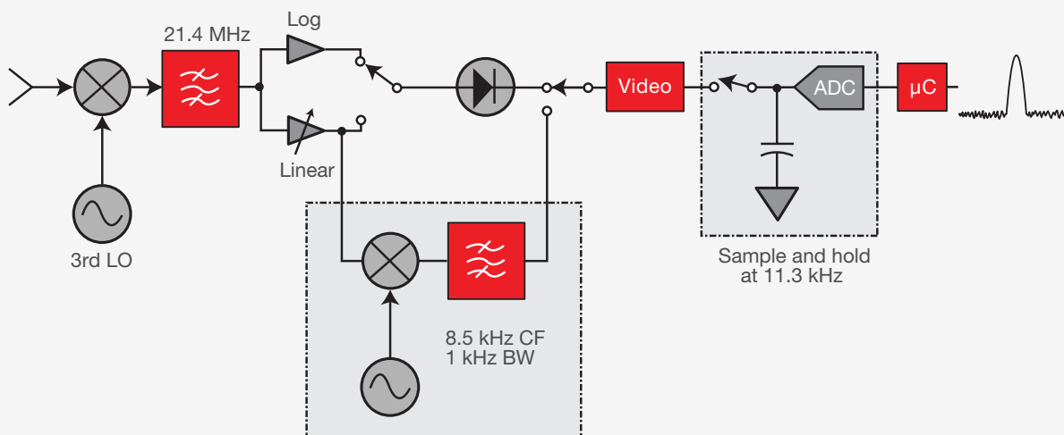
Figure 3-1. Digital implementation of 1-, 3-, 10-, 30-, 100- and 300-Hz resolution filters in ESA-E Series spectrum analyzers
