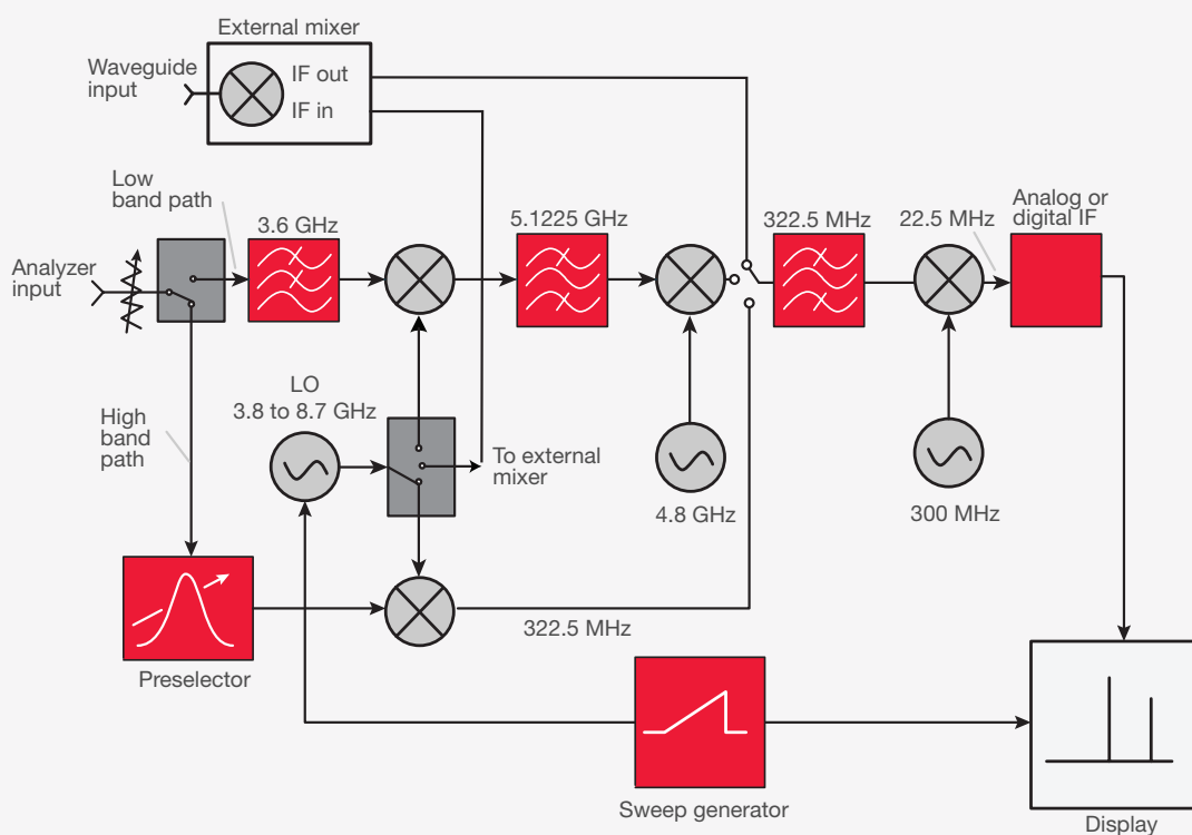
Figure 7-14. Spectrum analyzer and external mixer block diagram
