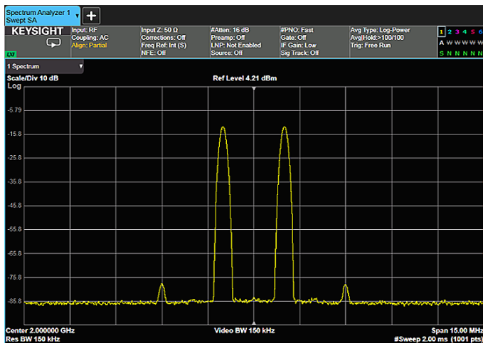
Figure 1- 5. Two-tone test on an RF power amplifier
