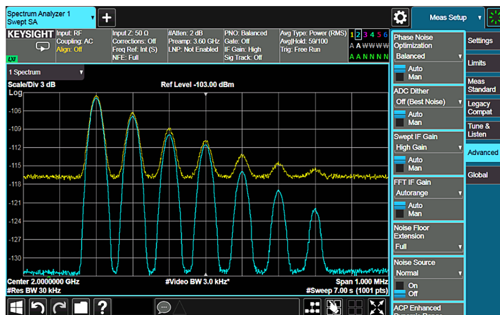
Figure 5-4. Noise floor extension view of harmonics
