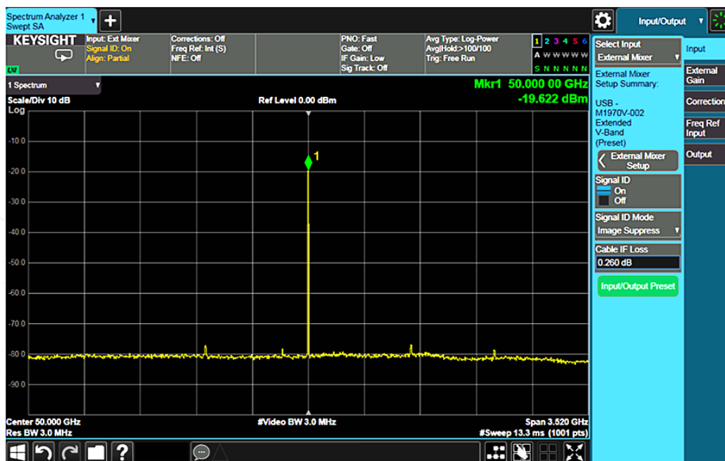
Figure 7-18. The image suppress function displays only real signals
