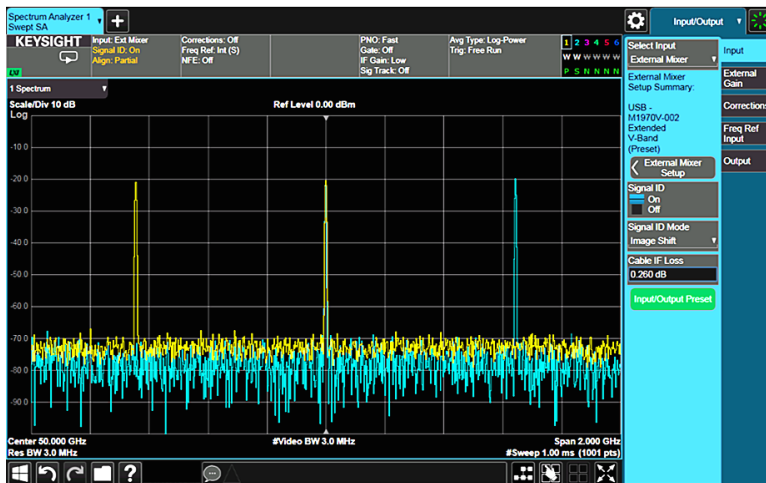
Figure 7-17a: 6 - centered (yellow trace)
