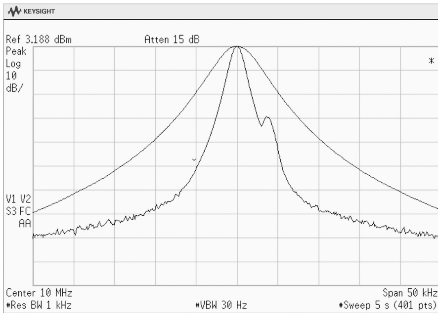
Figure 2-10. The 3-kHz filter (top trace) does not resolve the smaller signal; reducing the resolution bandwidth to 1 kHz (bottom trace) does resolve the smaller signal
