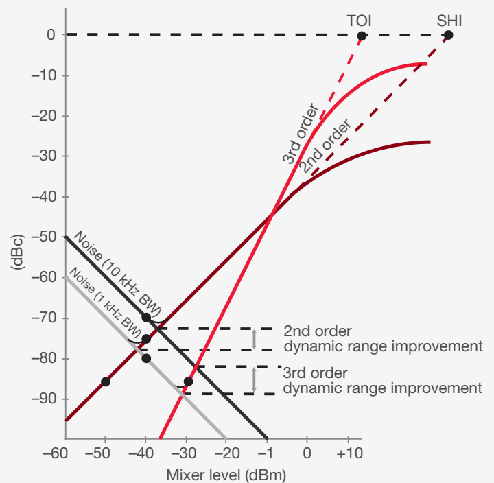
Figure 6-3. Reducing resolution bandwidth improves dynamic range
