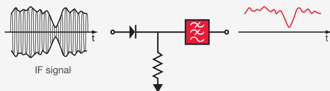
Figure 2-16a. Envelope detector
