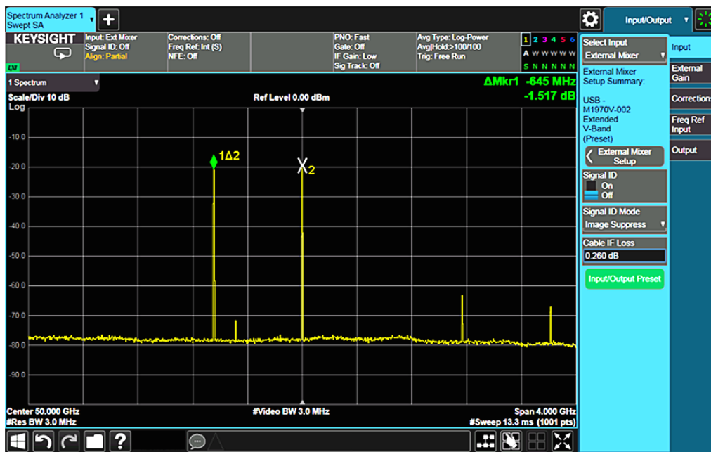
Figure 7-15. Which ones are the real signals?
