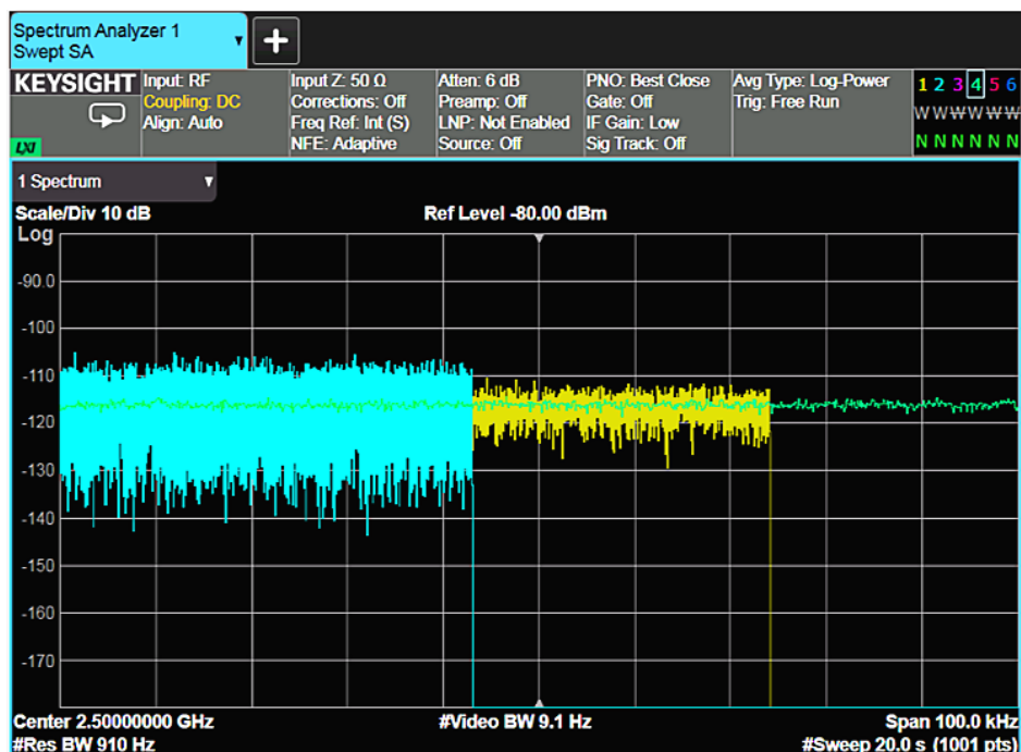
Figure 2-29. Smoothing effect of VBW-to-RBW ratios of 3:1, 1:10, and 1:100
