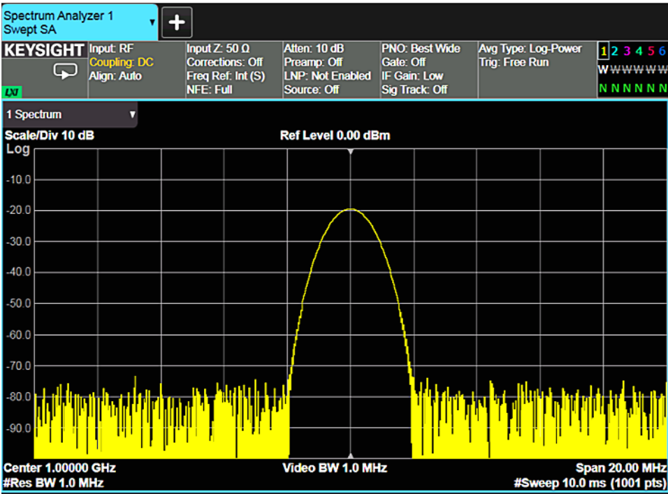
Figure 2-24. Normal detection displays maximum values in buckets where the signal only rises or only falls
