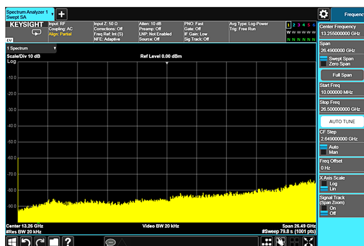
Figure 2-15a. Full span sweep speed, RBW of 20 kHz, without Option FS1
