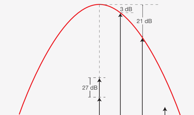
Figure 7-13. Improved third-order intermodulation distortion; test tone separation is significant relative to preselector bandwidth
