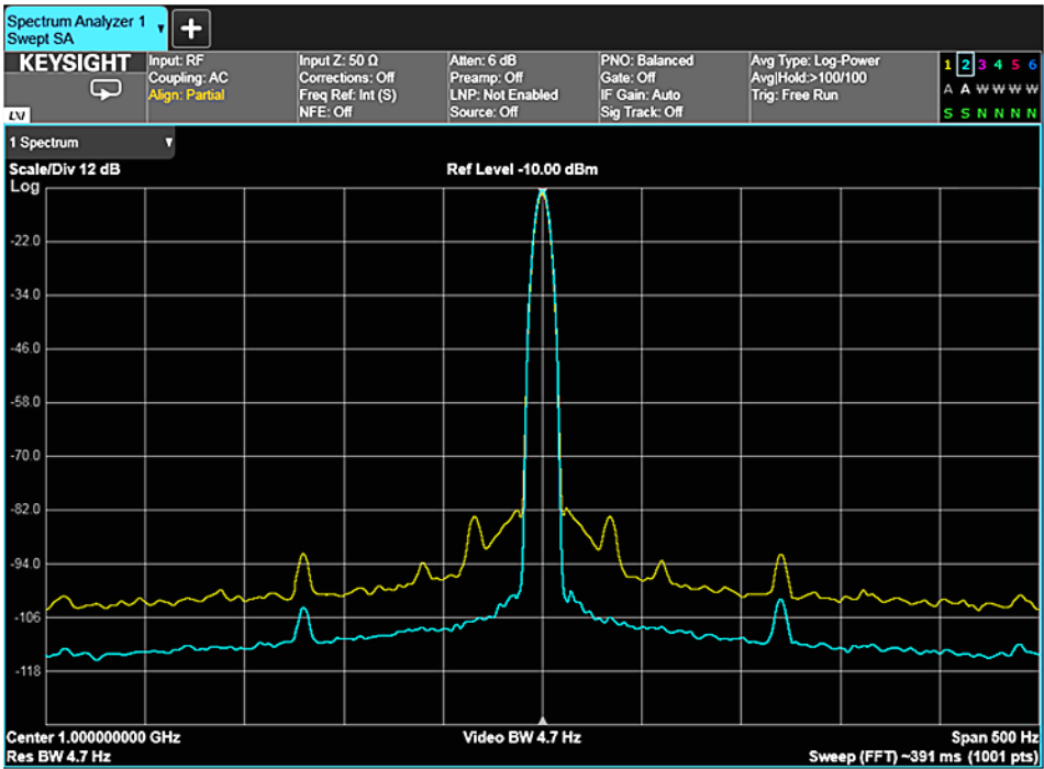
Figure 7-11. Phase noise levels for fundamental and 4th harmonic mixing
