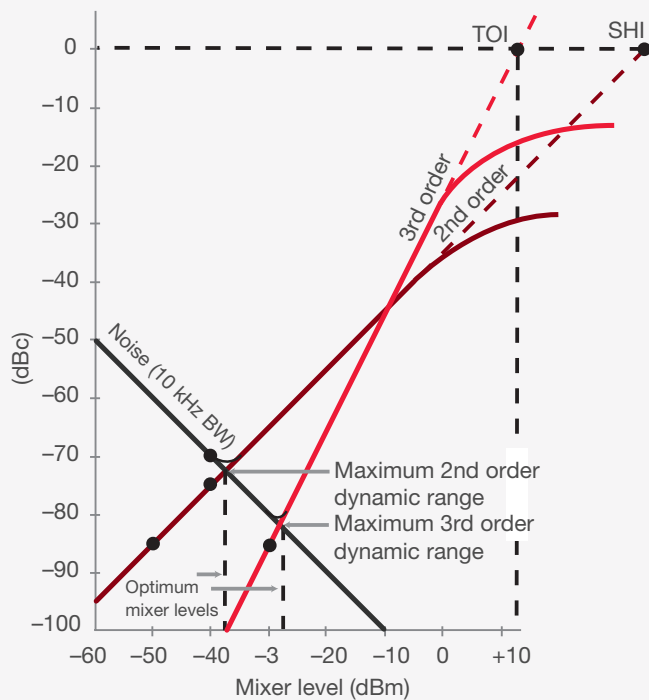
Figure 6-2. Dynamic range versus distortion and noise
