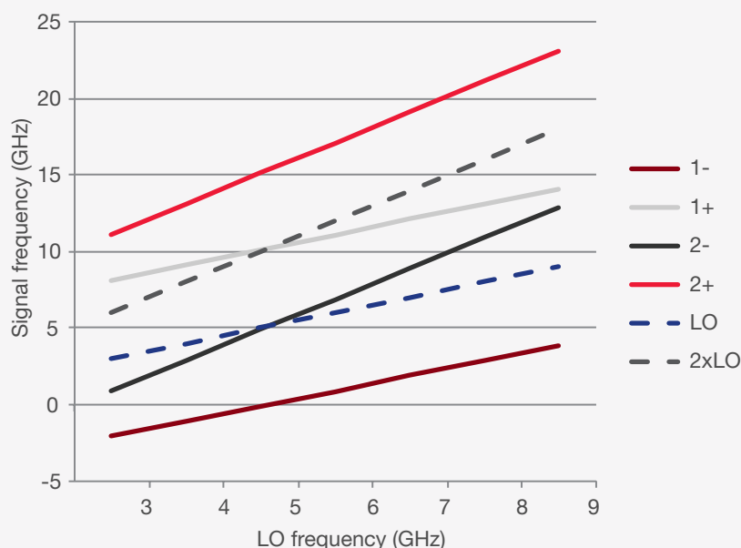
Figure 7-3. Signals in the “1 minus” frequency range produce single, unambiguous responses in the low-band, high-IF case
