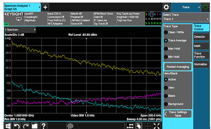
Figure 2-12b. Detail of the 140-kHz carrier offset region
