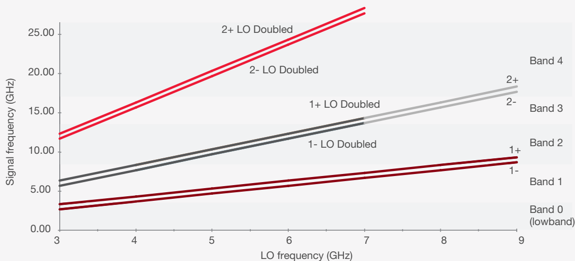
Figure 7-7. X-Series analyzer harmonic bands using LO doubling
