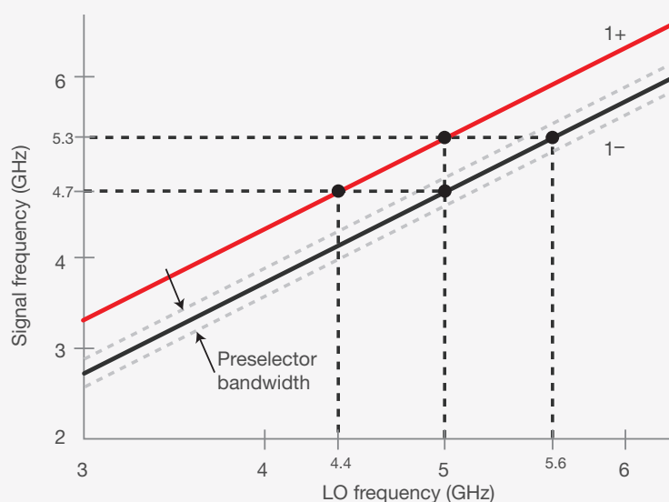
Figure 7-8. Preselection; dashed gray lines represent bandwidth of tracking preselector
