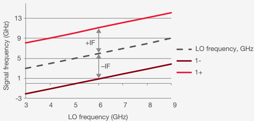
Figure 7-2. Tuning curves for fundamental mixing in the low band, high IF case
