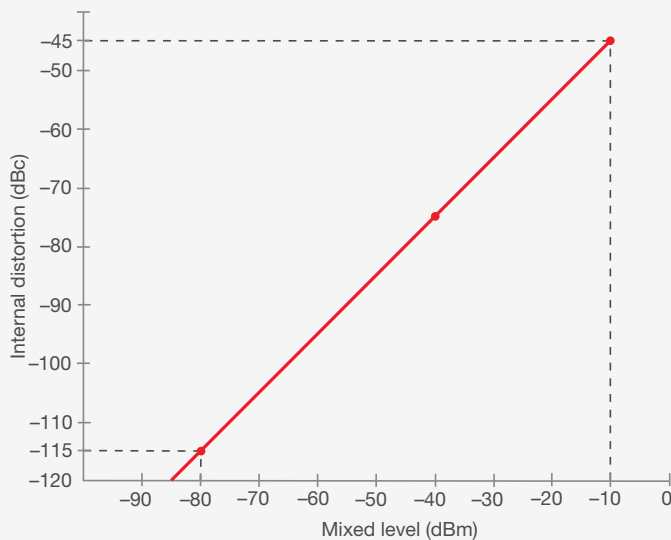
Figure 7-12. Second-order distortion graph
