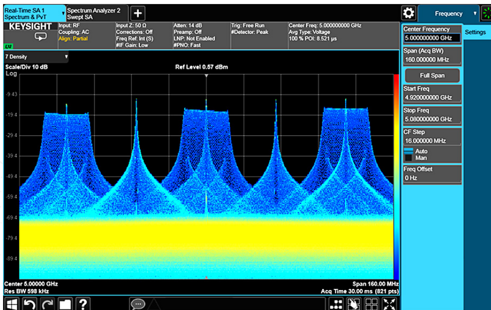
Figure 8-8. Real-time capture of two C-band acquisition radar signals.
