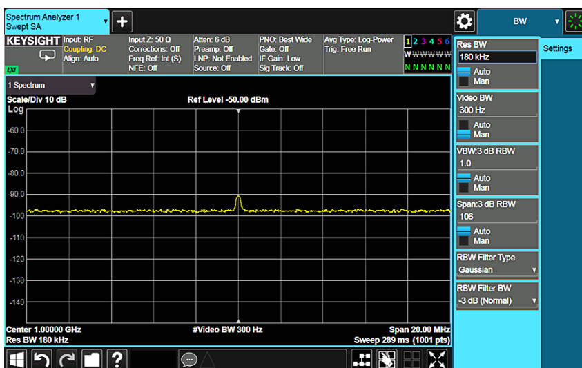
Figure 5-3. Video filtering makes low-level signals more discernible
