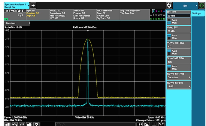
Figure 5-2. Displayed noise level changes as 10 \log (BW_2 / BW_1)
