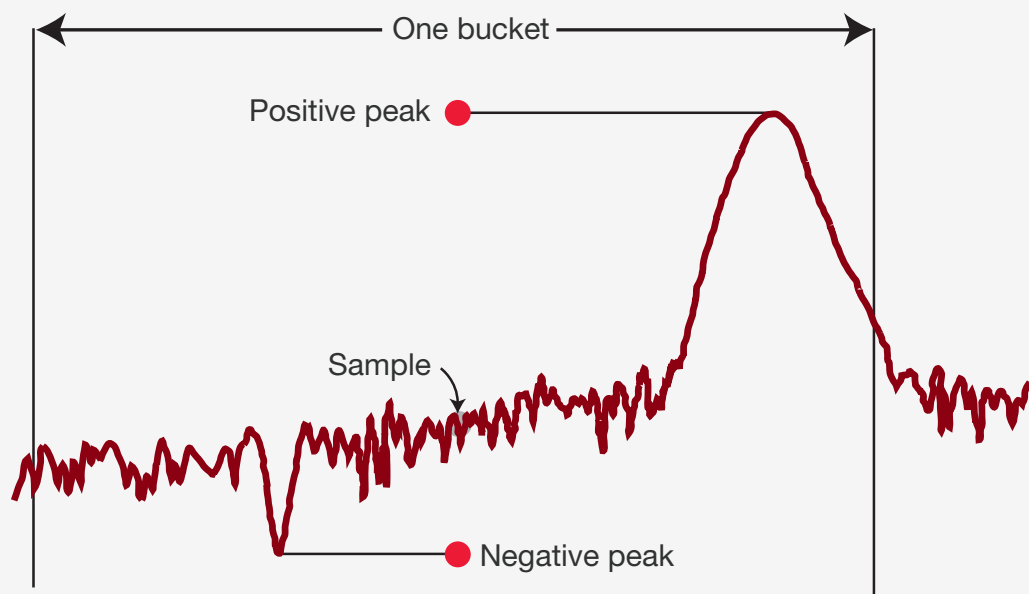
Figure 2-18. The trace point saved in memory is based on the detector type algorithm
