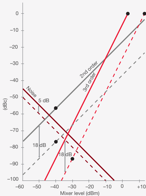
Figure 6-6. Dynamic range for 1.3-dB maximum error
