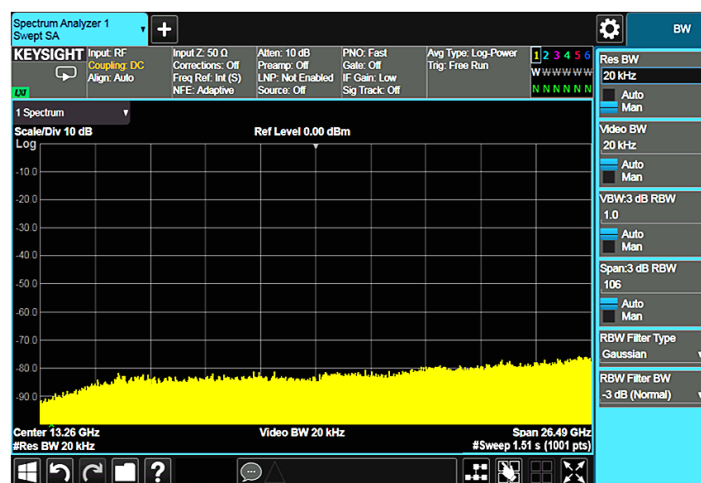
Figure 2-15b. Full span sweep speed, RBW of 20 kHz, with Option FS1
