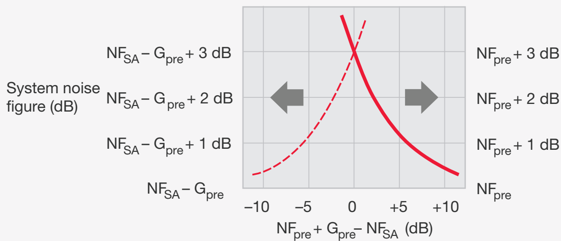
Figure 5-9. System noise figure for noise signals
