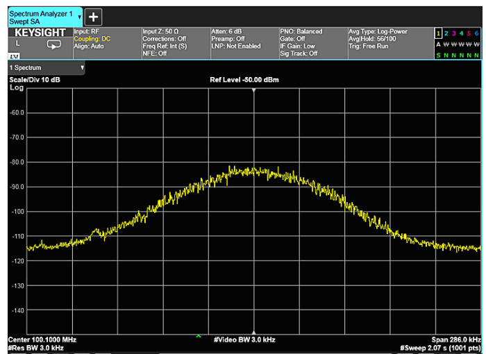
Figure 2-32b. Trace averaging
