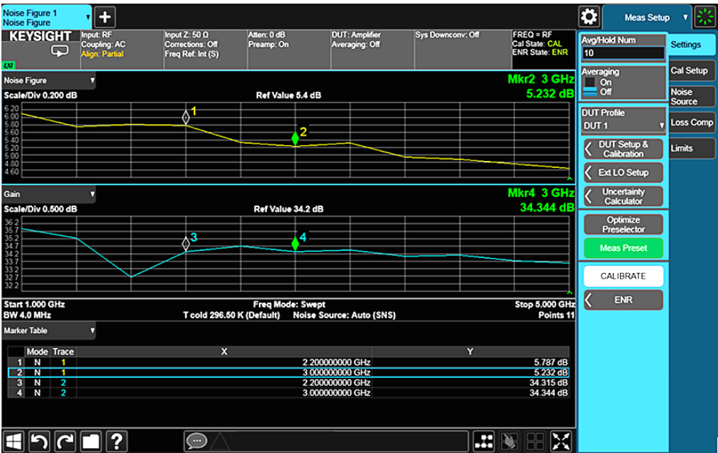
Figure 8-2. Noise figure measurement
