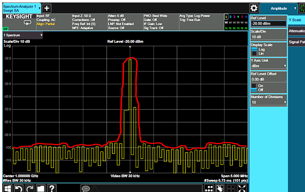
Figure 2-26. Normal detection can show two peaks when only one peak actually exists
