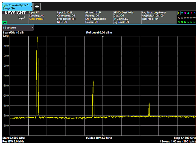
Figure 1-3. Harmonic distortion test of a transmitter
