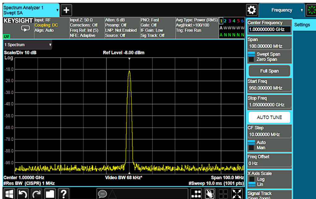
Figure 2-17. Each of the 1001 trace points (buckets) covers a 100-kHz frequency span and a 0.01-millisecond time span
