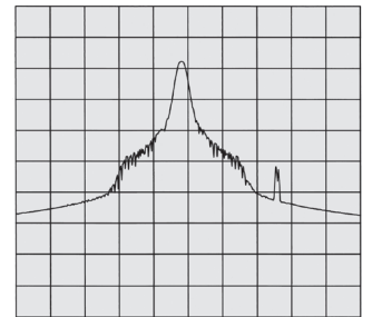
Figure 2-33c. The time-gated spectrum of signal #1 identifies it as the source of spurious emission
