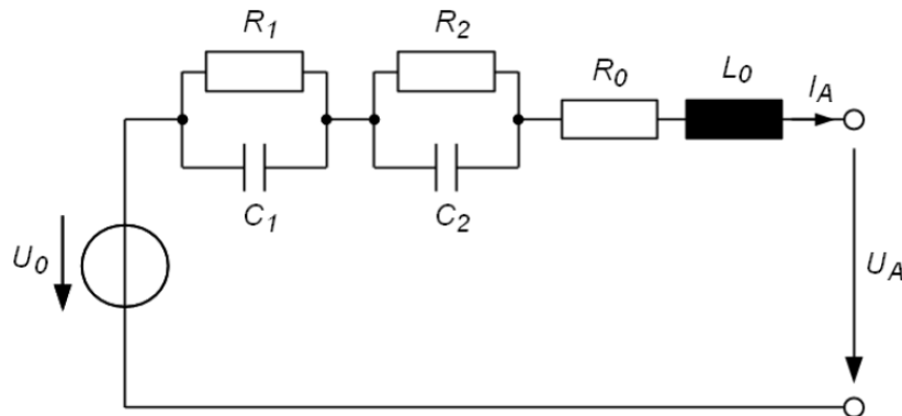
Figure 2: Battery model
