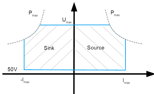
Figure 3: Max. power of 50 V to U_{max} (2 quadrant system).
