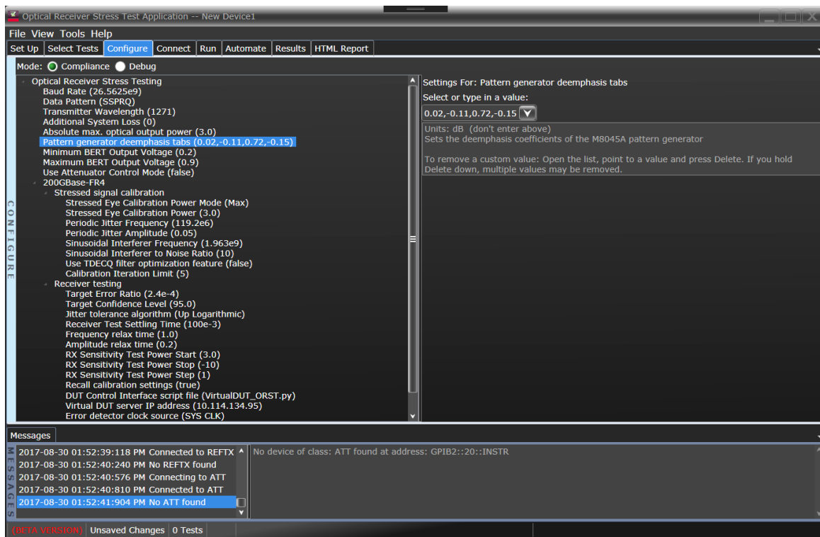
Figure 6. The N4917BSCA software Configure tab lets the user fine-tune the standard compliant stressed receiver test or adapt to the test to other standards by offering multiple, user-editable settings, such as the stress signal parameters or test conformance limits.
