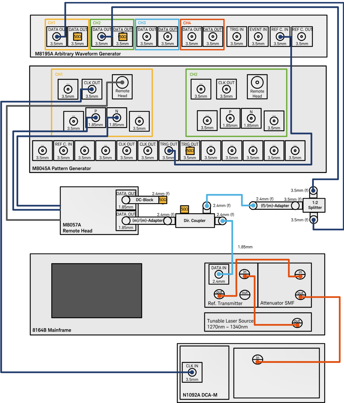
Figure 8. Setup for stressed eye signal calibration for 200 GBASE-FR4/-LR4/-DR4 and 400 GBASE-FR8/LR8 with clean clock.
