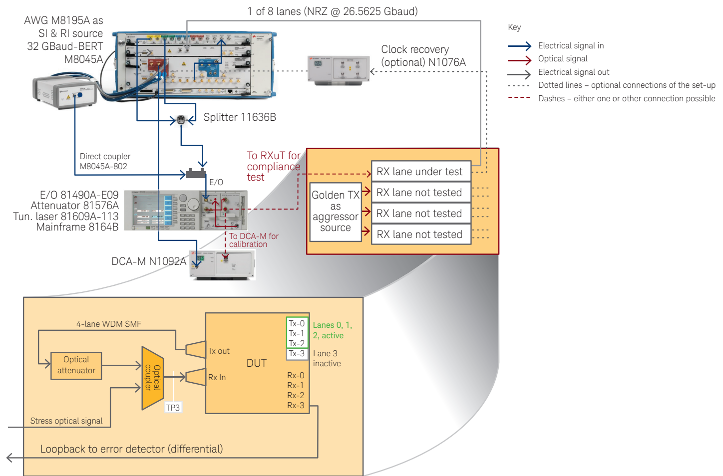
Figure 2. Optical receiver stress test setup for 200 GBASE-LR4/-FR4.
