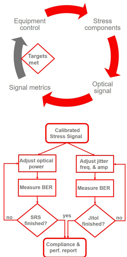
Figure 1. Calibration process and performance test steps as carried out by the N4917BSCA software.
