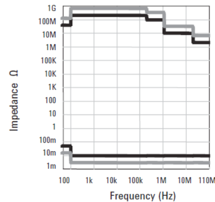
Impedance measurement range (typical)
