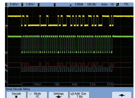
View on-screen serial decode of an I 2 C packet.
