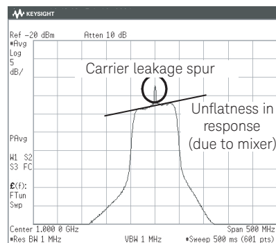
Figure 35. An example of poor PSD flatness.
