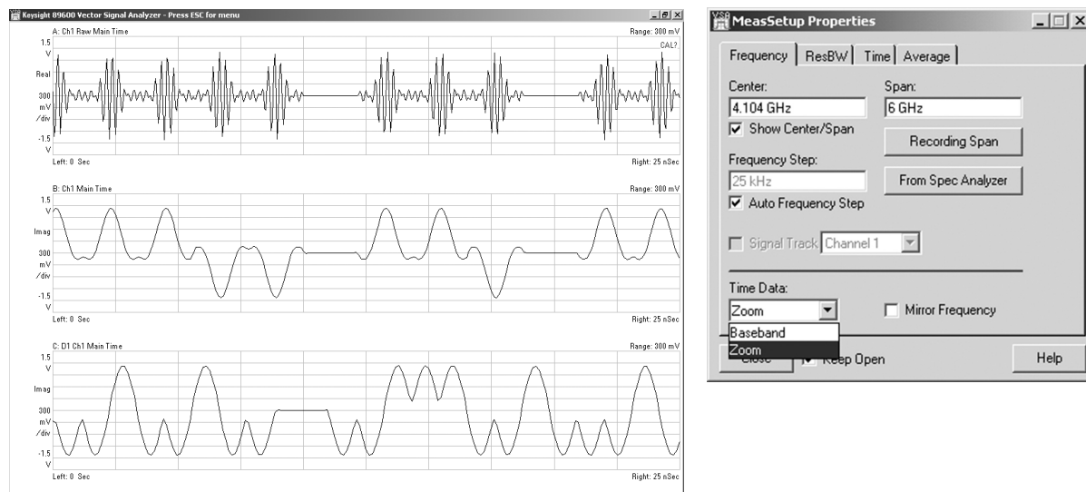
Figure 8. 89601A Vector Signal Analyzer software using Zoom (Demodulation) mode to show both the time (voltage) waveform of pulsed RF signal, and the recovered pulse shape.
