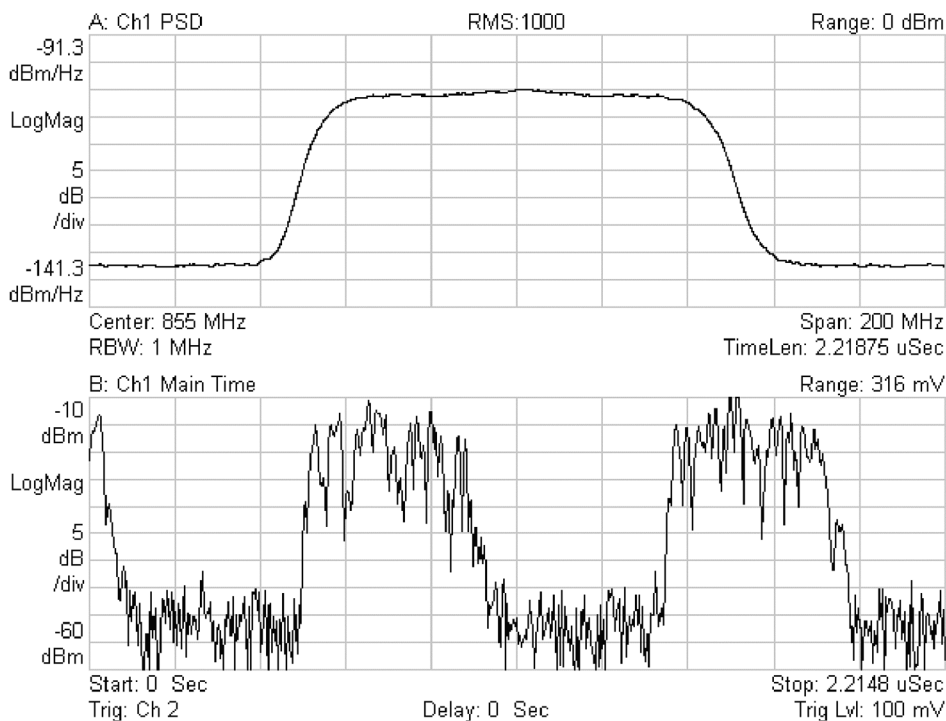
Figure 17. Pulsed noise spectrum and time (linear magnitude) displays.
