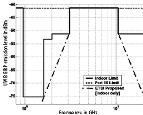
Figure 48a. Indoor FCC and proposed ETSI spectrum masks.
