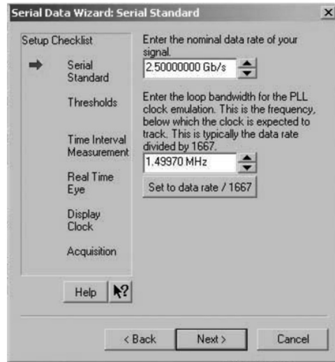
Figure 49b. Setup window for the software clock recovery application.
