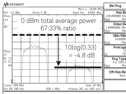
Figure 37. Frequency switched signal 67:33 ratio.
