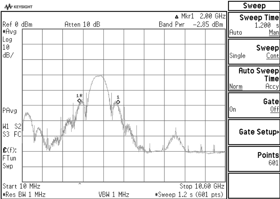
Figure 43. Mixed noise and spurious average detection.
