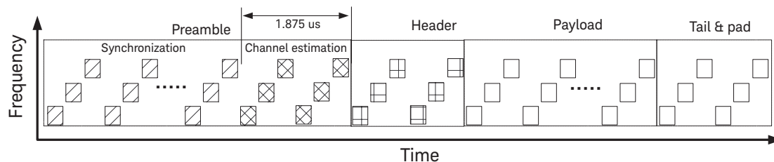
Figure 60. Sequence of symbols in the Mode 1 MB-OFDM packet.
