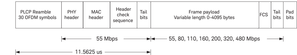
Figure 12. Frame structure for UWB-OFDM format.
