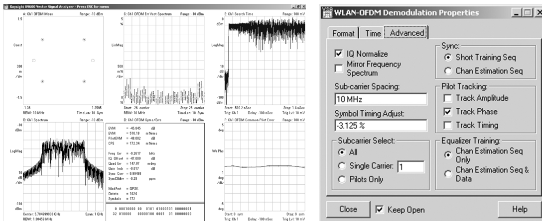
Figure 54. Measuring demod characteristics, including channel flatness, using a x32 time scaled 802.11a test waveform.
