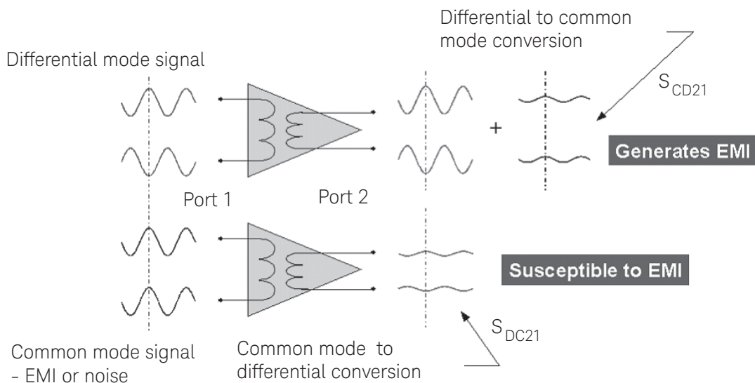
Figure 22. Terminology for signals that apply to a differential device. Signals referenced to each other are differential mode; signals referenced to ground are common mode. Some devices may convert to a single-ended, unbalanced, signal on the input or output.
