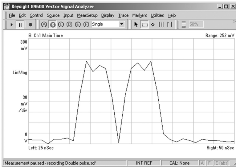
Figure 51. Demodulated double pulse
