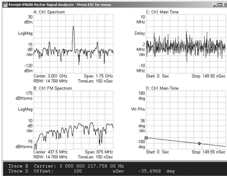
Figure 56. Using the FM demodulation in 89601.
