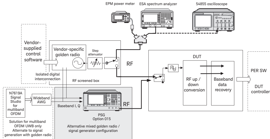
Figure 64. Golden radio receiver test configuration.
