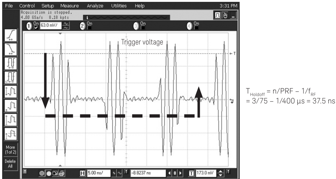
Figure 30. A 4 ns, 400 MHz pulsed waveform 75 MHz pulse repetition frequency (PRF) rate.
