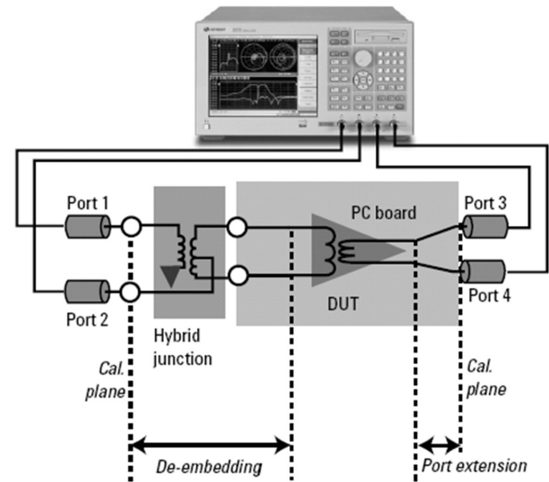
Figure 23. Basic configuration for device test using hybrid junction.
