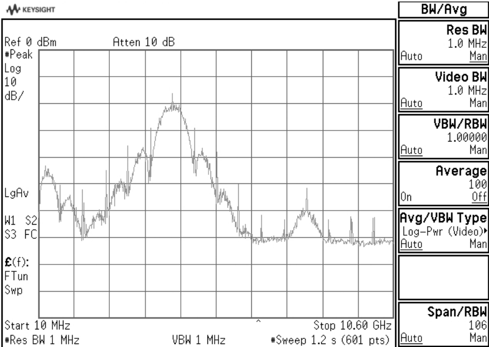
Figure 42. Mixed noise and spurious peak detection.
