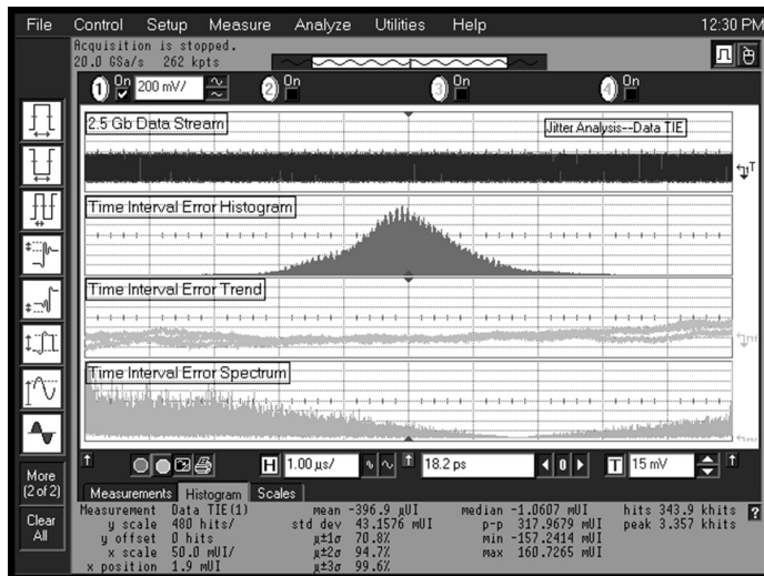
Figure 49a. Time domain jitter analysis.
