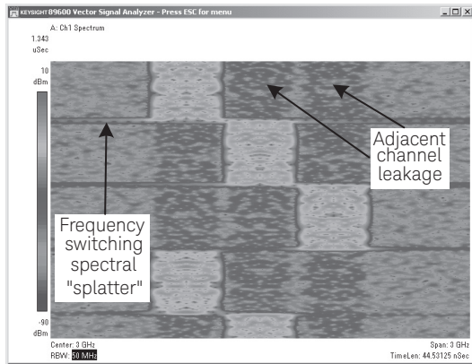
Figure 46. Spectrogram of MB-OFDM.
