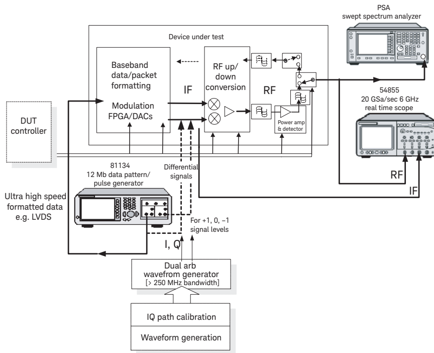
Figure 27. Transmitter test configuration for RF/analog circuitry.
