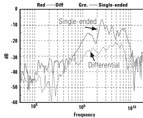
Figure 29b. CMRR of single-ended and differential probes.
