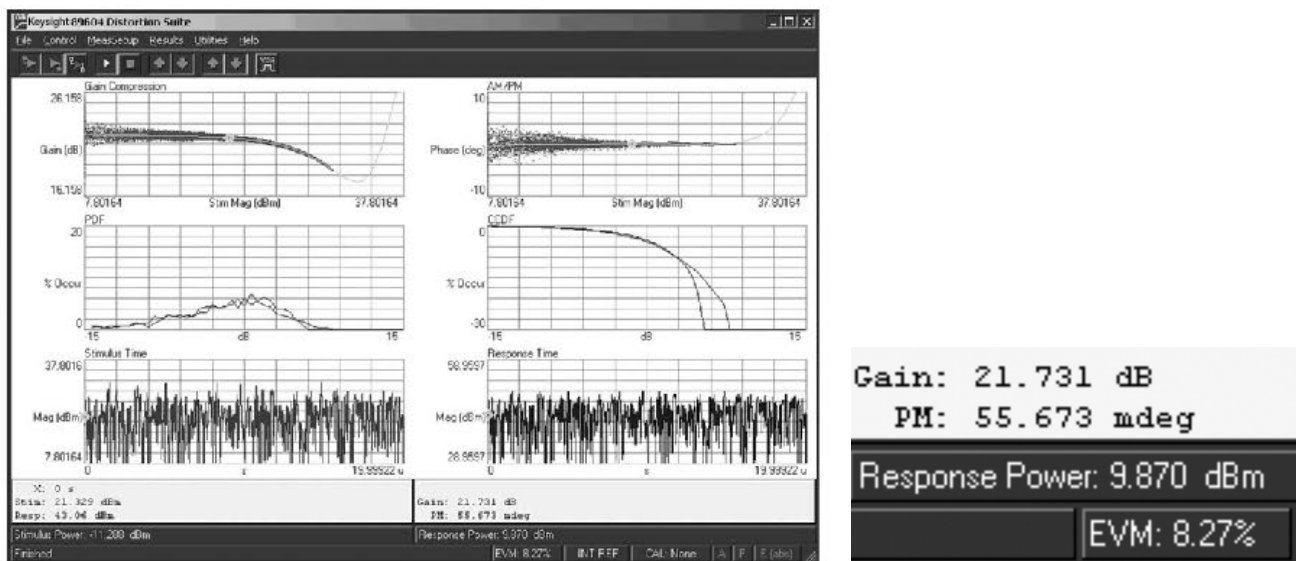
Figure 25. Sample plot from 89604 software using an 802.11 OFDM waveform as the test signal.
