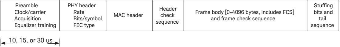
Figure 13. Frame structure for DS-UWB format.
