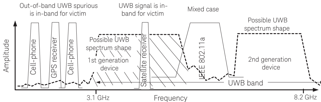
Figure 15. In-band versus out-of-band Interference for different victims.
