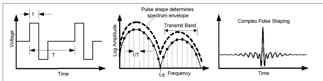
Figure 2. Time and spectrum plots for a bipolar pulse, and an example of a complex pulse with a more desirable spectrum shape.
