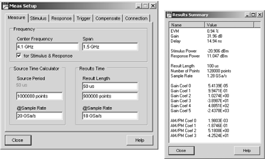
Figure 26. Example of configuration options and curve fitting results for 89604.
