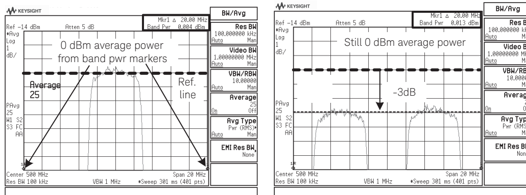
Figure 36a. A 5 MHz noise source on a 500 MHz carrier.
