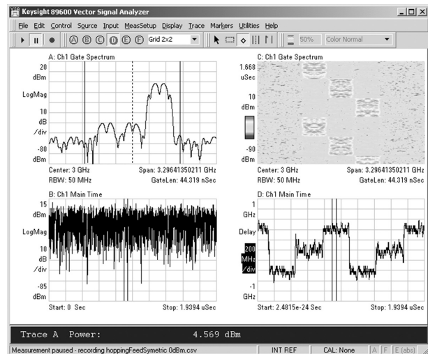
Figure 53b. Spectrum versus time of modulated OFDM signal.
