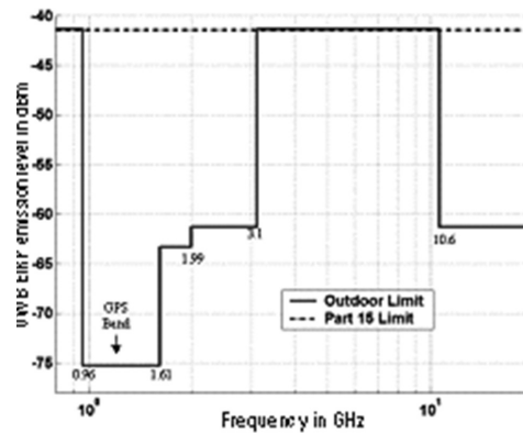
Figure 48b. Outdoor FCC spectrum mask.
