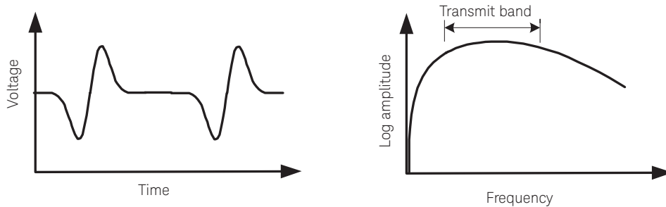
Figure 5. Time and spectrum plots of Gaussian mono-pulse, showing approximation to a carrier cycle.
