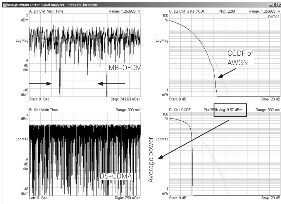
Figure 38. Peak power, average power, and CCDF of full bandwidth OFDM-like (top) and DS-UWB-like signal envelopes (bottom).
