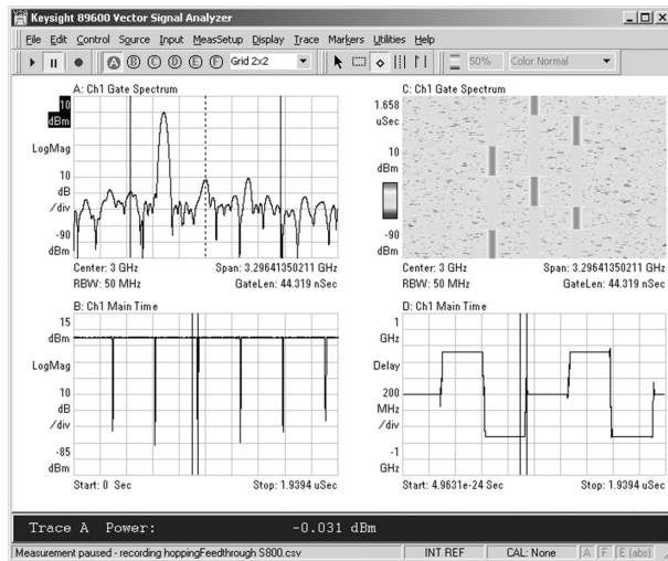
Figure 53a. Frequency versus time results for frequency-switched RF carrier.
