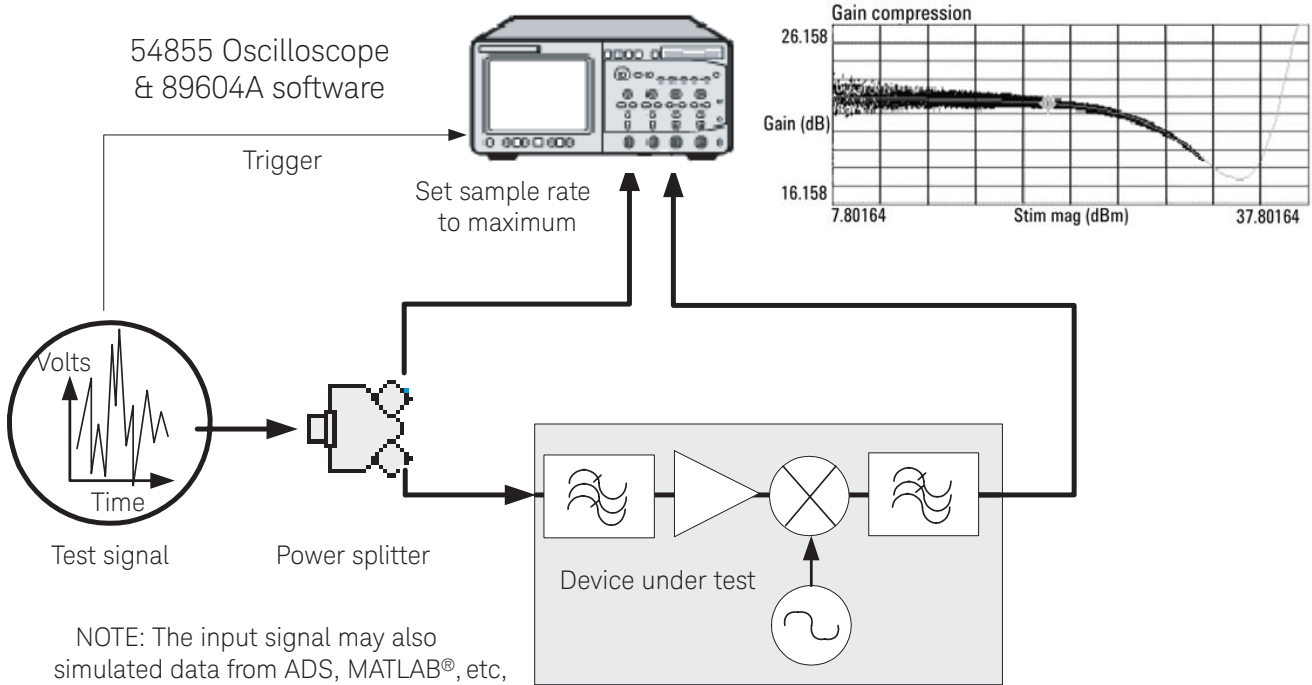
Figure 24. Test configuration for using 89604 distortion suite.
