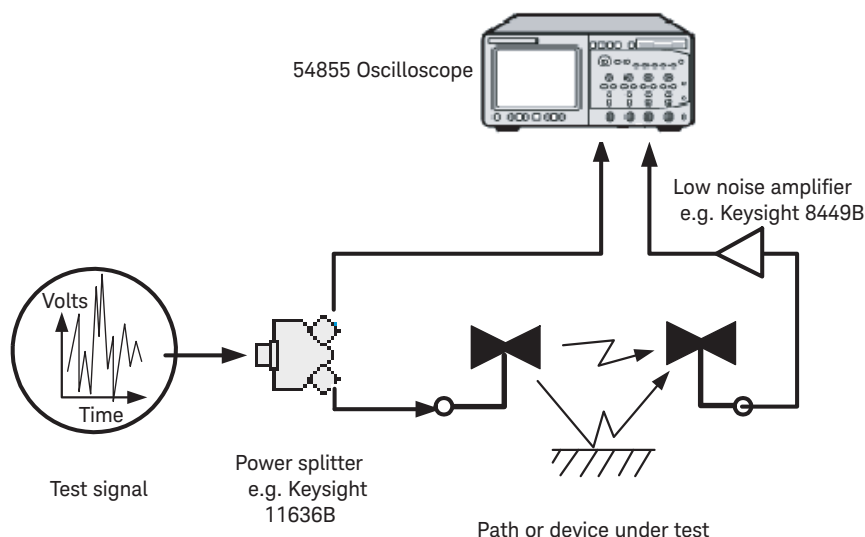
Figure 21. Using digitized signal for time correlation/coherence measurements.
