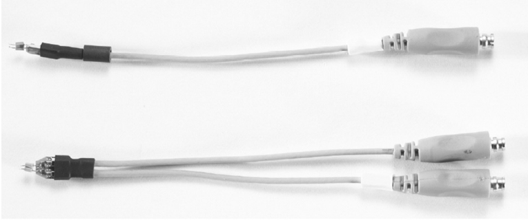
Figure 28. Photograph of 1134A single ended and differential probe heads.
