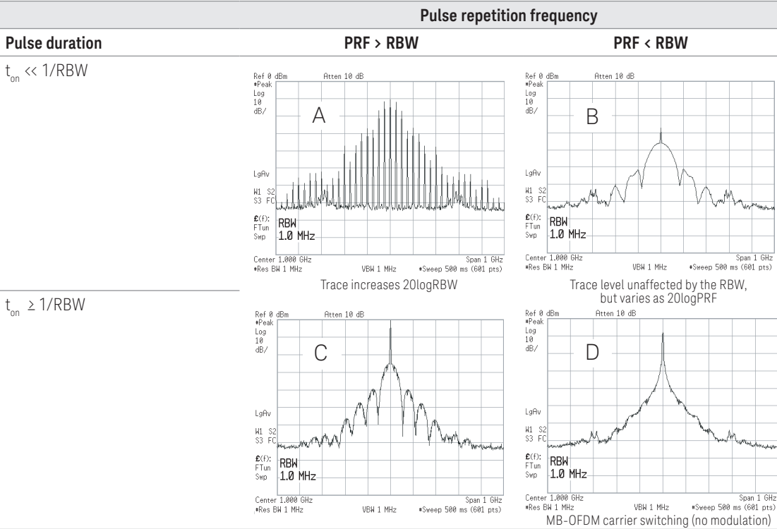
Figure 40. Swept spectrum peak detector response to pulse signals with various PRF and pulse duration. Note: These plots are for pulsed signals that do not have any modulation applied.
